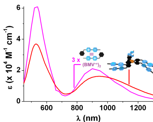
Figure 30. Electronic UV-Vis-NIR absorption spectra of \text{HV}_\text{D}^{6(\bullet+)} compared to that of (\text{BMV}^{\bullet+})_2 in water. Solvent: water buffered at pH 7.0 with 0.1 M \text{Na}_2\text{HPO}_4/\text{NaH}_2\text{PO}_4 . T = 25.0(1)^\circ\text{C} .
