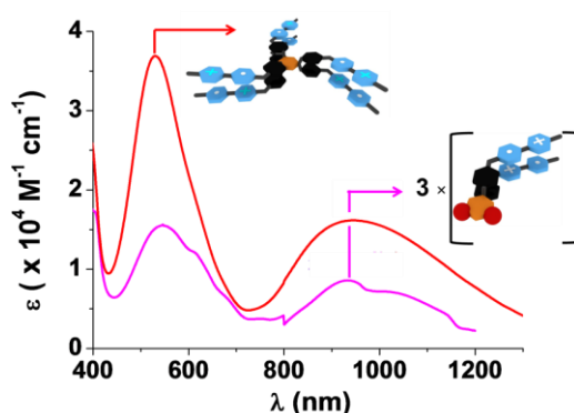
Figure 31. Electronic UV-Vis-NIR absorption spectra of \text{HV}_\text{D}^{6(\bullet+)} compared to that of (\text{BV}^{\bullet+})_2 in water. Solvent: water buffered at pH 7.0 with 0.1 M \text{Na}_2\text{HPO}_4/\text{NaH}_2\text{PO}_4 . T = 25.0(1)^\circ\text{C} .
