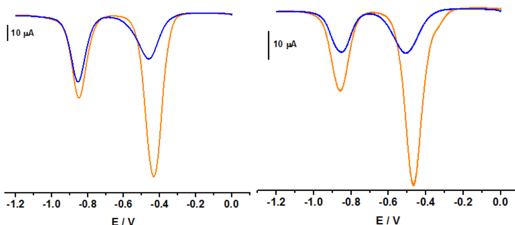
Figure 54. Square Wave voltammograms of \text{C23}^{4+} , [\text{C23}^{4+}] = 0.05 \text{ mM} (left) and \text{C24}^{4+} , [\text{C24}^{4+}] = 0.05 \text{ mM} (right) in the absence (orange line) and the presence of \text{CB}[7] (blue line, respectively 3 and 4 equivalents of \text{CB}[7] ). All voltammograms were recorded in Argon-purged phosphate buffer solutions (pH 7) at 298 K ( E versus \text{Ag}/\text{AgCl} ).
