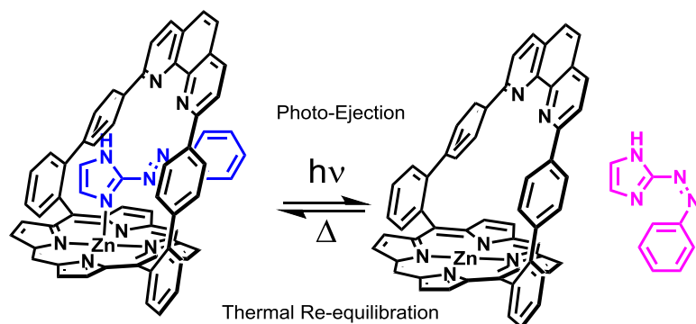
Figure 18. Schematic representation of the principle of photo-ejection of the azo-aryl-imidazole from the pentacoordinated species with \text{ZnL}^1 .
