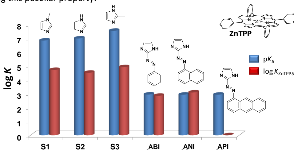
Figure 13. Schematic representation of the \log K_{\text{ZnTPP,S}} values as a function of the pK a sequence (simulated with ChemAxon pK a calculator) which demonstrate the steric effects induced by the bulkiness of the azo-chromophore substituents.
