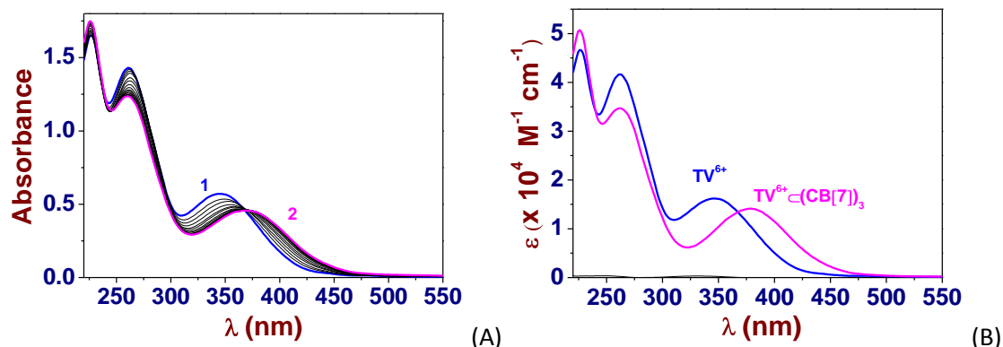
Figure 7. A) UV-Vis. absorption titration of TV 6+ by CB [7]. B) Electronic spectra of TV 6+ and its inclusion complex with CB [7] ( TV 6+ ⊂ ( CB [7]) 3 ). Solvent: water pH 7.0 (0.1 M Na 2 H 2 PO 4 /NaH 2 PO 4 ). [ TV 6+ ] 0 = 10 -4 M; (1) [ CB [7]] 0 /[ TV 6+ ] 0 = 0; (2) [ CB [7]] 0 /[ TV 6+ ] 0 = 9.3; l = 1 cm; T = 25.0(1)°C. The absorption spectra are not corrected from dilution effects.
