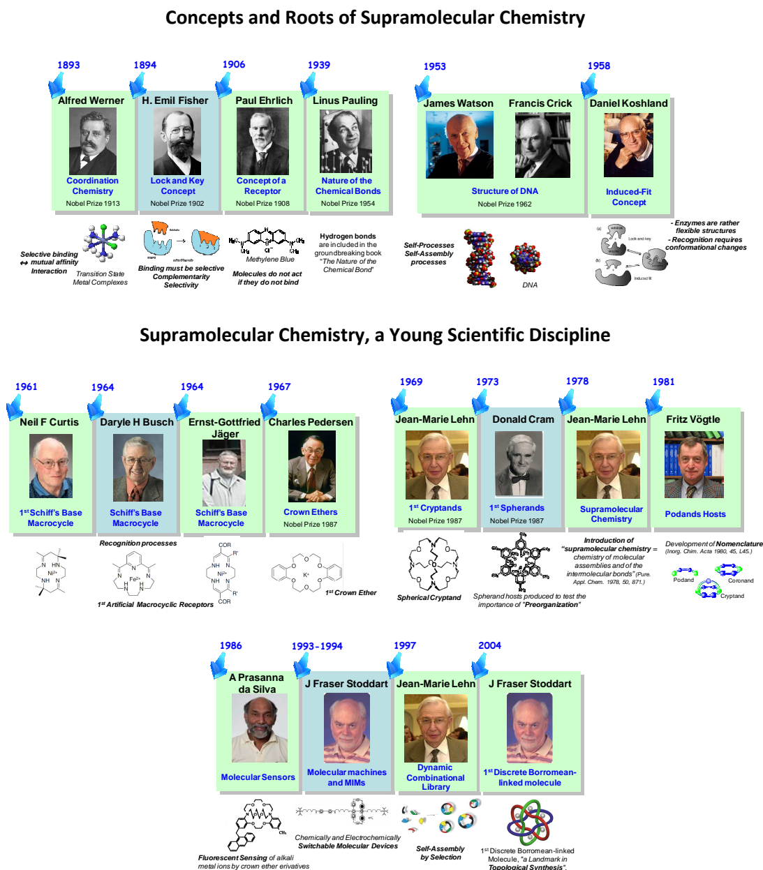
Figure 1. Timeline of supramolecular chemistry
