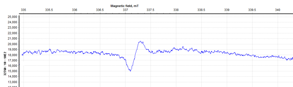
Figure 43. EPR spectra measured for (top) \text{C23}^{2(•+)} and (bottom) \text{C23}^{2(•+)} and 4 equivalents of CB[7] . Solvent: water.
