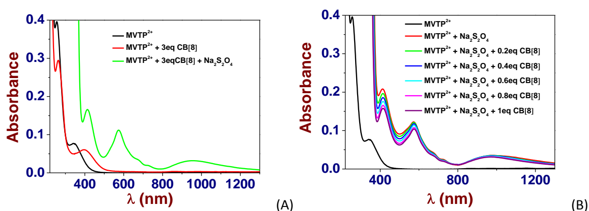
Figure 32. (A) UV-Vis.-NIR spectra of \text{MVTP}^{2+} ( [\text{MVTP}^{2+}]_0 = 2.0 \times 10^{-5} M, black line) and of its \text{MVTP}^{2+} \subset \text{CB}[8] complex ( [\text{CB}[8]]_0 / \text{MVTP}^{2+} = 3 , red line). Addition of a freshly prepared \text{O}_2 -free sodium dithionite (green line) induces formation of absorptions in the visible and NIR regions that are characteristics of the stable radical dimeric species (\text{MVTP}^{\bullet+})_2 , see Figure 28 for comparison propose with \text{CB}[7] ). (B) UV-Vis.-NIR spectra of \text{MVTP}^{2+} ( [\text{MVTP}^{2+}]_0 = 2.0 \times 10^{-5} M, black line) and of its radical species \text{MVTP}^{\bullet+} under its predominant dimeric state (red line, addition of freshly prepared \text{O}_2 -free sodium dithionite). Upon addition of \text{CB}[8] ( [\text{CB}[8]]_0 / [\text{MVTP}^{\bullet+}]_0 = 0 , red line and [\text{CB}[7]]_0 / [\text{MVTP}^{\bullet+}]_0 = 1 , purple line), weak variations of the absorption spectrum of (\text{MVTP}^{\bullet+})_2 are observed. Solvent: water buffered at pH 7.0 with 0.1 M \text{Na}_2\text{H}_2\text{PO}_4 / \text{NaH}_2\text{PO}_4 ; l = 1 cm; T = 25.0(1)^\circ \text{C} . In each of the solutions considered, the \text{MVTP}^{\bullet+} species was generated from \text{MVTP}^{2+} using freshly prepared sodium dithionite solution at ca. 10^{-2} under \text{O}_2 free conditions. The absorption spectra are not corrected from dilution effects.
