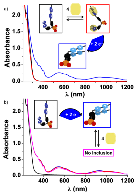
Figure 21. (a) UV-Vis-NIR spectra of \text{BV}^{4+} ( [\text{BV}^{4+}]_0 = 5.3 \times 10^{-5} M, black line) and of its \text{BV}^{4+}(\text{CB}[7])_2 complex ( [\text{BV}^{4+}]_0 = 5.3 \times 10^{-5} M and [\text{CB}[7]]_0 = 2.12 \times 10^{-4} M, red line). (b) UV-Vis-NIR spectra of \text{BV}^{4+} ( [\text{BV}^{4+}]_0 = 5.3 \times 10^{-5} M, black line) and of its radical analogue \text{BV}^{2(\bullet+)} (blue line, addition of freshly prepared and \text{O}_2 -free sodium dithionite), and upon addition of \text{CB}[7] ( [\text{CB}[7]]_0 = 5.3 \times 10^{-5} M, red line and [\text{CB}[7]]_0 = 2.12 \times 10^{-4} M, pink line). Solvent: water buffered at pH 7.0 with 0.1 M \text{Na}_2\text{HPO}_4/\text{NaH}_2\text{PO}_4 ; l = 1 cm; T = 25.0(1)^\circ\text{C} . In each of the solutions considered, the \text{BV}^{2(\bullet+)} species was generated from \text{BV}^{4+} using freshly prepared sodium dithionite solution at ca. 10^{-2} M under \text{O}_2 free conditions.
