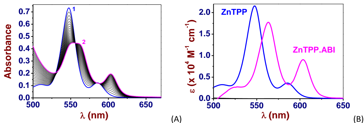
Figure 2. (A) UV-Vis. absorption spectrophotometric titration of ZnTPP by azo-benzene-imidazole ( ABI ). Solvent: 1,2-dichloroethane; T = 25.0(2) \text{ }^\circ\text{C} ; l = 1 \text{ cm} . (1) [\text{ZnTPP}]_0 = 3.4 \times 10^{-5} \text{ M} ; (2) [\text{ABI}]_0/[\text{ZnTPP}]_0 = 131 . (B) Electronic spectra of ZnTPP and its pentacoordinated species with ABI .
