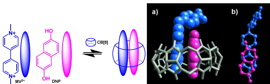
Figure 11. Schematic representation of the host-guest complex involving CT interactions and X-ray crystal structure (a) MV 2+ •DNP • CB[8] and (b) MV 2+ •DNP . Figure (right) taken from ref. 70 (Kim et al. 2001).
