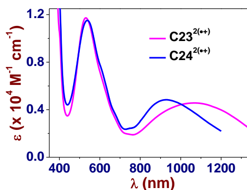
Figure 51. Electronic UV-Vis.-NIR absorption spectra of C23 2(•+) and C24 2(•+) in water. Solvent: water buffered at pH 7.0 with 0.1 M Na 2 HPO 4 /NaH 2 PO 4 . T = 25.0(1)^\circ\text{C} .
