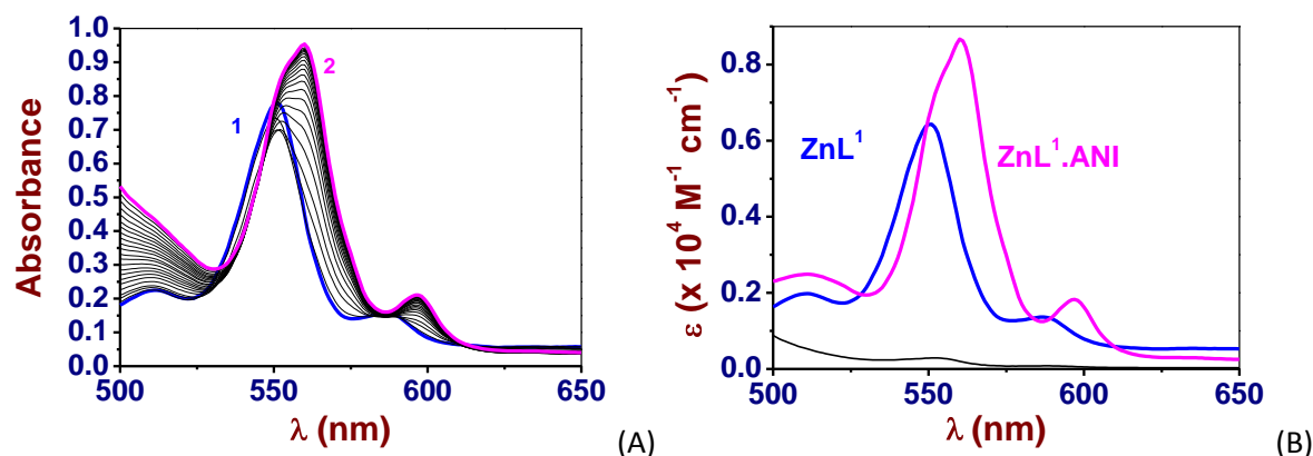
Figure 6. (A) UV-Vis. absorption spectrophotometric titration of \text{ZnL}^1 by azo-naphthyl-imidazole ( ANI ). Solvent: 1,2-dichloroethane; T = 25.0(2)^\circ\text{C} ; l = 1\text{ cm} . (1) [\text{ZnL}^1]_0 = 4.80 \times 10^{-6}\text{ M} ; (2) [\text{ANI}]_0/[\text{ZnL}^1]_0 = 3.97 . (B) Electronic spectra of the \text{ZnL}^1 receptor and its pentacoordinated species with ANI .
