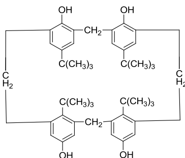
Figure 3. First cyclic condensate from p -alkylphenol/CH 2 O based on the Zinke and Ziegler synthesis. 17
