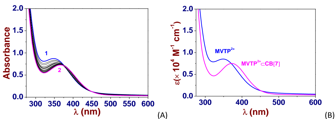
Figure 6. A) UV-Vis. absorption titration of \text{MVTP}^{2+} by \text{CB}[7] . B) Electronic spectra of \text{MVTP}^{2+} and its inclusion complex with \text{CB}[7] ( \text{MVTP}^{2+} \subset \text{CB}[7] ). Solvent: water pH 7.0 (0.1 M \text{Na}_2\text{H}_2\text{PO}_4/\text{NaH}_2\text{PO}_4 ). [\text{MVTP}^{2+}]_0 = 10^{-4} \text{ M} ; (1) [\text{CB}[7]]_0/[\text{MVTP}^{2+}]_0 = 0 ; (2) [\text{CB}[7]]_0/[\text{MVTP}^{2+}]_0 = 2.62 ; l = 1 \text{ cm} ; T = 25.0(1)^\circ\text{C} . The absorption spectra are not corrected from dilution effects.
