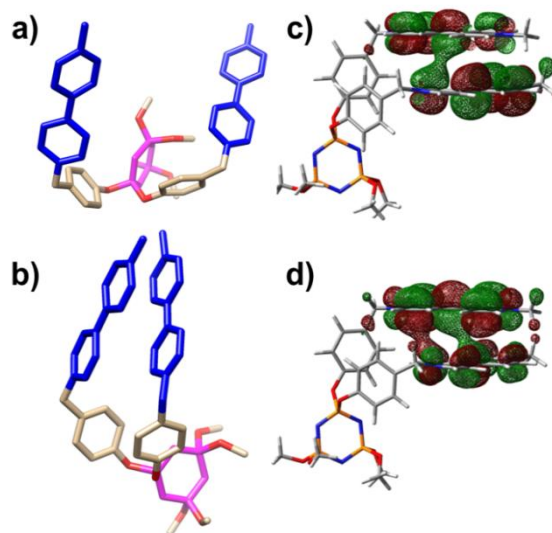
Figure 32. Optimized geometries of the BV 4+ a) and BV 2(•+) b) models, and representations of SOMO c) and SOMO-1 d) in BV 2(•+) computed in aqueous solution at the M06/6-31G(d,p) level.
