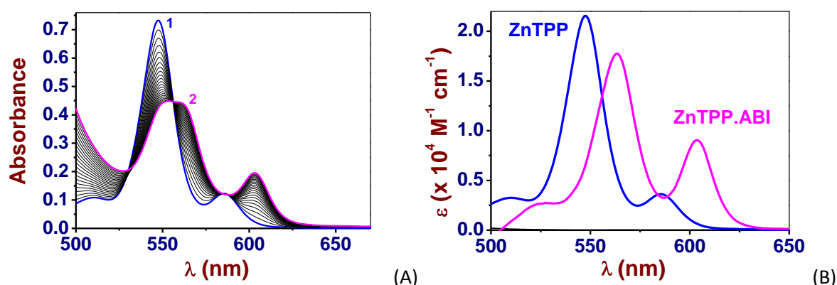
Figure 2. (A) UV-Vis. absorption spectrophotometric titration of ZnTPP by azo-benzene-imidazole ( ABI ). Solvent: 1,2-dichloroethane; T = 25.0(2)^\circ\text{C} ; l = 1\text{ cm} . (1) [\text{ZnTPP}]_0 = 3.4 \times 10^{-5}\text{ M} ; (2) [\text{ABI}]_0/[\text{ZnTPP}]_0 = 131 . (B) Electronic spectra of ZnTPP and its pentacoordinated species with ABI .
