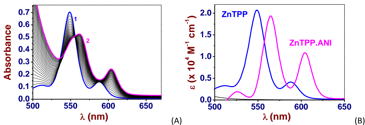
Figure 3. (A) UV-Vis. absorption spectrophotometric titration of ZnTPP by azo-naphthyl-imidazole ( ANI ). Solvent: 1,2-dichloroethane; T = 25.0(2)^\circ\text{C} ; l = 1\text{ cm} . (1) [\text{ZnTPP}]_0 = 3.4 \times 10^{-5}\text{ M} ; (2) [\text{ANI}]_0/[\text{ZnTPP}]_0 = 82 . (B) Electronic spectra of ZnTPP and its pentacoordinated species with ANI .
