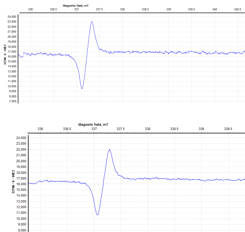
Figure 44. EPR spectra measured for (top) \text{C24}^{2(•+)} and (bottom) \text{C24}^{2(•+)} and 4 equivalents of CB[7] . Solvent: water.
