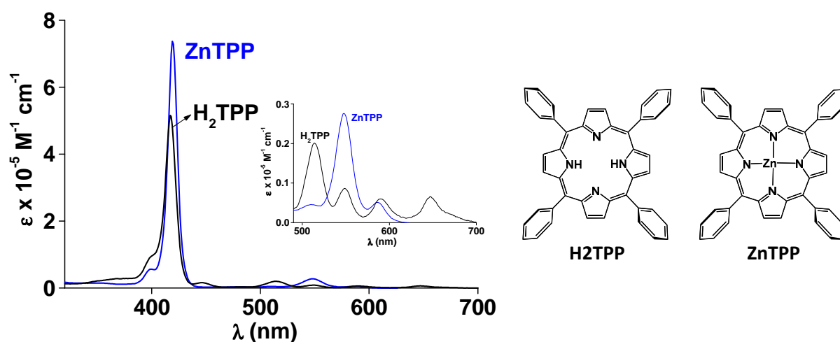
Figure 24. Electronic spectra H 2 TPP and ZnTPP . Solvent: 1,2-dichloroethane; T = 25.0^\circ \text{C} .
