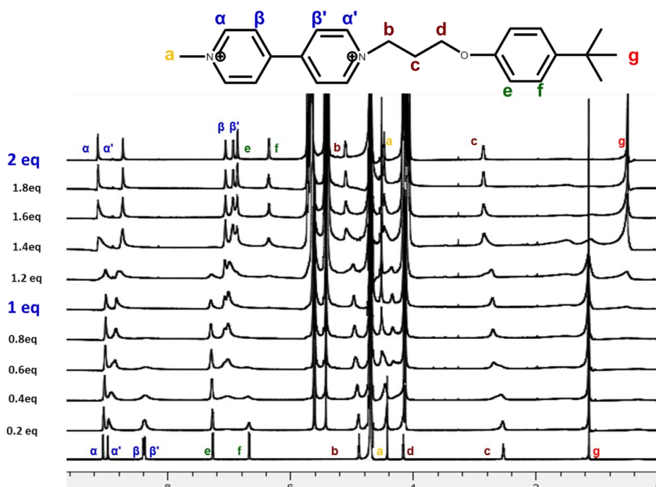
Figure 28. ^1\text{H} NMR spectra (600 MHz, \text{D}_2\text{O} , 298 K) of \text{MC3}^{2+} (3.5 mM) in the presence of increasing amounts of CB[7] .
