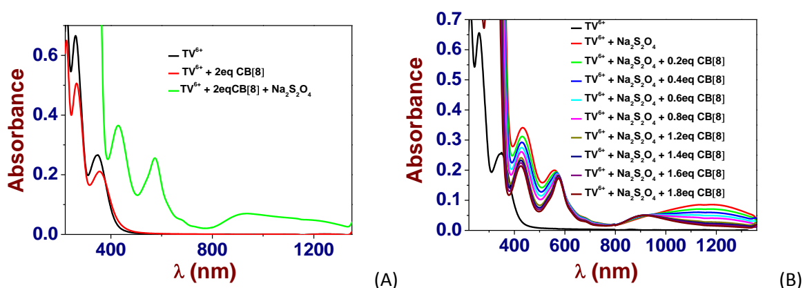
Figure 33. (A) UV-Vis.-NIR spectra of \text{TV}^{6+} ( [\text{TV}^{6+}]_0 = 2.0 \times 10^{-5} \text{ M} , black line) and of its \text{TV}^{6+} \subset (\text{CB}[8])_3 complex ( [\text{CB}[8]]_0/[\text{TV}^{6+}]_0 = 2 , red line). Addition of a fresh \text{O}_2 -free sodium dithionite (green line) induces formation of absorptions in the visible and NIR regions that are characteristics of the stable radical dimeric species (\text{TV}^{3(\bullet+)})_2 , see Figure 29 for comparison propose with \text{CB}[7] ). The NIR absorption however displays a broader shape with respect to that measured in the absence of \text{CB}[7] or \text{CB}[8] . (B) UV-Vis.-NIR spectra of \text{TV}^{6+} ( [\text{TV}^{6+}]_0 = 2.0 \times 10^{-5} \text{ M} , black line) and of its triradical species \text{TV}^{3(\bullet+)} under its predominant dimeric state (red line, addition of freshly prepared \text{O}_2 -free sodium dithionite). Upon addition of \text{CB}[8] ( [\text{CB}[8]]_0/[\text{TV}^{3(\bullet+)}]_0 = 0 , red line and [\text{CB}[8]]_0/[\text{TV}^{3(\bullet+)}]_0 = 1.8 , wine line), large spectral variations of the absorption spectrum of (\text{TV}^{3(\bullet+)})_2 are observed indicating host-guest complexation with \text{CB}[8] . In addition to this feature, no precipitation of oligomeric species (\text{TV}^{3(\bullet+)})_n occurs. Solvent: water buffered at pH 7.0 with 0.1 M \text{Na}_2\text{H}_2\text{PO}_4/\text{NaH}_2\text{PO}_4 ; l = 1 \text{ cm} ; T = 25.0(1)^\circ \text{ C} . In each of the solutions considered, the \text{MVT}^{2+} species was generated from \text{MVT}^{2+} using freshly prepared sodium dithionite solution at ca. 10^{-2} under \text{O}_2 free conditions. The absorption spectra are not corrected from dilution effects.
