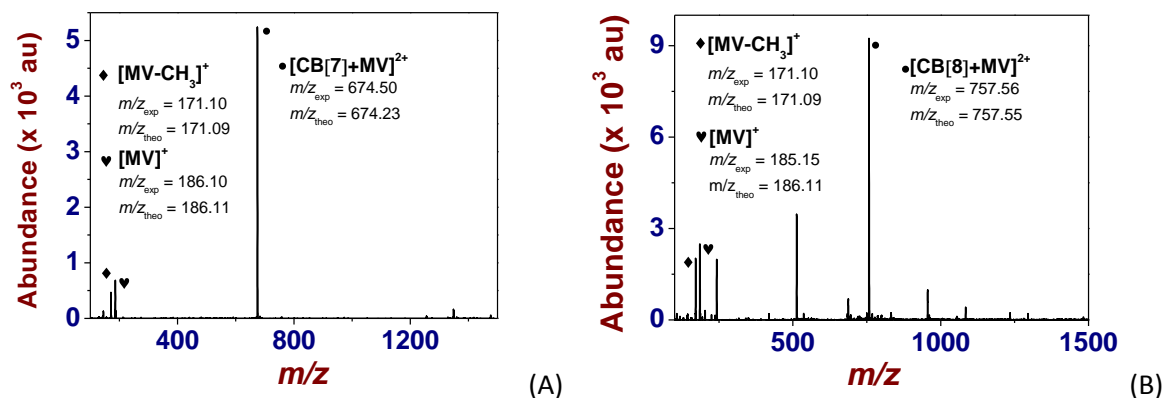
Figure 14. ESI mass spectra of the MV 2+ complex formed with (A) CB[7] and (B) CB[8] . (A) [MV^{2+}]_0 = 55 \mu\text{M} with 1 equivalent of CB[7] ; V_c = 300 \text{ V} . (B) [MV^{2+}]_0 = 100 \mu\text{M} with 1 equivalent of CB[8] . V_c = 150 \text{ V} . Solvent: water; positive mode.
