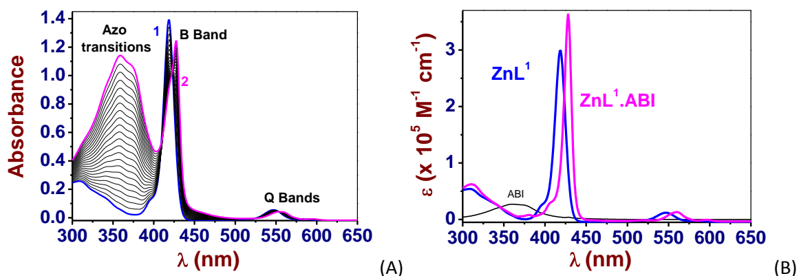
Figure 5. (A) UV-Vis. absorption spectrophotometric titration of \text{ZnL}^1 by azo-benzene-imidazole ( ABI ). Solvent: 1,2-dichloroethane; T = 25.0(2)^\circ\text{C} ; l = 1\text{ cm} . (1) [\text{ZnL}^1]_0 = 4.69 \times 10^{-6}\text{ M} ; (2) [\text{ABI}]_0/[\text{ZnL}^1]_0 = 35.18 . (B) Electronic spectra of the \text{ZnL}^1 receptor and its pentacoordinated species with ABI .
