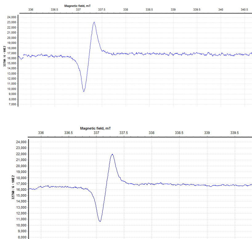
Figure 44. EPR spectra measured for (top) \text{C24}^{2(\bullet+)} and (bottom) \text{C24}^{2(\bullet+)} and 4 equivalents of CB[7] . Solvent: water.
