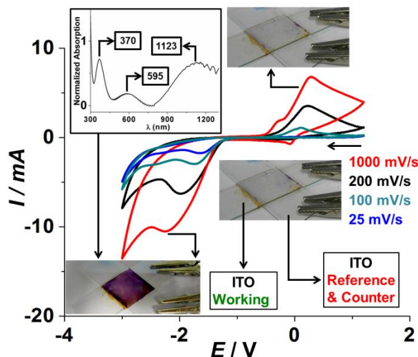
Figure 33. Variable scan cyclic voltammograms of a solution of \text{HV}^{12+} \bullet 12\text{Cl}^- in 1 M NaCl \text{H}_2\text{O} , sandwiched between two ITO coated glass slides (4-8 Ohms, 1500–2000 Å nominal coating thickness). One of the ITO slides is used as a working electrode while the other is used as counter and reference electrode. A colour change (colourless to purple) is observed upon reduction. Inset: UV-Vis-NIR spectrum of the device switched at –2 V.
