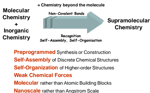
Figure 2. Key aspects of supramolecular chemistry
