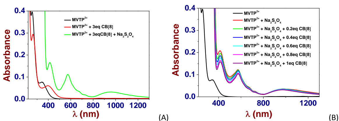
Figure 32. (A) UV-Vis.-NIR spectra of MVTP^{2+} ( [MVTP^{2+}]_0 = 2.0 \times 10^{-5} M, black line) and of its MVTP^{2+} \subset CB[8] complex ( [CB[8]]_0/[MVTP^{2+}] = 3 , red line). Addition of a freshly prepared O_2 -free sodium dithionite (green line) induces formation of absorptions in the visible and NIR regions that are characteristics of the stable radical dimeric species (MVTP^{\bullet\bullet})_2 , see Figure 28 for comparison propose with CB[7] . (B) UV-Vis.-NIR spectra of MVTP^{2+} ( [MVTP^{2+}]_0 = 2.0 \times 10^{-5} M, black line) and of its radical species MVTP^{\bullet\bullet} under its predominant dimeric state (red line, addition of freshly prepared O_2 -free sodium dithionite). Upon addition of CB[8] ( [CB[8]]_0/[MVTP^{\bullet\bullet}]_0 = 0 , red line and [CB[7]]_0/[MVTP^{\bullet\bullet}]_0 = 1 , purple line), weak variations of the absorption spectrum of (MVTP^{\bullet\bullet})_2 are observed. Solvent: water buffered at pH 7.0 with 0.1 M Na_2H_2PO_4/NaH_2PO_4 ; l = 1 cm; T = 25.0(1)^\circ\text{C} . In each of the solutions considered, the MVTP^{\bullet\bullet} species was generated from MVTP^{2+} using freshly prepared sodium dithionite solution at ca. 10^{-2} under O_2 free conditions. The absorption spectra are not corrected from dilution effects.
