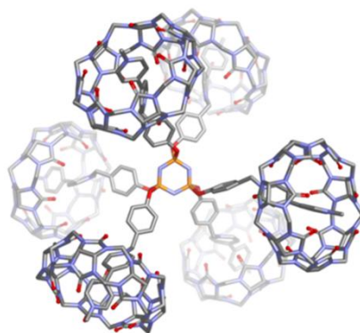
Figure 27. Capped-Stick representation of the minimum energy geometry of \text{HV}^{12+} \subset (\text{CB}[7])_6 obtained with PM6 calculations.
