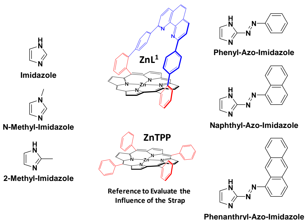
Figure 30. Chemical structures of the Zn(II) metalloporphyrins and imidazole substrates examined on this work.
