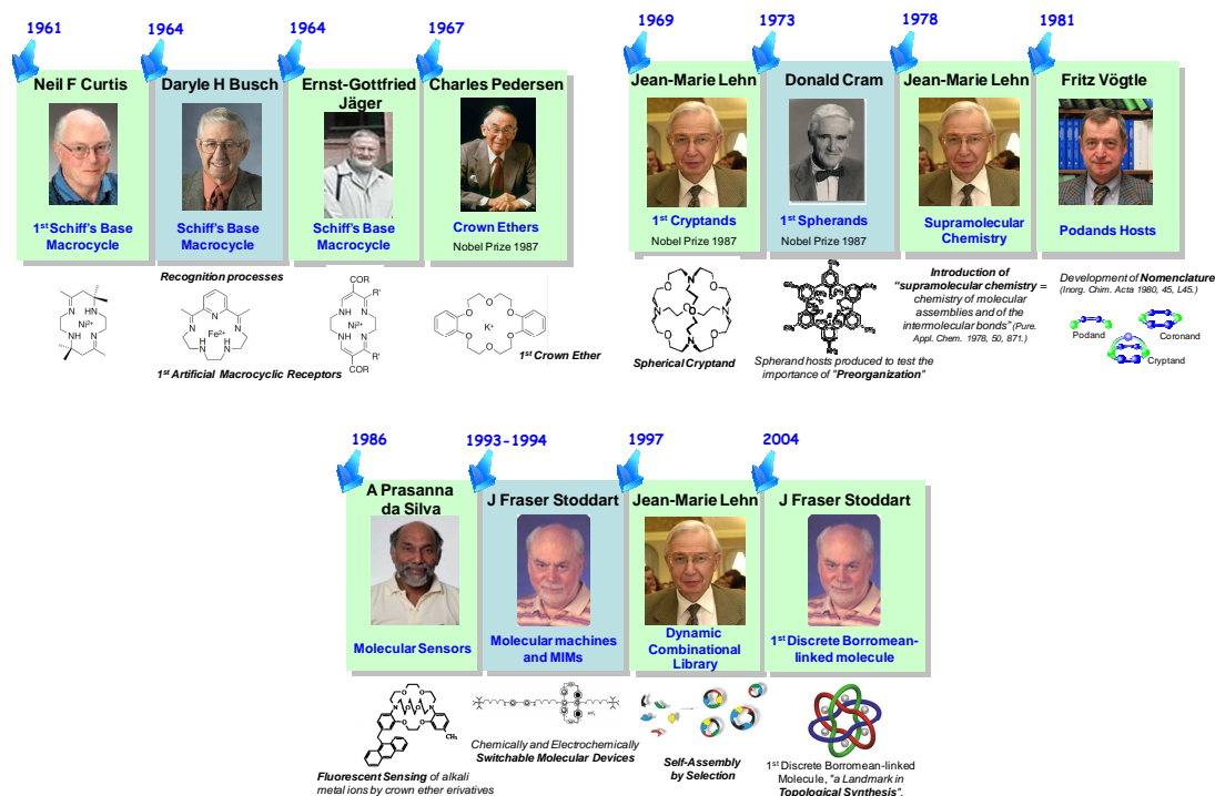
Figure 1. Timeline of supramolecular chemistry
