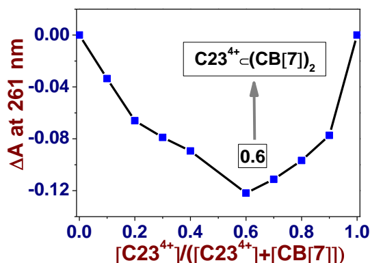
Figure 22. Job plot ( \Delta A at 261 nm) upon mixing C23^{4+} with CB[7] at pH 7. ( [C23^{2+}]_0 + [CB[7]]_0 ) = 6.9 \times 10^{-5} M; Solvent :water pH 7.0 (0.1 M Na_2H_2PO_4/NaH_2PO_4 ); l = 1 cm; T = 25.0(1)^\circ C .
