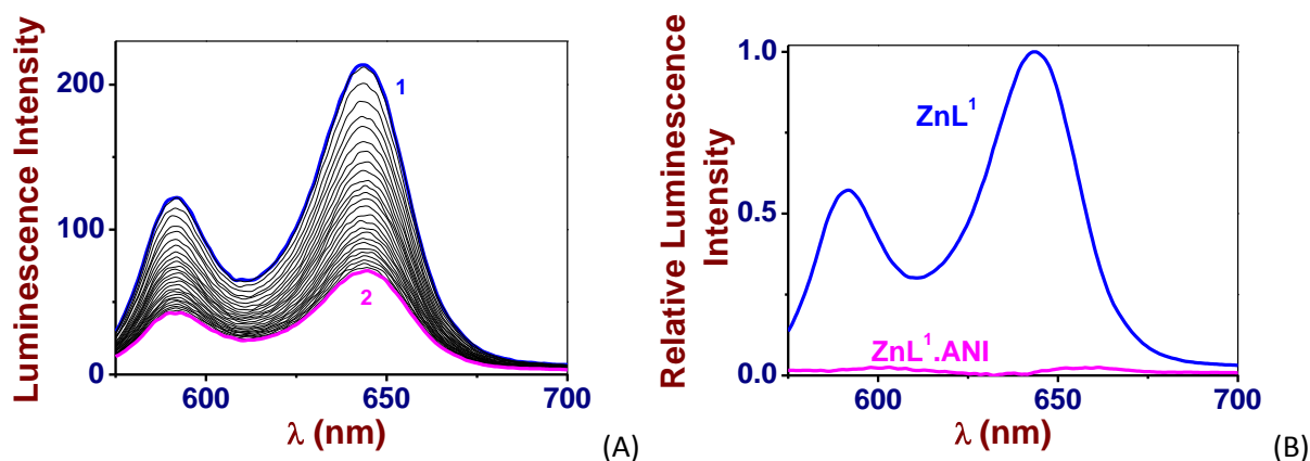
Figure 11. (A) Spectrofluorimetric titration of ZnL 1 receptor by azo-naphthyl-imidazole ( ANI ). \lambda_{\text{exc}} = 555 nm; exc. and em. slits 10/10 nm; (1) [\text{ZnL}^1]_{\text{tot}} = 1.20 \times 10^{-5} M; (2) [\text{ANI}]_0/[\text{ZnL}^1]_{\text{tot}} = 58.3 . (B) Relative reconstituted emission spectra of ZnL 1 and its pentacoordinated complex with ANI .
