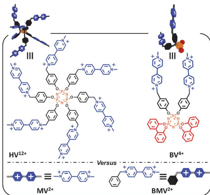
Figure 1. Structural formulas and 3D representations of phosphazene derivatives bearing six 4,4'-bipyridinium subunits ( HV 12+ ) and two 4,4'-bipyridinium subunits and two [1,1'-biphenyl]-2,2'-diol protective groups ( BV 4+ ).
