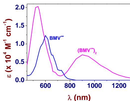
Figure 17. UV-Vis.-NIR electronic spectra of BMV •+ under its monomeric or dimeric form. Solvent: Water pH 7.0 (0.1 M \text{Na}_2\text{HPO}_4/\text{NaH}_2\text{PO}_4 ); T = 25.0(1)^\circ\text{C} .
