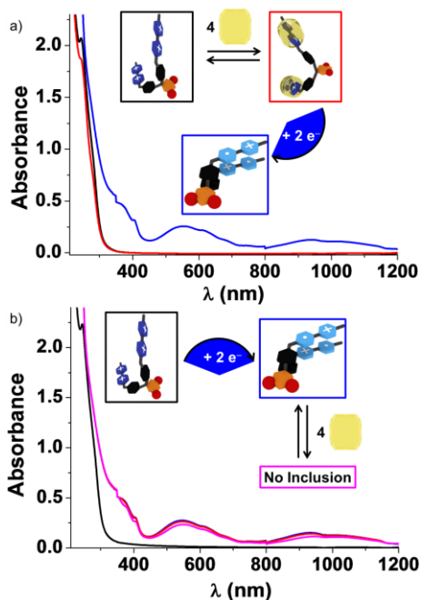
Figure 21. (a) UV-Vis-NIR spectra of BV^{4+} ( [BV^{4+}]_0 = 5.3 \times 10^{-5} M, black line) and of its BV^{4+} \subset (CB[7])_2 complex ( [BV^{4+}]_0 = 5.3 \times 10^{-5} M and [CB[7]]_0 = 2.12 \times 10^{-4} M, red line). (b) UV-Vis-NIR spectra of BV^{4+} ( [BV^{4+}]_0 = 5.3 \times 10^{-5} M, black line) and of its radical analogue BV^{2(\bullet+)} (blue line, addition of freshly prepared and O_2 -free sodium dithionite), and upon addition of CB[7] ( [CB[7]]_0 = 5.3 \times 10^{-5} M, red line and [CB[7]]_0 = 2.12 \times 10^{-4} M, pink line). Solvent: water buffered at pH 7.0 with 0.1 M Na_2HPO_4/NaH_2PO_4 ; l = 1 cm; T = 25.0(1) °C. In each of the solutions considered, the BV^{2(\bullet+)} species was generated from BV^{4+} using freshly prepared sodium dithionite solution at ca. 10^{-2} M under O_2 free conditions.
