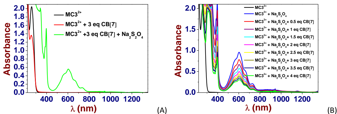
Figure 34. (A) UV-Vis.-NIR spectra of \text{MC3}^{2+} ( [\text{MC3}^{2+}]_0 = 10^{-4} M, black line) and of its \text{MC3}^{2+}\text{CB[7]} complex ( [\text{CB[7]}]_0/[\text{MC3}^{2+}]_0 = 3 , red line). Addition of a freshly prepared \text{O}_2 -free sodium dithionite (green line) induces formation of absorptions in the Vis. region that are characteristics of the radical species \text{MC3}^{\bullet+} . (B) UV-Vis.-NIR spectra of \text{MC3}^{2+} ( [\text{MC3}^{2+}]_0 = 10^{-4} M, black line) and of its radical species \text{MC3}^{\bullet+} (blue line, addition of freshly prepared and \text{O}_2 -free sodium dithionite). Upon addition of \text{CB[7]} ( [\text{CB[7]}]_0/[\text{MC3}^{\bullet+}]_0 = 0 , blue line and [\text{CB[7]}]_0/[\text{MC3}^{\bullet+}]_0 = 4 , green line), the Vis. absorptions experienced a significant hypochromic shift that is indicative of host/guest complexation. Solvent: water buffered at pH 7.0 with 0.1 M \text{Na}_2\text{H}_2\text{PO}_4/\text{NaH}_2\text{PO}_4 ; l = 1 cm; T = 25.0(1)^\circ\text{C} . In each of the solutions considered, the \text{MC3}^{\bullet+} species was generated from \text{MC3}^{2+} using freshly prepared sodium dithionite solution at ca. 10^{-2} under \text{O}_2 free conditions. The absorption spectra are not corrected from dilution effects.
