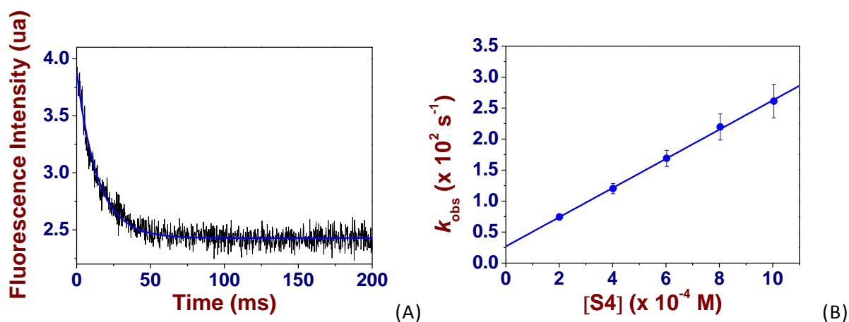
Figure 12. (A) Variation of the luminescence intensity versus time for the formation of \text{ZnL}^1\text{ABI} complex. Solvent: 1,2-dichloroethane; T = 25.0(2)^\circ\text{C} ; l = 1 \text{ cm} ; [\text{ZnL}^1] = 1.07 \times 10^{-5} \text{ M} ; [\text{ABI}]_0/[\text{ZnL}^1]_0 = 10.43 . \lambda_{\text{exc}} = 554 \text{ nm} ; set of band pass filter ( \lambda > 550 \text{ nm} ). (B) Variation of the pseudo-first order constants k_{\text{obs}} ( \text{s}^{-1} ) for the formation of \text{ZnL}^1\text{ABI} complex versus [\text{ABI}]_{\text{tot}} . Solvent: 1,2-dichloroethane; T = 25.0(2)^\circ\text{C} ; [\text{ZnL}^1] = 1.07 \times 10^{-5} \text{ M} .
