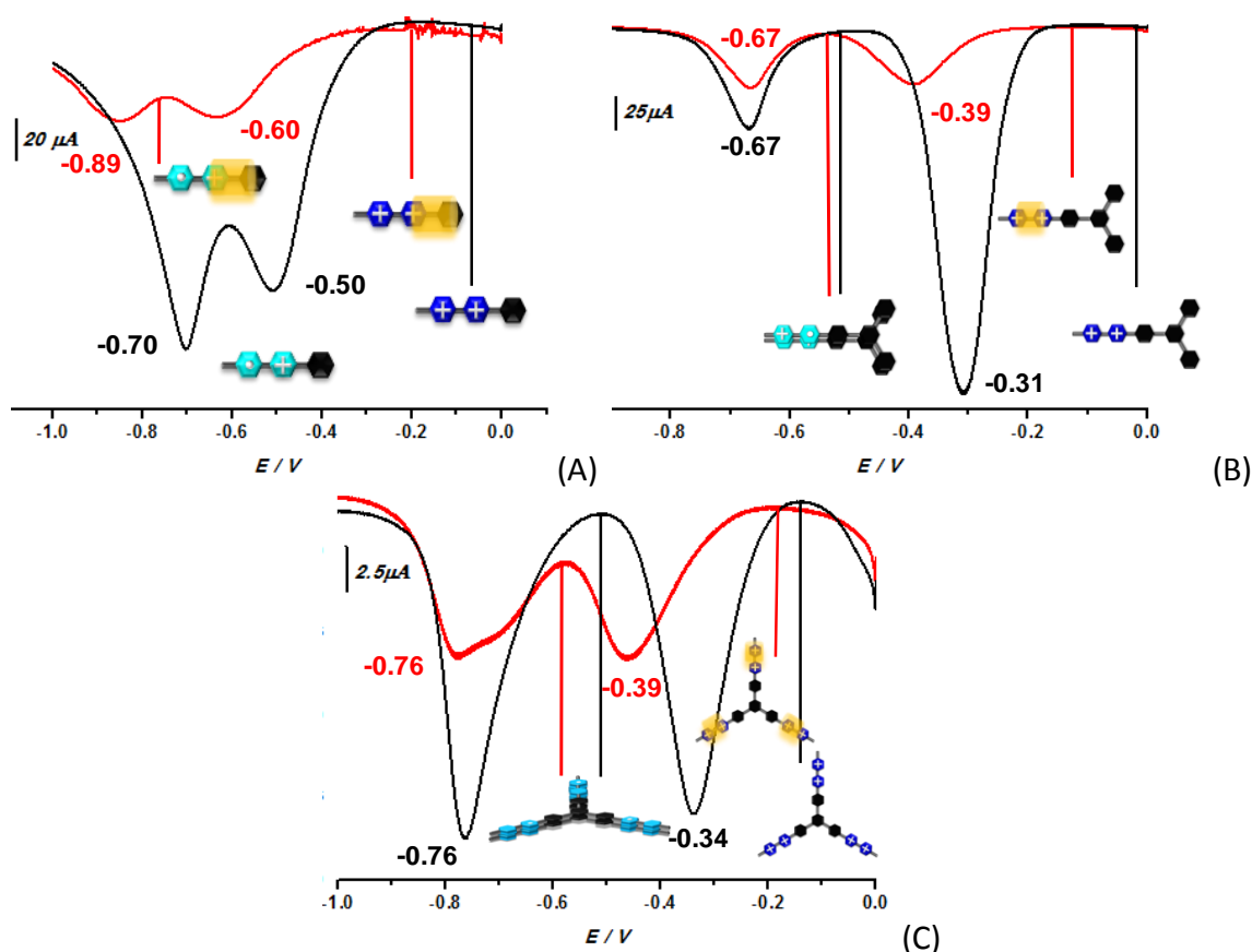
Figure 30. Square wave voltammograms (SWVs) of (A) MPV 2+ , (B) MVTP 2+ , and (C) TV 6+ in the absence and the presence of CB[7] (respectively 2, 4, and 8 equivalents of CB[7] ). All voltammograms were recorded in Argon-purged phosphate buffer solutions (pH 7) at 298 K. The scan rate was set at 1000 mVs -1 . E versus Ag/AgCl.
