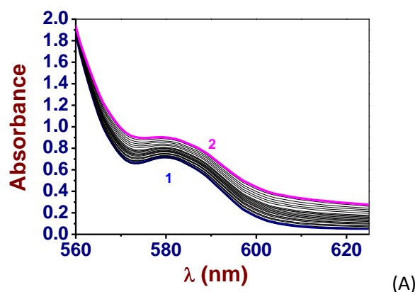
Figure 7. UV-Vis. absorption spectrophotometric titration of \text{ZnL}^1 by azo-phenanthryl-imidazole (noted API ). Solvent: 1,2-dichloroethane; T = 25.0(2)^\circ\text{C} ; l = 1\text{ cm} . (1). [\text{ZnL}^1]_0 = 4.80 \times 10^{-6}\text{ M} ; (2) [\text{API}]_0/[\text{ZnL}^1]_0 = 223.6 .
