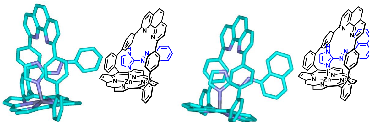
Figure 15. Schematic representation of the X-ray crystal structures of \text{ZnL}^1.\text{ABI} and \text{ZnL}^1.\text{ANI} .
