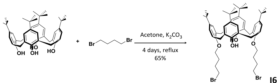
Figure 15. Synthesis of 1,3-bis(4-bromobutoxy)- p - tert -butyl-calix[4]arene ( I6 ).
