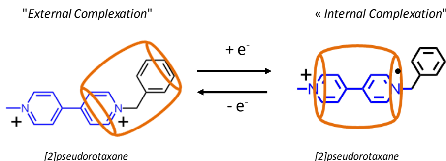
Figure 37. Electrochemically controlled translocation of the macrocycle CB[7] in the host/guest complex with BMV 2+ .
