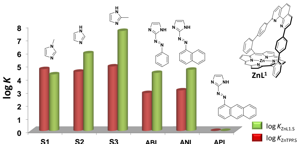
Figure 14. Schematic representation of the \log K_{ZnTPP.S} and \log K_{ZnL^1.S} values that shows the effect of hydrogen bonding with the phenanthroline strap on the extra-stabilization of the pentacoordinated complexes notwithstanding the bulkiness of the azo-chromophores.
