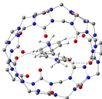
Figure 24. Molecular geometry of \text{MV}^{2+} \cdot \text{CB}[7] optimized at the B3LYP/6-31G(d) level.
