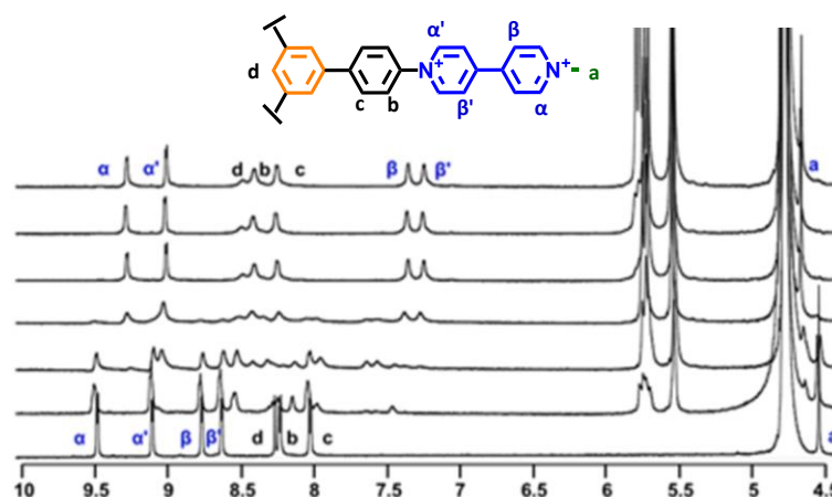
Figure 19. Full ^1\text{H} NMR spectra (600 MHz, \text{D}_2\text{O} , 298 K) of \text{TV}^{6+} in the presence of increasing amounts of \text{CB}[7] .
