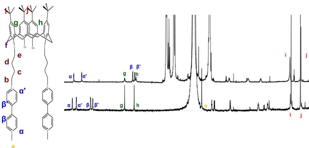
Figure 31. 1 H NMR spectra (600 MHz, D 2 O, 298 K) of C24 without and with and excess of CB[7] .
