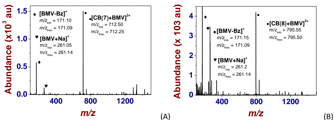
Figure 15. ESI mass spectra of the BMV 2+ complex formed with (A) CB[7] and (B) CB[8] . (A) [BMV^{2+}]_0 = 50 \mu\text{M} with 1 equivalent of CB[7] ; V_c = 280 \text{ V} . (B) [BMV^{2+}]_0 = 100 \mu\text{M} with 1 equivalent of CB[8] . V_c = 280 \text{ V} . Solvent: water; positive mode.
