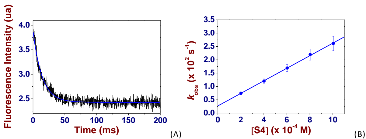
Figure 12. (A) Variation of the luminescence intensity versus time for the formation of \text{ZnL}^1\cdot\text{ABI} complex. Solvent: 1,2-dichloroethane; T = 25.0(2) \text{ }^\circ\text{C} ; l = 1 \text{ cm} ; [\text{ZnL}^1] = 1.07 \times 10^{-5} \text{ M} ; [\text{ABI}]_0/[\text{ZnL}^1]_0 = 10.43 . \lambda_{\text{exc}} = 554 \text{ nm} ; set of band pass filter ( \lambda > 550 \text{ nm} ). (B) Variation of the pseudo-first order constants k_{\text{obs}} ( \text{s}^{-1} ) for the formation of \text{ZnL}^1\cdot\text{ABI} complex versus [\text{ABI}]_{\text{tot}} . Solvent: 1,2-dichloroethane; T = 25.0(2) \text{ }^\circ\text{C} ; [\text{ZnL}^1] = 1.07 \times 10^{-5} \text{ M} .
