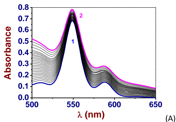
Figure 4. UV-Vis. absorption spectrophotometric titration of ZnTPP by azo-phenanthryl-imidazole (API). Solvent: 1,2-dichloroethane; T = 25.0(2)^\circ\text{C} ; l = 1\text{ cm} . (1) [\text{ZnTPP}]_0 = 3.4 \times 10^{-5}\text{ M} ; (2) [\text{API}]_0/[\text{ZnTPP}]_0 = 1015.7 .
