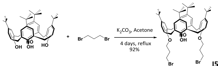
Figure 13. Synthesis of 1,3-bis(3-bromopropoxy)- p - tert -butyl-calix[4]arene ( I5 )
