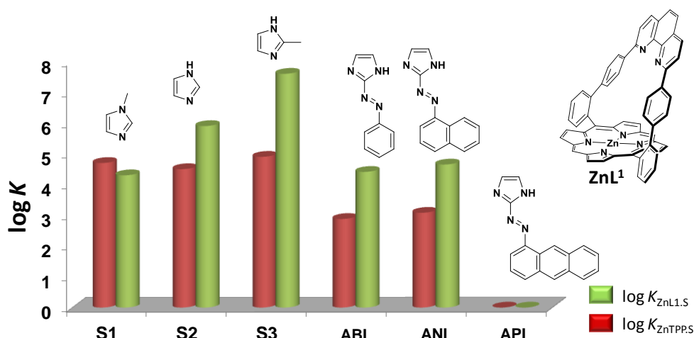
Figure 14. Schematic representation of the \log K_{\text{ZnTPP-S}} and \log K_{\text{ZnL}^1\text{-S}} values that shows the effect of hydrogen bonding with the phenanthroline strap on the extra-stabilization of the pentacoordinated complexes notwithstanding the bulkiness of the azo-chromophores.
