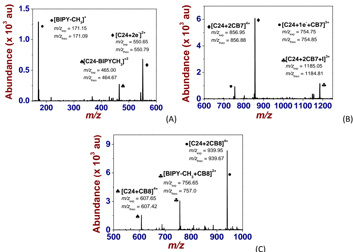
Figure 27. (A) ESI mass spectrum of free C24 4+ . [\text{C24}^{4+}]_0 = 4.7 \times 10^{-5} \text{ M} . Solvent: \text{H}_2\text{O} ; positive mode. V_c = 150 \text{ V} . \bullet = [\text{BIPY-CH}_3]^+ , m/z_{\text{exp}} = 171.15 , m/z_{\text{theo}} = 171.09 . \heartsuit = [\text{C24}^{4+} - \text{BIPY-CH}_3]^{2+} , m/z_{\text{exp}} = 465.00 , m/z_{\text{theo}} = 464.67 . \blacklozenge = [\text{C24}^{4+} + 2\text{e}]^{2+} , m/z_{\text{exp}} = 550.65 , m/z_{\text{theo}} = 550.79 .
