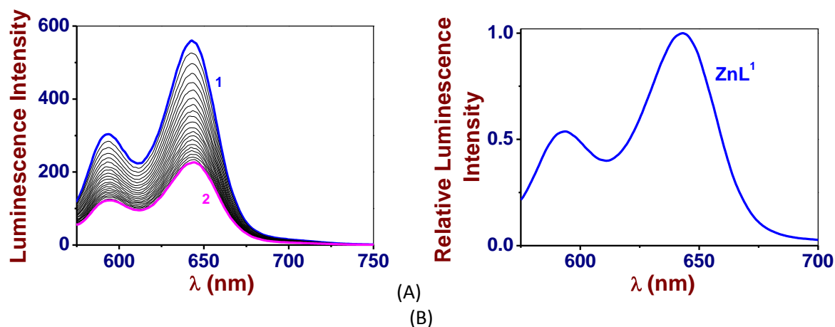
Figure 10. (A) Spectrofluorimetric titration of ZnL 1 receptor by azo-benzene-imidazole ( ABI ). \lambda_{\text{exc}} = 554 nm; exc. and em. slits 15/20 nm; (1) [\text{ZnL}^1]_{\text{tot}} = 4.7 \times 10^{-6} M; (2) [\text{ABI}]_0/[\text{ZnL}^1]_0 = 9.66 . (B) Relative reconstituted emission spectra of ZnL 1 and its pentacoordinated complex with ABI .
