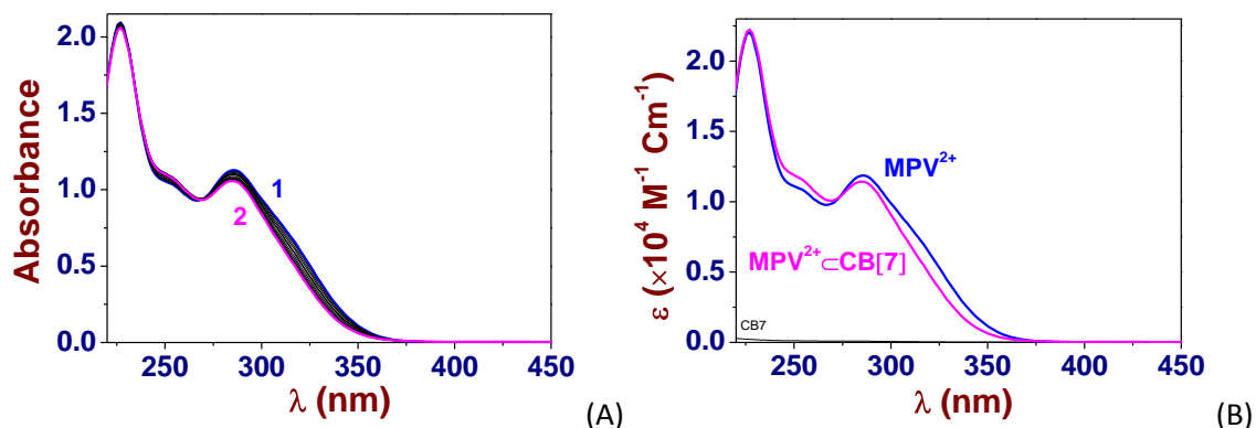
Figure 2. A) UV-Vis. absorption titration of \text{MPV}^{2+} by \text{CB}[7] . B) Electronic spectra of \text{MPV}^{2+} and its inclusion complex with \text{CB}[7] ( \text{MPV}^{2+} \subset \text{CB}[7] ). Solvent: water pH 7.0 (0.1 M \text{Na}_2\text{H}_2\text{PO}_4/\text{NaH}_2\text{PO}_4 ). [\text{MPV}^{2+}]_0 = 9.5 \times 10^{-5} \text{ M} ; (1) [\text{CB}[7]]_0/[\text{MPV}^{2+}]_0 = 0 ; (2) [\text{CB}[7]]_0/[\text{MPV}^{2+}]_0 = 3.75 ; l = 1 \text{ cm} ; T = 25.0(1)^\circ\text{C} . The absorption spectra are not corrected from dilution effects.
