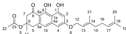
Acetylvismione D C 27 H 32 O 6 452,55 g/mol
