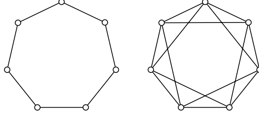
Figure 1.2 – an odd hole of length 7 and its corresponding odd antihole
