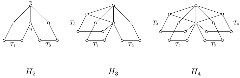
Figure 8.6 – the graphs H_2 , H_3 and H_4
