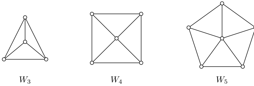
Figure 3.7 – examples of wheels
