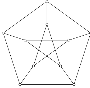
Figure 3.1 – a 3-regular simple graph ( Petersen's graph )
