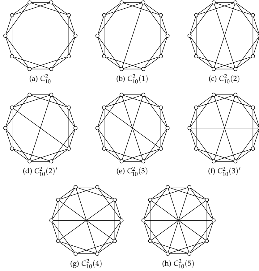
Figure 5.7 – the (3,3) -graphs obtained from C_{10}^2
