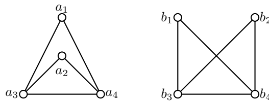
Figure 3.2 – two isomorphic graphs ( a_i \rightarrow b_i is an isomorphism)
