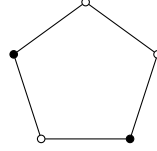
Figure 1.1 – the 5-circuit and a largest stable set (in black). It cannot be covered by 2 cliques
