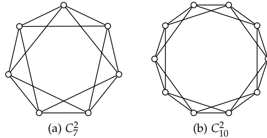
Figure 5.5 – the minimally t -imperfect graphs C_7^2 and C_{10}^2
