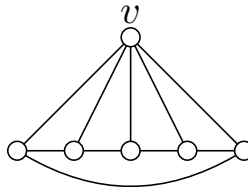
Figure 4.4 – substituting a vertex of K_2 by C_5
