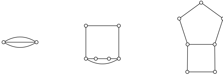
Figure 8.7 – examples of odd thetas
