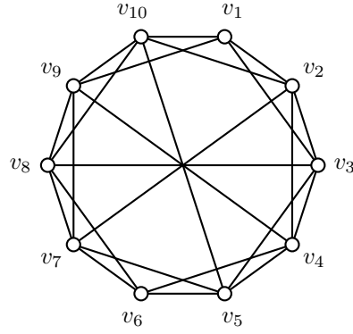
Figure 5.9 – denoting the vertices of \overline{C_{10}^2(1)} for the proof of Proposition 5.2.16
