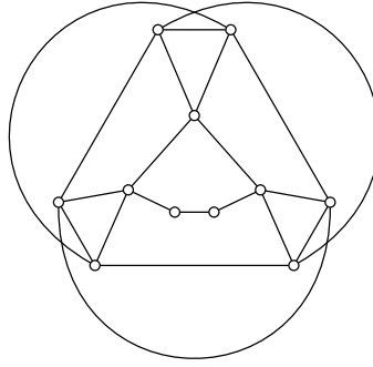
Figure 7.2 – an example of a 3-colorable t-perfect graph which does not have the IRCN
