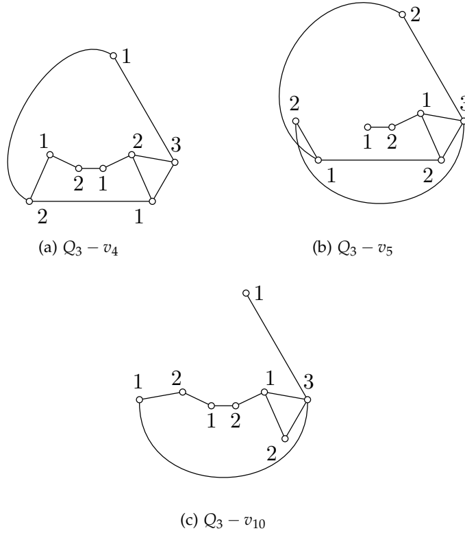
Figure 7.5 – a 3-coloring with one color used exactly once
