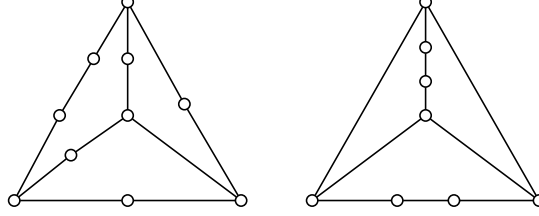
Figure 3.4 – non-totally and totally odd subdivisions of K_4
