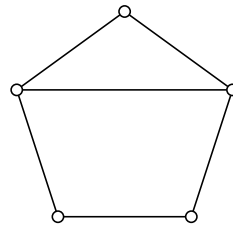
Figure 6.2 – the graph C_5^+ , also known as the house
