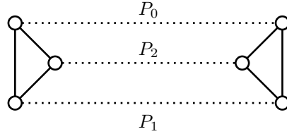
Figure 3.12 – a graph is a skewed prism if it is not isomorphic to K_4 and is formed by two vertex-disjoint triangles joined by three vertex-disjoint paths P_0 , P_1 and P_2 (drawn dotted) such that: both P_0 and P_2 are even, and P_1 is odd. There are no other edges.
