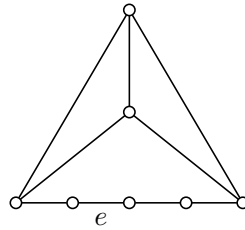
Figure 3.9 – contracting an edge does not keep h-perfection
