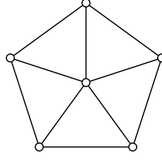
Figure 5.3 – the graph W_5
