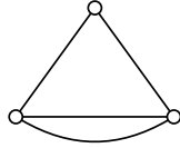
Figure 8.5 – the graph C_3^+
