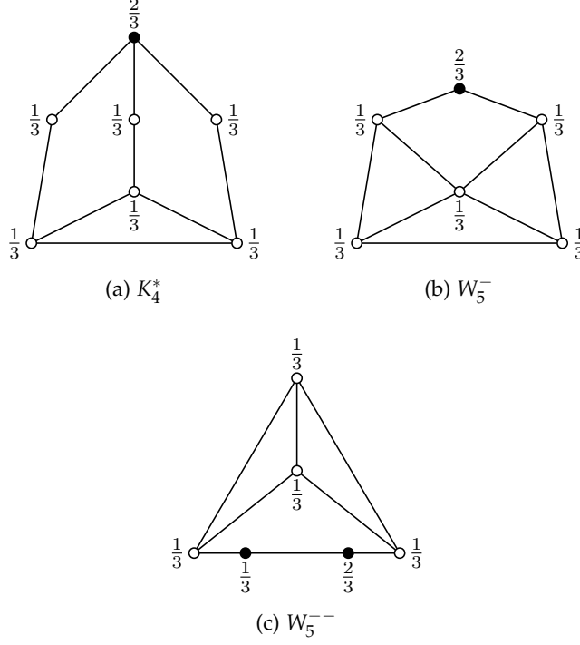
Figure 4.2 – the graphs K_4^* , W_5^- and W_5^{--} , their respective special vertices (shown black-filled) and a non-integral vertex of F_h at a special vertex.
