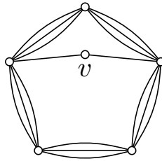
Figure 6.8 – the graph H_3
