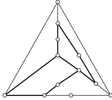
Figure 8.9 – a counter-example to the construction of [18] for odd- C_5^+ -free graphs
