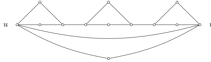
Figure 8.8 – an odd- C_5^+ -free 2-connected elementary critical non-bipartite graph which is not critical non-basic
