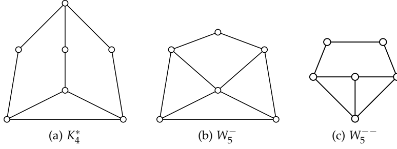
Figure 5.2 – the graphs K_4^* , W_5^- and W_5^{--}
