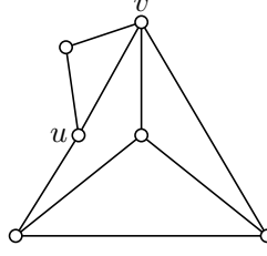
Figure 3.10 – deleting an edge does not keep h-perfection
