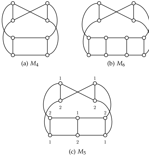
Figure 5.4 – examples of Möbius ladders and a 2-vertex-coloring of M_5
