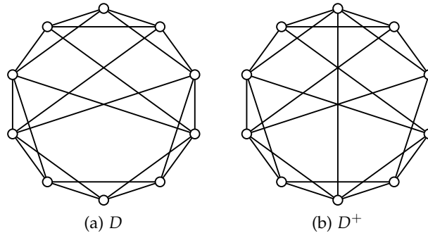
Figure 5.8 – the (3,3) -graphs obtained from D
