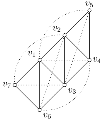
Figure 6.5 – the construction of v_1, \dots, v_7 . Dotted lines indicate pairs of non-adjacent vertices.
