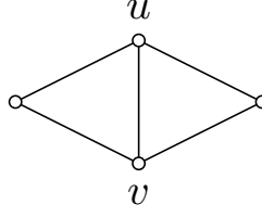
Figure 6.3 – a diamond with central vertices u, v
