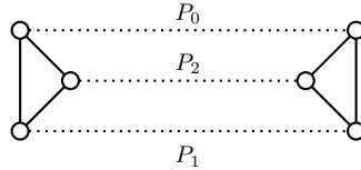
Figure 5.12 – a graph is a skewed prism if it is not isomorphic to K_4 and is formed by two vertex-disjoint triangles joined by three vertex-disjoint paths P_0 , P_1 and P_2 (drawn dotted) such that: both P_0 and P_2 are even, and P_1 is odd. There are no other edges.
