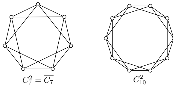
Figure 3.8 – examples of webs
