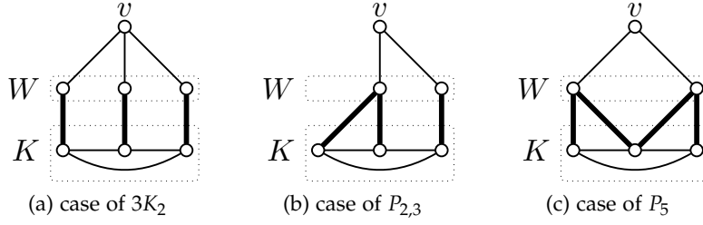
Figure 4.3 – obtaining an induced K_4^* , W_5^{--} and W_5^- of G from subgraphs of H
