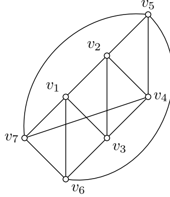
Figure 6.6 – CASE 1. building a C_7^2 from v_1, \dots, v_7 when N_G(v_4) \cup N_G(v_6) \subseteq V(H) .
