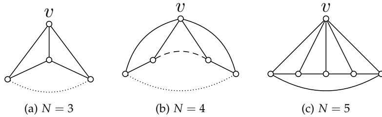
Figure 5.11 – The different possibilities for H : dotted and dashed lines denote pairwise-disjoint paths. Each ordinary line denotes an edge, dotted lines correspond to odd paths and the dashed one to a non-trivial even path. There is no other edge.
