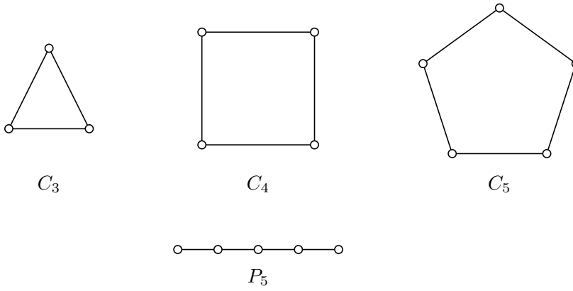
Figure 3.6 – examples of circuits and paths
