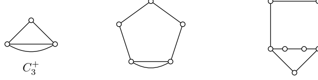
Figure 8.1 – C_3^+ and two \text{odd-}C_3^+ graphs
