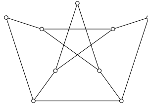
Figure 8.3 – the Petersen graph minus a vertex
