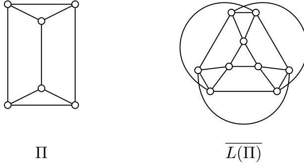
Figure 7.1 – the prism \Pi and the complement of its line graph
