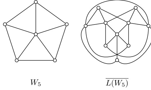
Figure 7.3 – the 5-wheel and the complement of its line-graph
