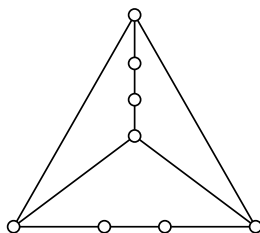
Figure 8.4 – a totally odd subdivision of K_4 . Each edge of K_4 is replaced with an odd path
