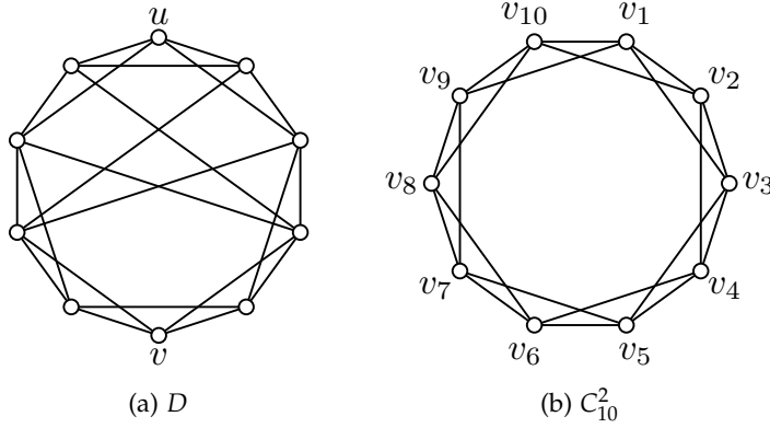
Figure 5.6 – the two normalized (3, 3) -graphs
