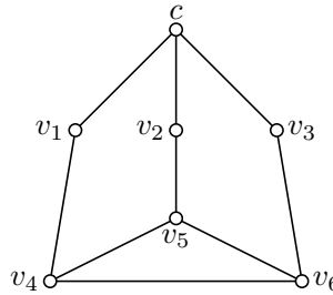
Figure 5.10 – notation for the vertices of K_4^*
