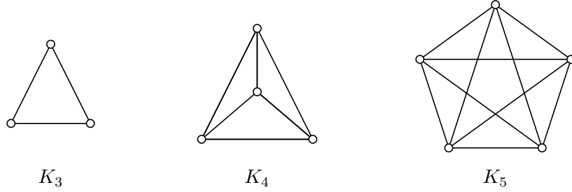
Figure 3.5 – examples of complete graphs
