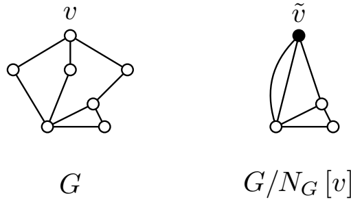
Figure 4.1 – a t-contraction at vertex v
