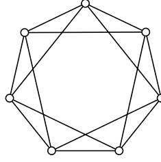
Figure 6.4 – the graph C_7^2
