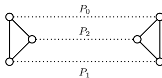
Figure 5.12 – a graph is a skewed prism if it is not isomorphic to K_4 and is formed by two vertex-disjoint triangles joined by three vertex-disjoint paths P_0 , P_1 and P_2 (drawn dotted) such that: both P_0 and P_2 are even, and P_1 is odd. There are no other edges.
