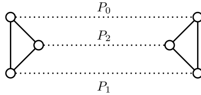
Figure 3.12 – a graph is a skewed prism if it is not isomorphic to K_4 and is formed by two vertex-disjoint triangles joined by three vertex-disjoint paths P_0, P_1 and P_2 (drawn dotted) such that: both P_0 and P_2 are even, and P_1 is odd. There are no other edges.
