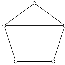
Figure 6.2 – the graph C_5^+ , also known as the house
