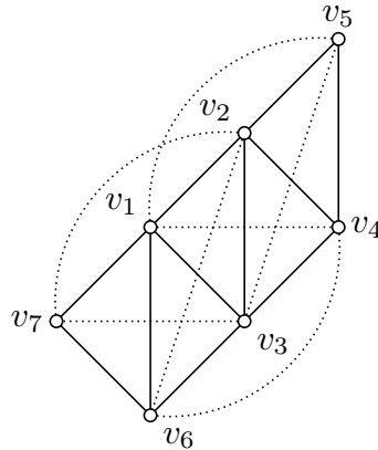
Figure 6.5 – the construction of v_1, \dots, v_7 . Dotted lines indicate pairs of non-adjacent vertices.
