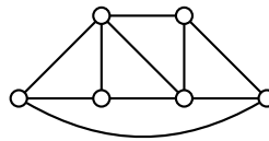
Figure 7.8 – the graph \overline{P_6}
