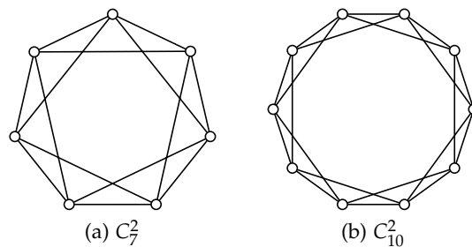
Figure 5.5 – the minimally t-imperfect graphs C_7^2 and C_{10}^2
