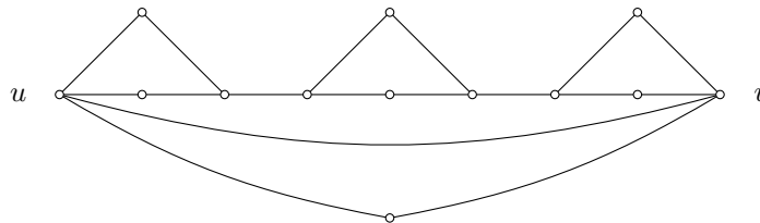
Figure 8.8 – an odd- C_5^+ -free 2-connected elementary critical non-bipartite graph which is not critical non-bipartite
