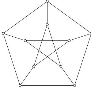
Figure 3.1 – a 3-regular simple graph ( Petersens's graph )
