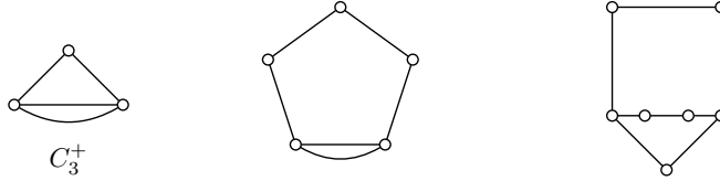
Figure 8.1 – C_3^+ and two odd-C_3^+ graphs
