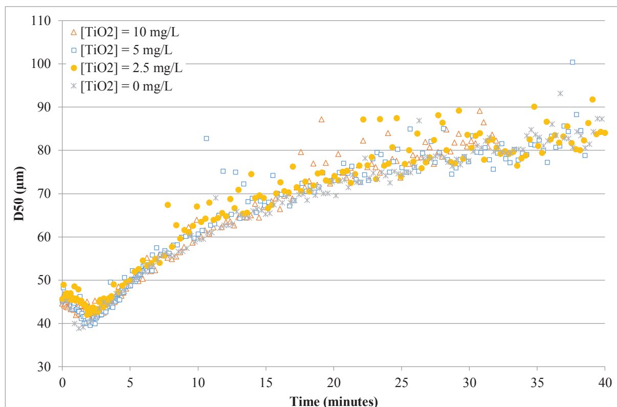
Figure 4: Evolution of illite and TiO 2 NPs aggregates diameters with time in river water ([Ca] = 3 mM; pH 8). Laser diffraction measurements, D50 = median diameter of aggregates
