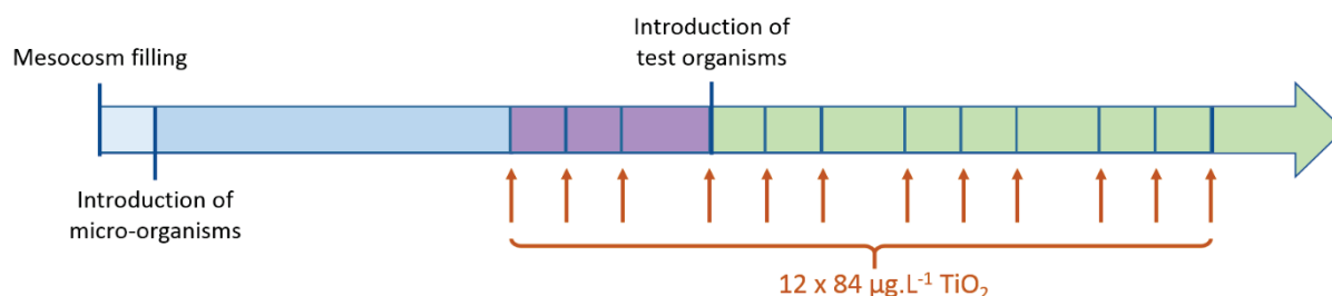
Figure 39: Time schedule for mesocosms experiments
