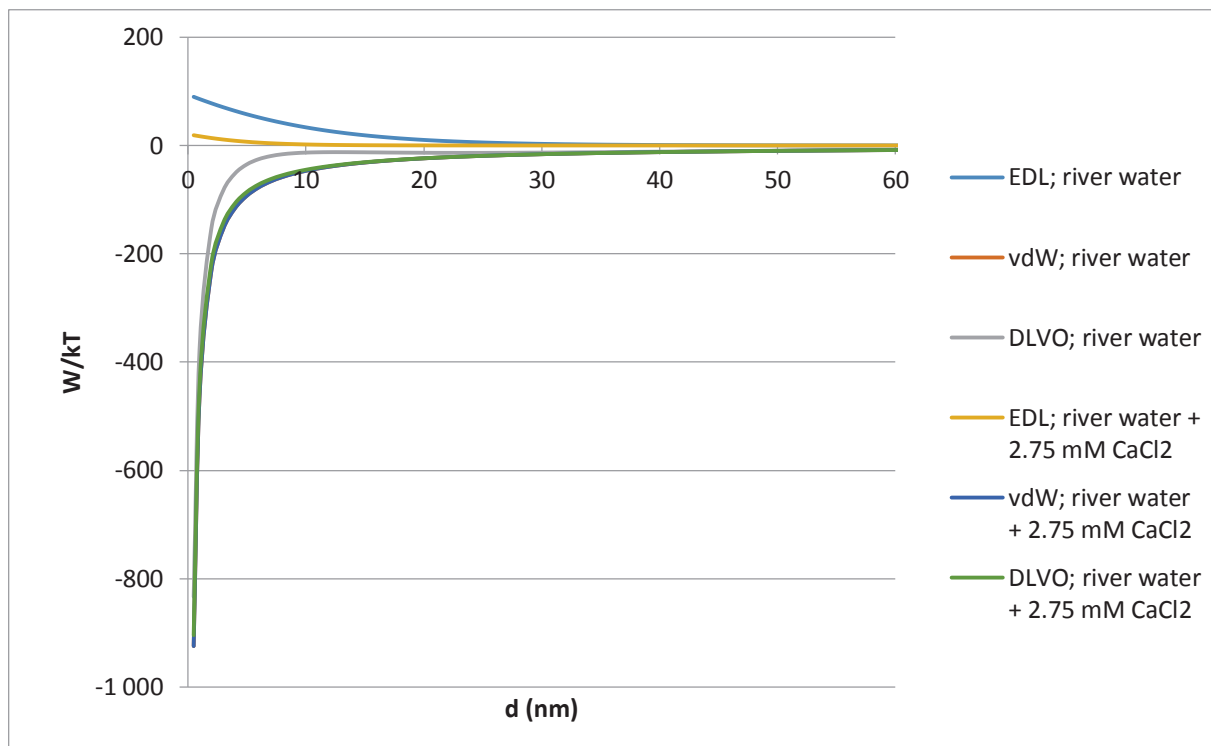
Figure S4: Interaction energies between \text{TiO}_2 NPs aggregates in the river water and in the river water with added \text{CaCl}_2 (pH 8)
