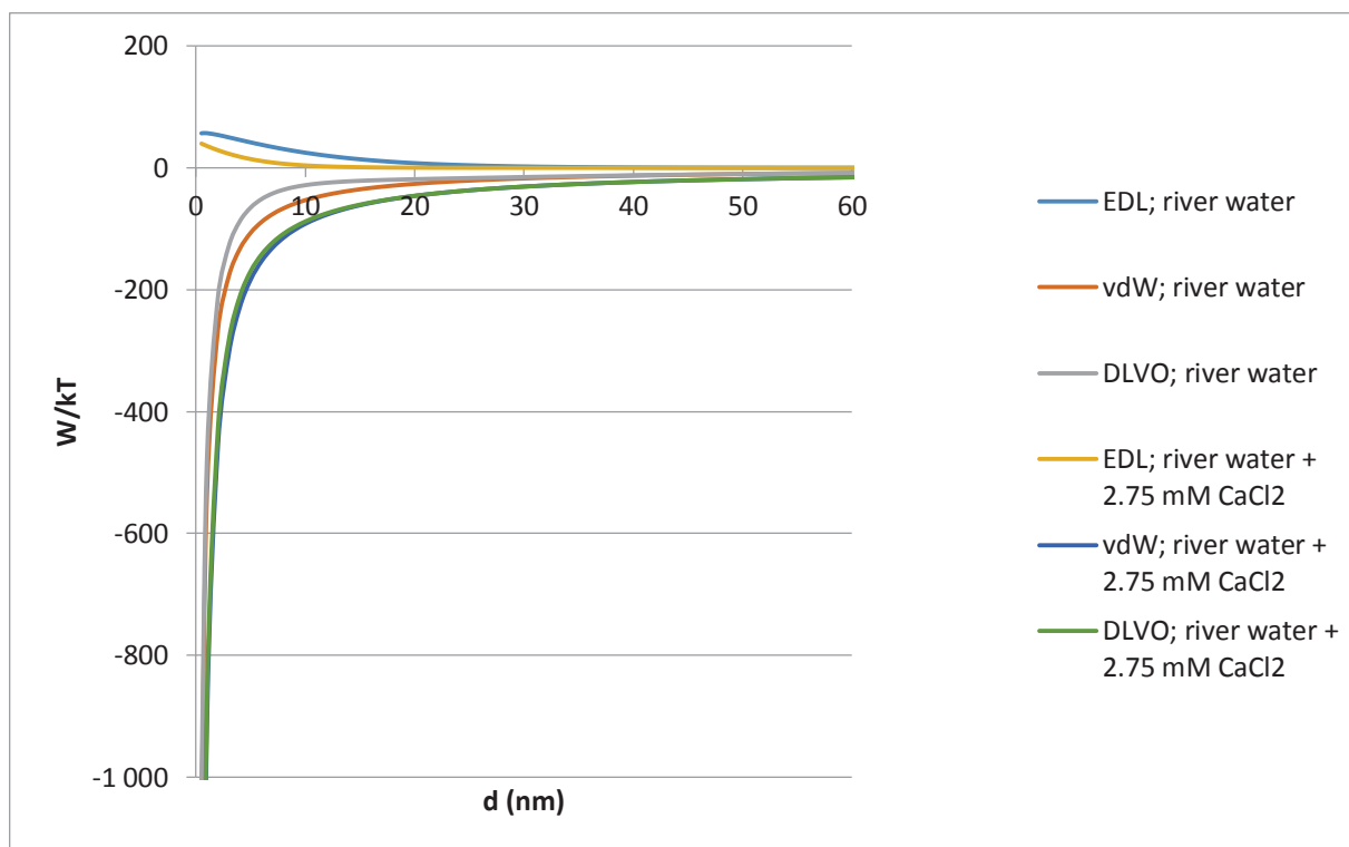
Figure S5: Interaction energies between \text{TiO}_2 NPs and illite aggregates in the river water and in the river water with added \text{CaCl}_2 (pH 8)
