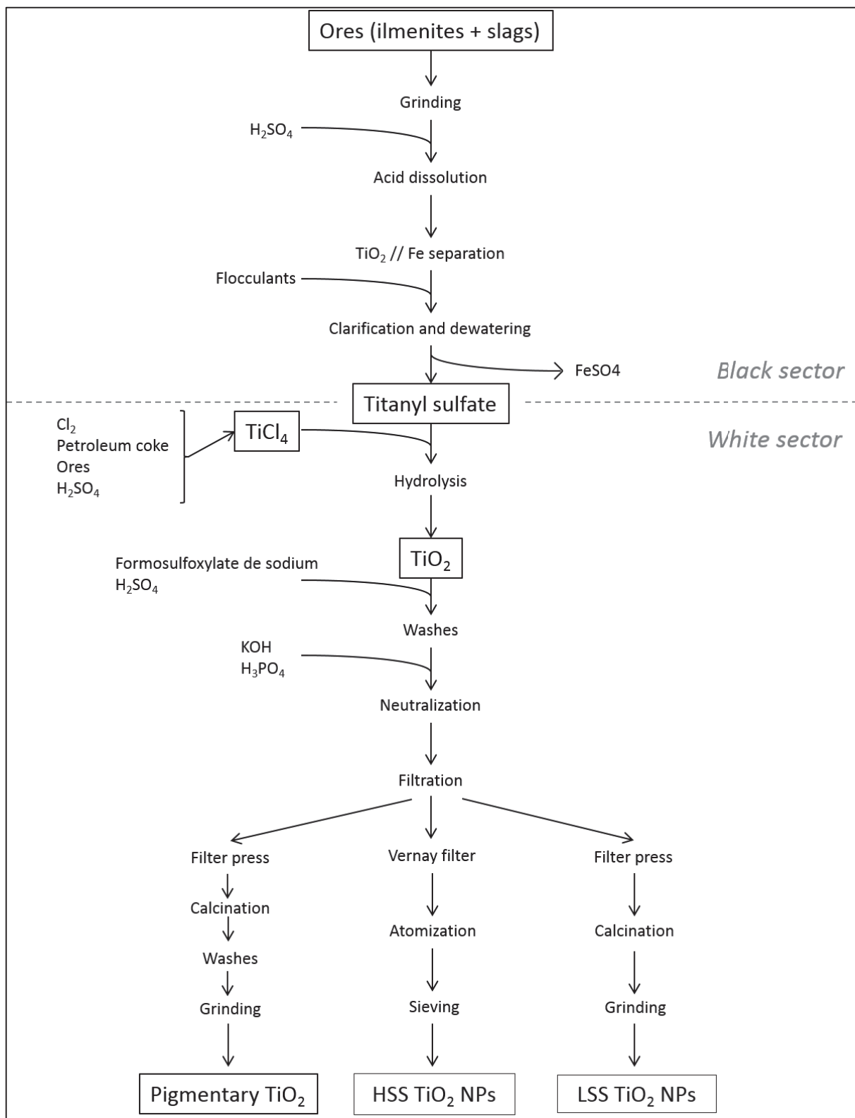
Figure 2: Nanoparticulate and pigmentary \text{TiO}_2 fabrication process (adapted from a factory communication)
