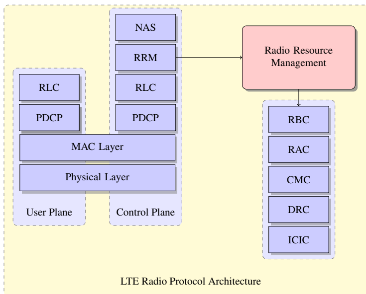
Fig. 2.2 LTE Radio Protocol Architecture
