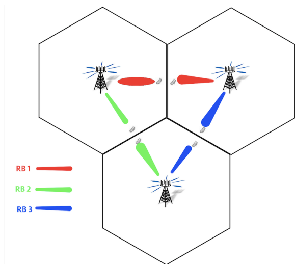
Fig. 4.1 RB allocation with Beamforming: the worst case
