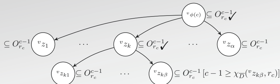
Figure 3.5 – The bottom-up procedure, cf. Proposition 3.8.
