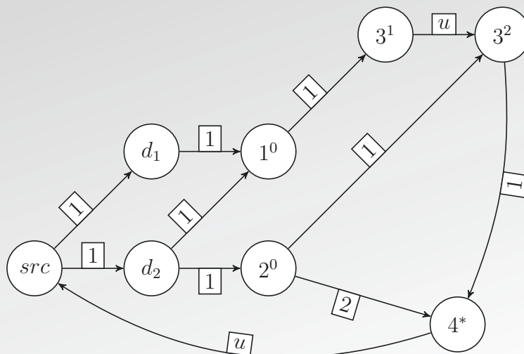
Figure 2.6 –The simplified transportation network associated with the instance of the delivery problem given on page 29.
