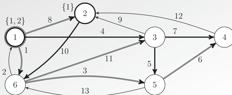
Figure 1.1 – The dissemination problem (an example).
