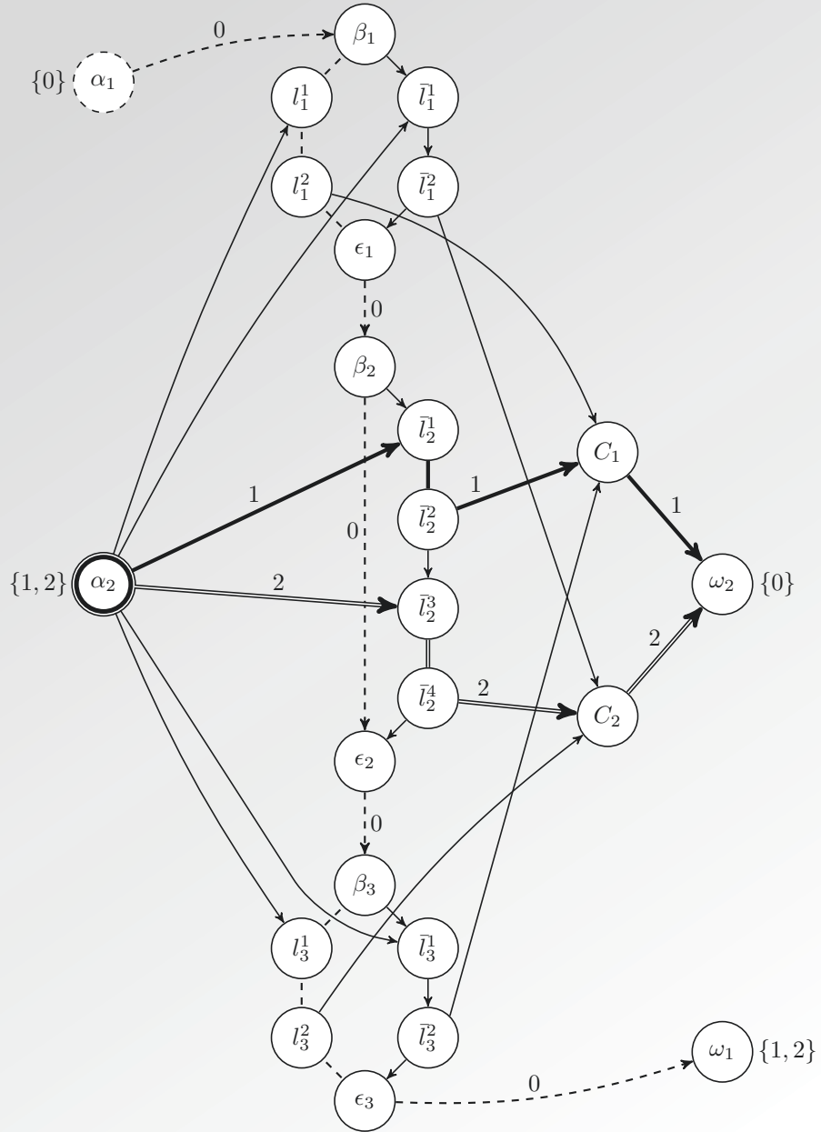
Figure 2.4 – The DT2R instance associated with the 3-SAT instance given on page 17.
