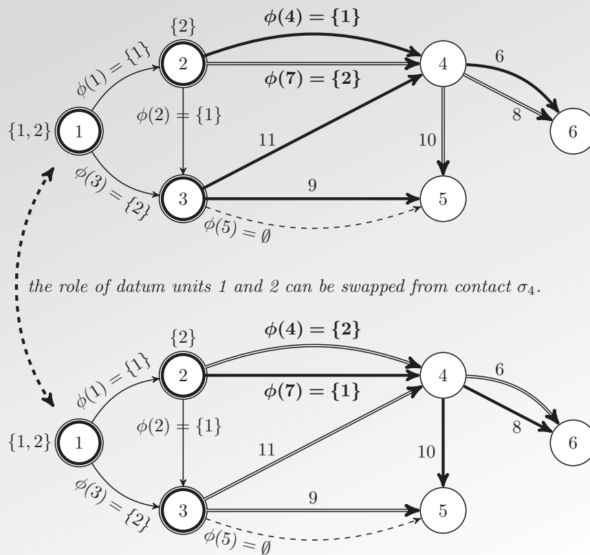
Figure 4.2 – A symmetry appears between datum units 1 and 2 when we try to set transfer \phi(4) .
