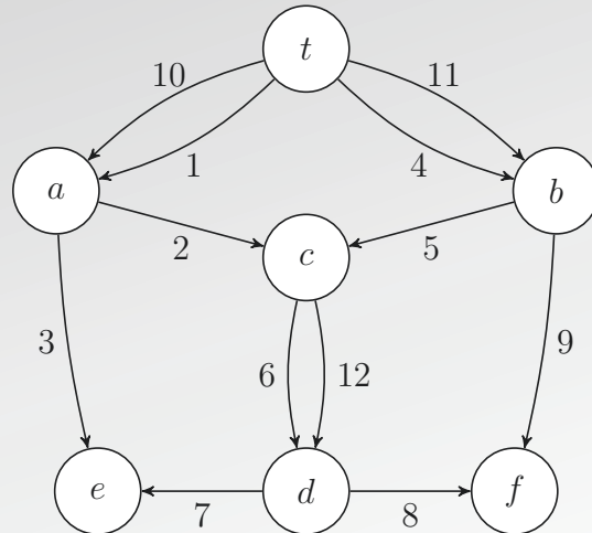
Figure 2.7 – This counter-example shows Theorem 2.6 no longer holds for evolving graphs.
