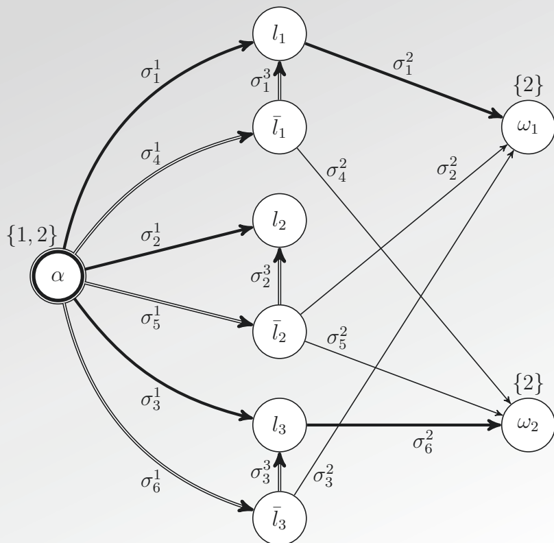
Figure 2.1 – The DT2U instance associated with the 3-SAT instance given on page 17.
