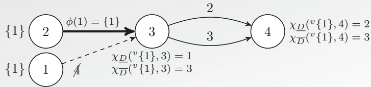
Figure 3.7 – The delivery-requirement-based deductive reasoning (Proposition 3.11).
