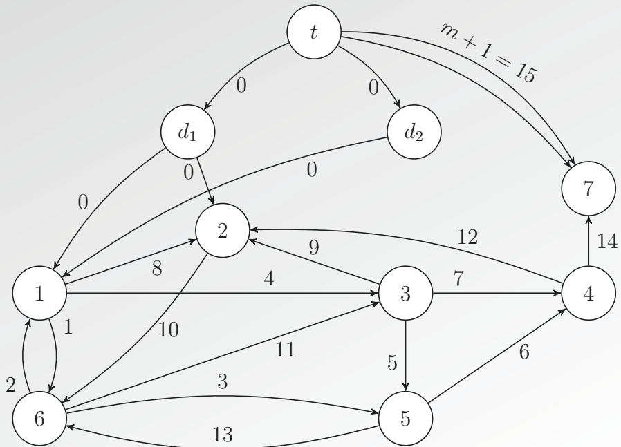
Figure 2.8 – An instance of the data transfer problem (DT) and the corresponding ADBEG instance.
