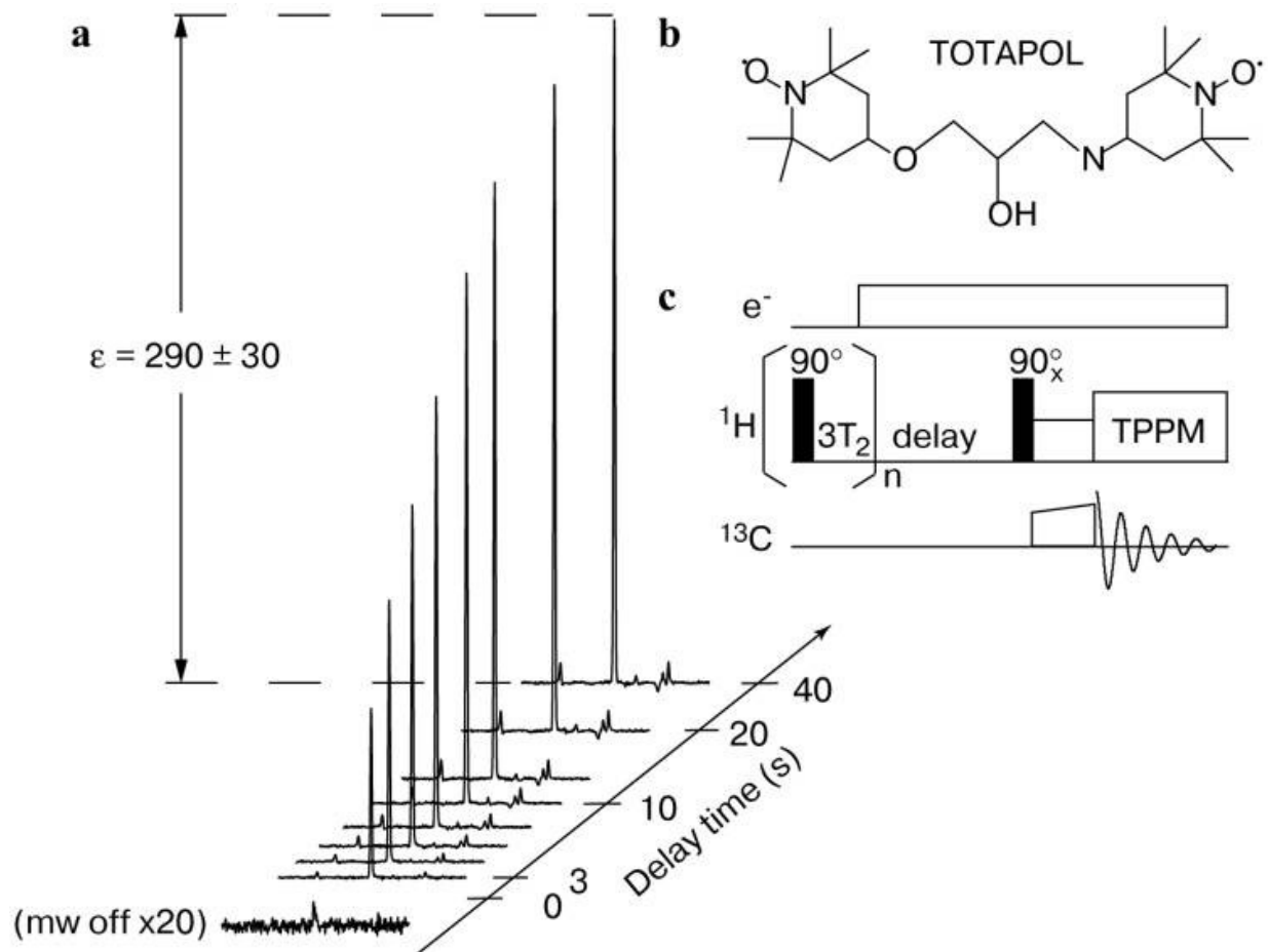
Figure I.5. (a) The build-up of the ^1\text{H} \rightarrow ^{13}\text{C} CPMAS signal of 2M ^{13}\text{C} -urea with 3 mM TOTAPOL in a frozen solution of [\text{H}_2]_6\text{-DMSO}/^2\text{H}_2\text{O}/\text{H}_2\text{O} (60/34/6 wt%) mixture as function of the \mu\text{w} irradiation time. (b) The structure of TOTAPOL, and (c) the ^1\text{H} \rightarrow ^{13}\text{C} CPMAS saturation-recovery pulse sequence. The experimental conditions are B_0 = 5 T, at a temperature of 90 K, and a MAS frequency of 7 kHz. Adapted from Ref. 35.
