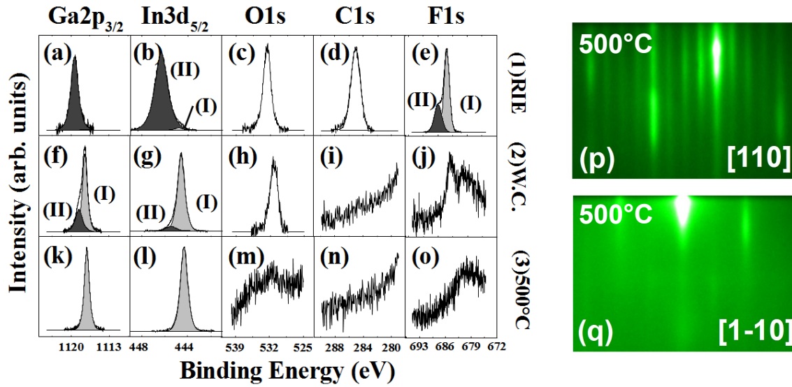
Figure 3.11: (a-o) XPS core levels of \text{Ga}2p_{3/2} , \text{In}3d_{5/2} , O1s, C1s and F1s recorded after different process steps. (1) Gate stack RIE, (2) Wet cleaning and (3) in-situ annealing at 500^\circ\text{C} for 5 minutes. (p,q) (4\times 2) surface reconstruction recorded by RHEED along the (p) [110] and (q) [1-10] azimuths of \text{In}_{0.53}\text{Ga}_{0.47}\text{As} (001), after in-situ annealing at 500^\circ\text{C} for 5 minutes.
