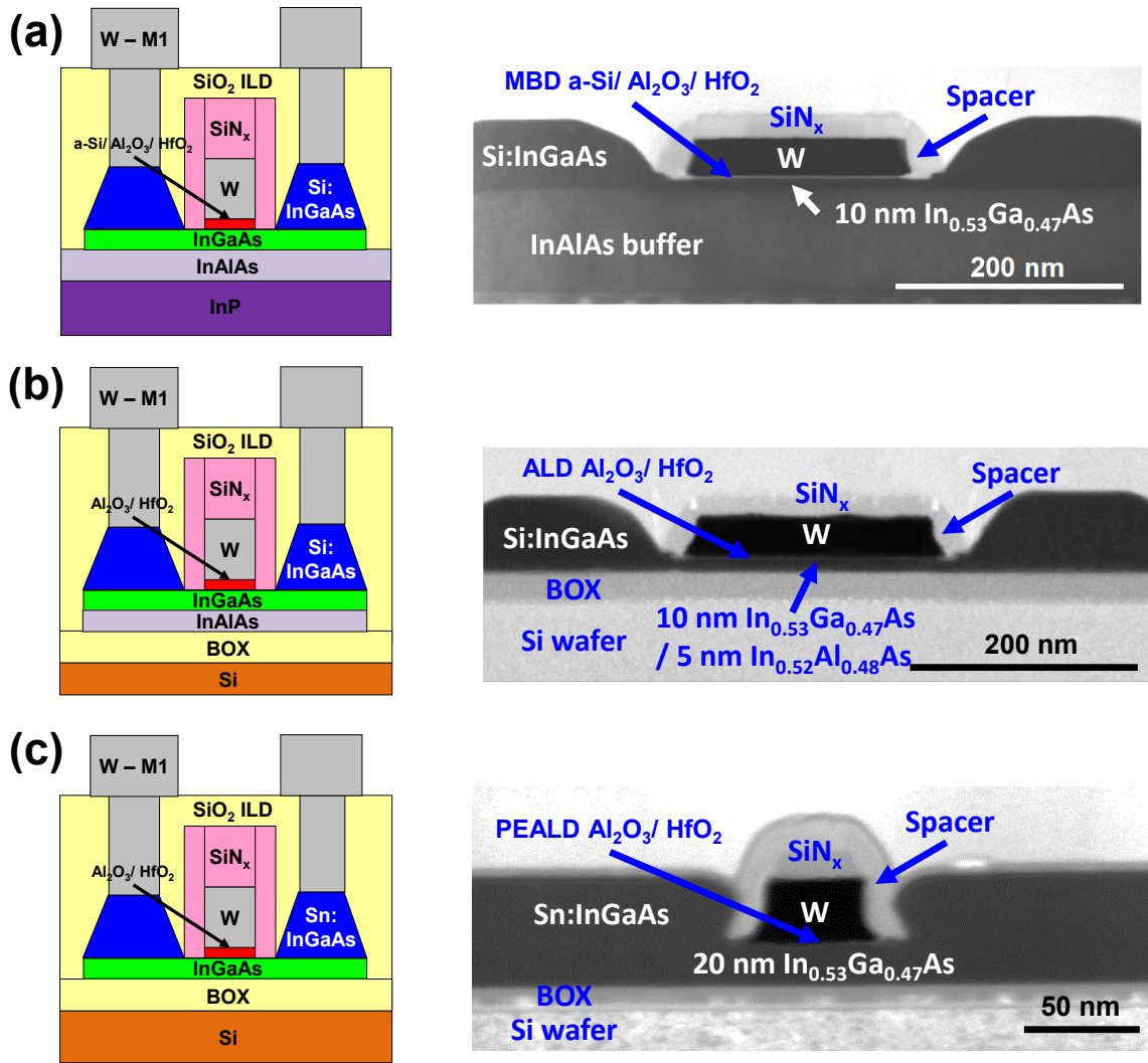
Figure 4.2: Schematic and TEM cross-sectional view of 3 types of self-aligned GF In 0.53 Ga 0.47 As MOSFETs: (a) “bulk” devices with t_{ch} = 10 nm, 1 nm a-Si/ 1 nm Al 2 O 3 / 2 nm HfO 2 gate stack, Si-doped RSD, with or without Ni-InGaAs contacts ; (b) “on-insulator” devices with t_{ch} = 10 nm on 5 nm InAlAs, 1 nm Al 2 O 3 / 3 nm HfO 2 gate stack, Si-doped RSD ; (c) “optimized on-insulator” devices with t_{ch} = 20 nm, 0.5 nm Al 2 O 3 / 3 nm HfO 2 gate stack, Sn-doped RSD.
