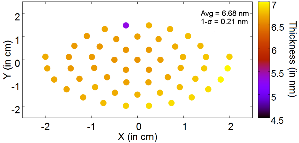
Figure 2.2: Ellipsometry thickness mapping of a 7 nm In 0.53 Ga 0.47 As active layer on a 10 nm BOX on Si after etch-stop removal.
