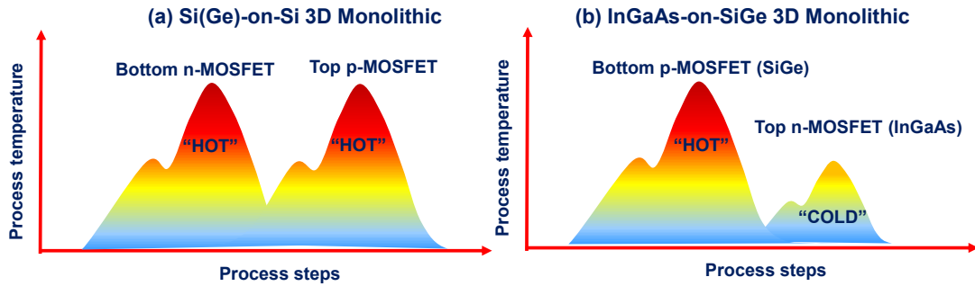
Figure 5.11: Illustration of thermal budget evolution versus processing steps for 3D monolithic integration of (a) SiGe or Si MOSFETs on top of Si MOSFETs and of (b) InGaAs MOSFETs on top of SiGe or Si MOSFETs.
