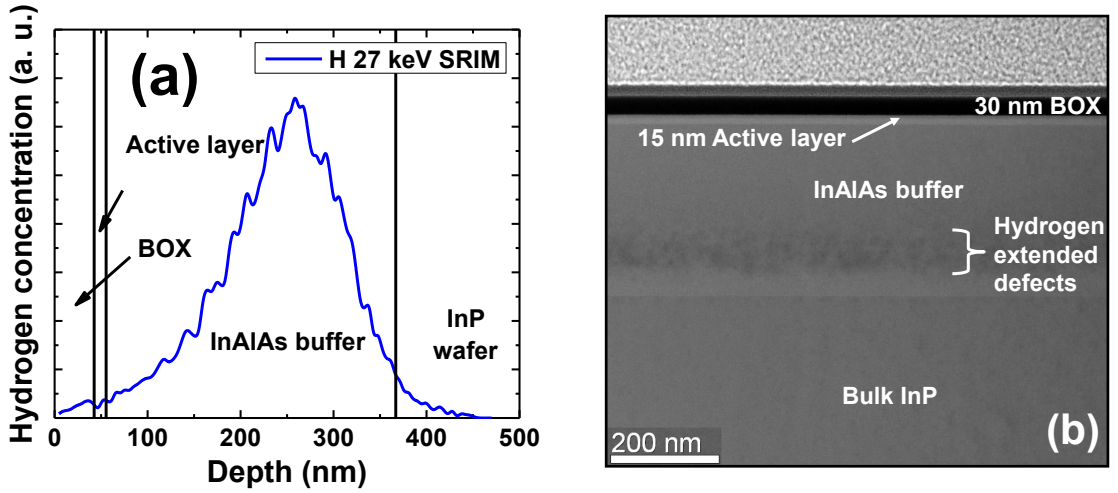
Figure 2.9: (a) SRIM [53] simulation of hydrogen dose implanted at 27 KeV in the III-V epitack. (b) Cross-sectional TEM image of the corresponding InP donor wafer with InAlAs (with 52% of indium) ( \text{In}_{0.52}\text{Al}_{0.48}\text{As} ) buffer, \text{In}_{0.53}\text{Ga}_{0.47}\text{As} active layer and \text{Al}_2\text{O}_3 BOX layer after hydrogen implantation.
