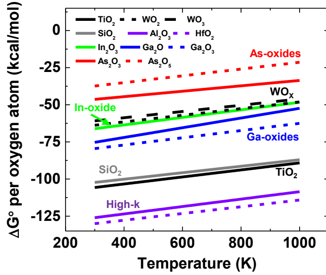
Figure 3.5: Gibbs free energy of oxidation per Oxygen atom plotted at 1 atm versus temperature for InGaAs oxides, high-k dielectrics ( \text{HfO}_2 , \text{Al}_2\text{O}_3 ), \text{SiO}_2 , W oxides and titanium-oxide ( \text{TiO}_2 ). Values calculated based on thermodynamic properties in [79, 80].
