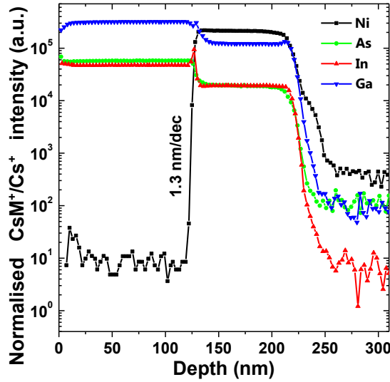
Figure 3.14: Back-side SIMS profile for 220 nm of \text{In}_{0.53}\text{Ga}_{0.47}\text{As} on InP after deposition of 50 nm Ni, annealed at 350^\circ\text{C} for 5 minutes.
