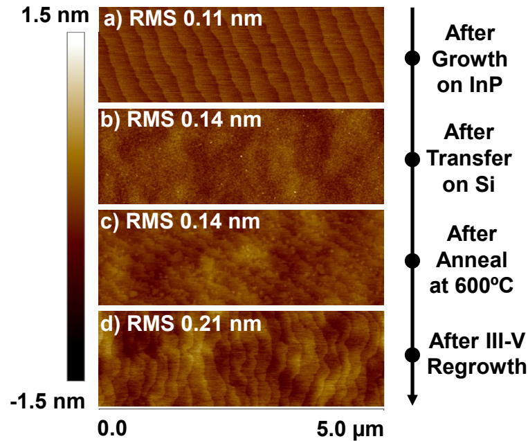
Figure 2.7: Atomic force microscopy (AFM) scans in tapping mode on the InGaAs surface after (a) growth on the donor wafer, (b) transfer to Si, (c) annealing at 600^{\circ}\text{C} under tertiarybutylarsine (TBA) and (d) about 50 nm \text{In}_{0.53}\text{Ga}_{0.47}\text{As} regrowth at 600^{\circ}\text{C} .
