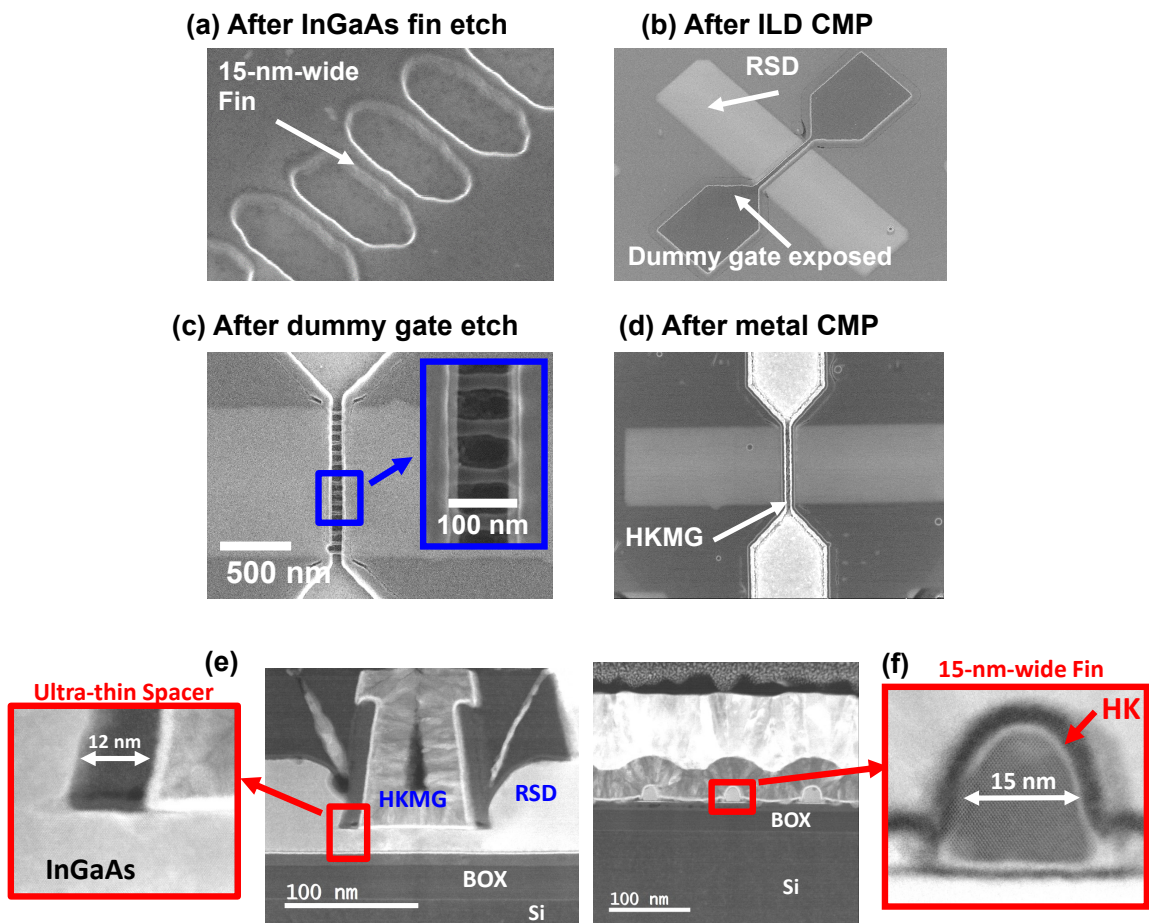
Figure 4.13: (a, b, c, d) SEM views taken at different critical stages of the RMG process: (a) after InGaAs fin patterning, (b) after SiO 2 ILD CMP exposing the top of the dummy gates, (c) after removal of the dummy gate and dummy HK, (d) after final HKMG deposition, W fill and metal CMP. (e, f) Cross sectionnal TEM image of a RMG InGaAs-OI MOSFET taken (e) across and (f) along the gate. Side insets show the scaled 12 nm thick SiN x spacers and 15 nm wide InGaAs fins.
