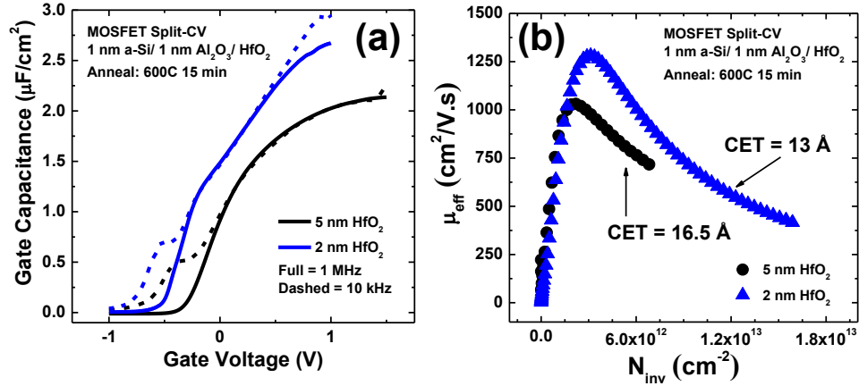
Figure 3.4: (a) Split C-V characteristics of W/ \text{HfO}_2 /1 nm \text{Al}_2\text{O}_3 /1 nm a-Si/ \text{In}_{0.53}\text{Ga}_{0.47}\text{As} MOSFETs with \text{HfO}_2 of nominally 5 nm and 2 nm annealed at 600°C for 15 minutes in the MOVPE system and measured at 25°C in the dark from 10 kHz to 1 MHz. (b) Effective mobility ( \mu_{\text{eff}} ) versus inversion-charge density ( N_{\text{inv}} ) for the same MOSFETs. The channel is 10 nm thick and non-intentionally doped (NID), on NID \text{In}_{0.52}\text{Al}_{0.48}\text{As} on InP.
