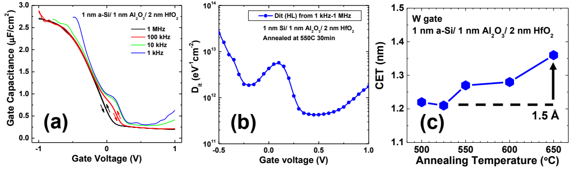
Figure 3.3: (a) C-V characteristics of a W/2 nm HfO 2 /1 nm Al 2 O 3 /1 nm a-Si/In 0.53 Ga 0.47 As MOS capacitor annealed at 550°C in Ar for 30 minutes and measured at 25°C in the dark from 1 kHz to 1 MHz. 100 kHz and 1 MHz curves are plotted with forward and reverse sweep. (b) D_{it} versus gate voltage extracted by the high-low frequency method [77]. (c) CET measured at 1 MHz versus annealing temperature in Ar for 30 minutes.
