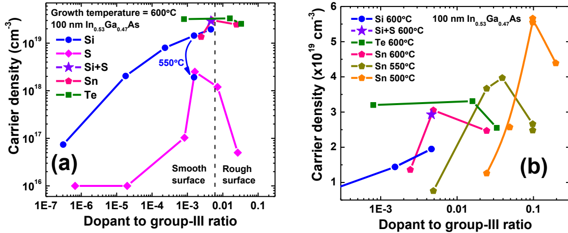
Figure 3.12: (a) Hall electron density versus dopant to group-III flux ratio for in-situ doped 100 \text{ nm In}_{0.53}\text{Ga}_{0.47}\text{As} grown at 600^\circ\text{C} with different n-type dopant species. The blue arrow indicates a Si doped sample grown at 550^\circ\text{C} . (b) Magnified Hall electron density versus dopant to group-III flux ratio focusing on the high doping region, for different dopant species and growth temperatures.
