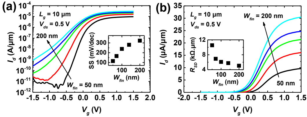
Figure 4.10: Transfer characteristics measured at V_{ds} = 0.5 V, on devices featuring a L_G of 10 \mu\text{m} , H_{fin} = 20 nm and W_{fin} ranging from 50 to 200 nm. Plotted in (a) log scale with SS vs W_{fin} in inset and (b) linear scale with source and drain series resistance ( R_{SD} ) vs W_{fin} in inset.
