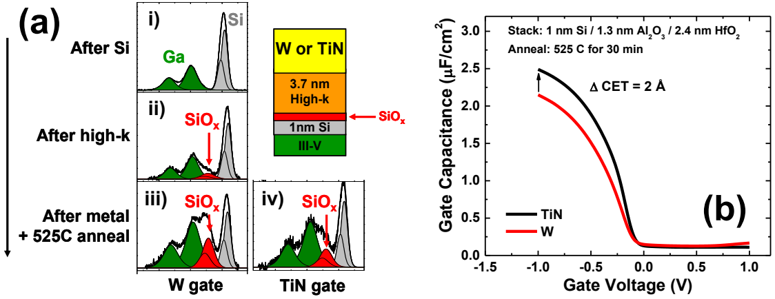
Figure 3.6: (a) Ga3p and Si2p core level XPS spectra after (i) hydrogen plasma and 1 nm a-Si deposition, (ii) 1.3 nm Al 2 O 3 and 2.4 nm HfO 2 deposition, (iv) post-metallization anneal at 525°C in Ar for 30 min. (b) MOSCAPs C-V characteristics at 1 MHz with two different gate metals (TiN and W).
