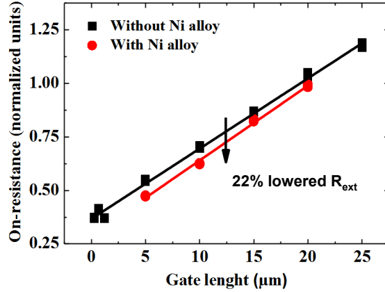
Figure 4.3: On-resistance versus gate length obtained on “bulk” MOSFETs with or without Ni-InGaAs contacts. The on-resistance is extracted from the drain current at V_g = 1 V and V_{ds} = 50 mV, normalized to 10 \text{ k}\Omega \cdot \mu\text{m} .
