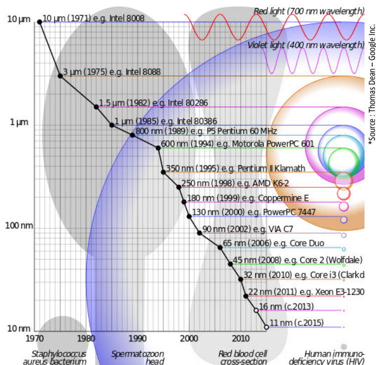
Fig. I-5. Lithography scaling.
