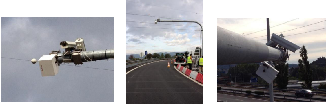
Fig. III-42. Pictures of the Multitoll DSRC system being installed on a Portuguese highway.
