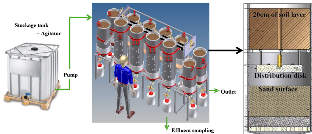
Fig.1 : Overview of the pilot batch experiment at a laboratory scale
