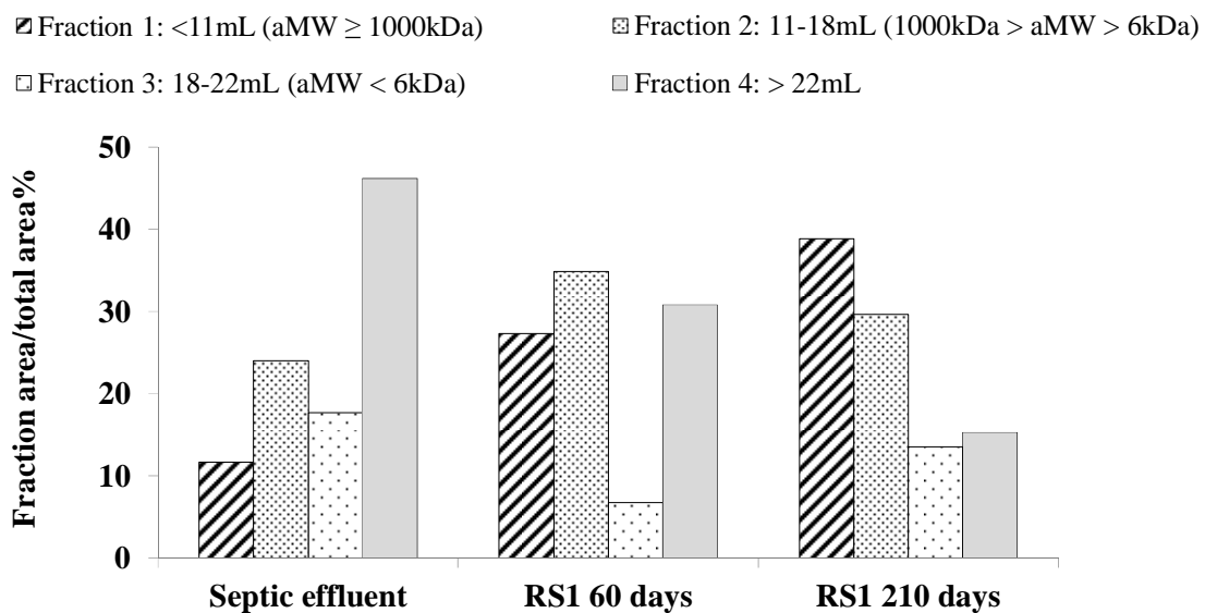
Fig.7. Evolution in the fractions of major group areas relative to total chromatographic areas of septic effluent and river sand biomass extraction at 60 and 210 days
