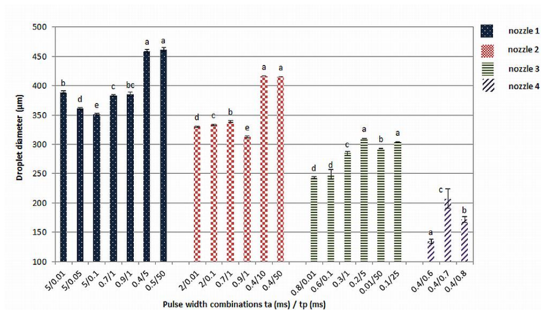
Figure 5.6. Droplet diameter ( \mu\text{m} , mean \pm std.) for different nozzles and pulse width combinations. Different letters indicate statistical differences within the same nozzle ( P < 0.05 )
