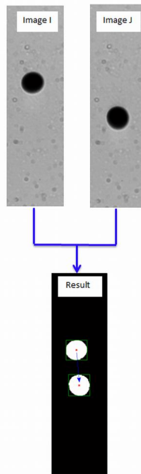
Figure 4.12 Droplet tracking result from two consecutive images in DOD mode.
