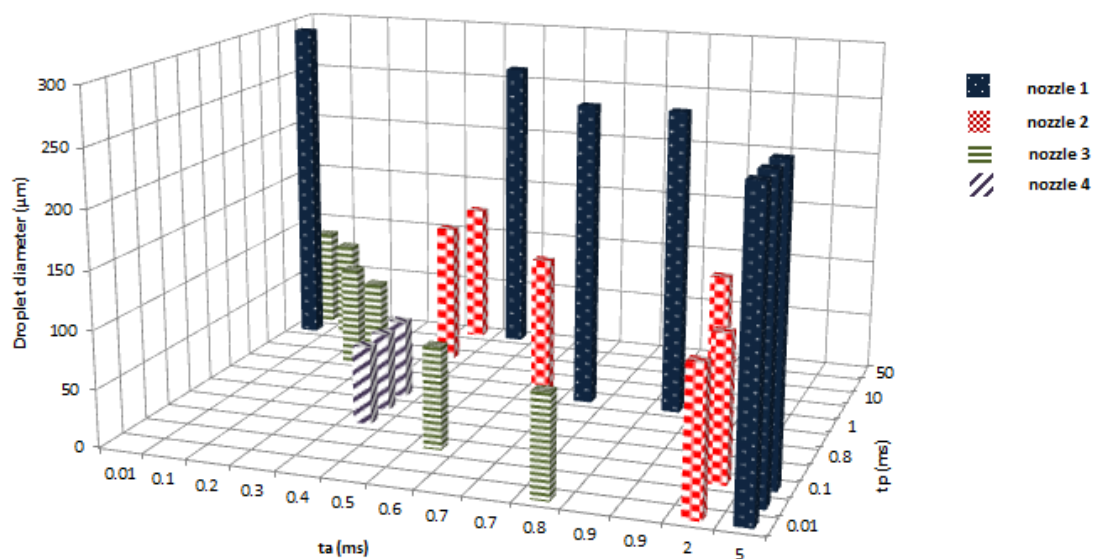
Figure 5.7. Mean droplet diameter results for the selected pulse width values for the 4 nozzles with V_p = \pm 4.5 \text{ V}
