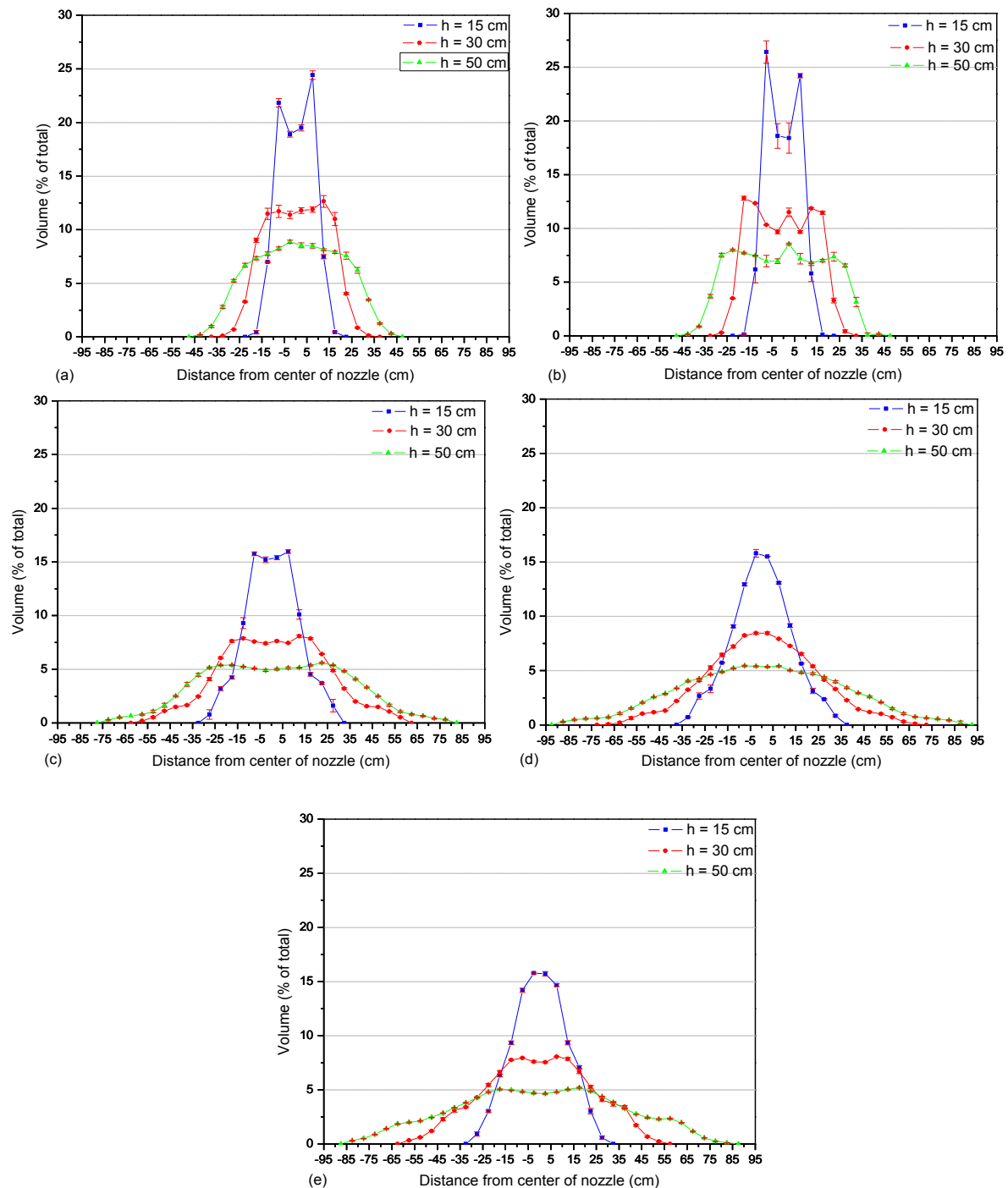
Figure 7.10. Spray distribution measurements (% and sd) at 3 different heights of the (a) Albus ATR orange nozzle at 600 kPa, (b) Albus ATR red nozzle at 800 kPa, (c) TeeJet XR 110 01 at 400 kPa, (d) TeeJet XR 110 04 at 400 kPa and (e) TeeJet AI 110 04 at 400 kPa
