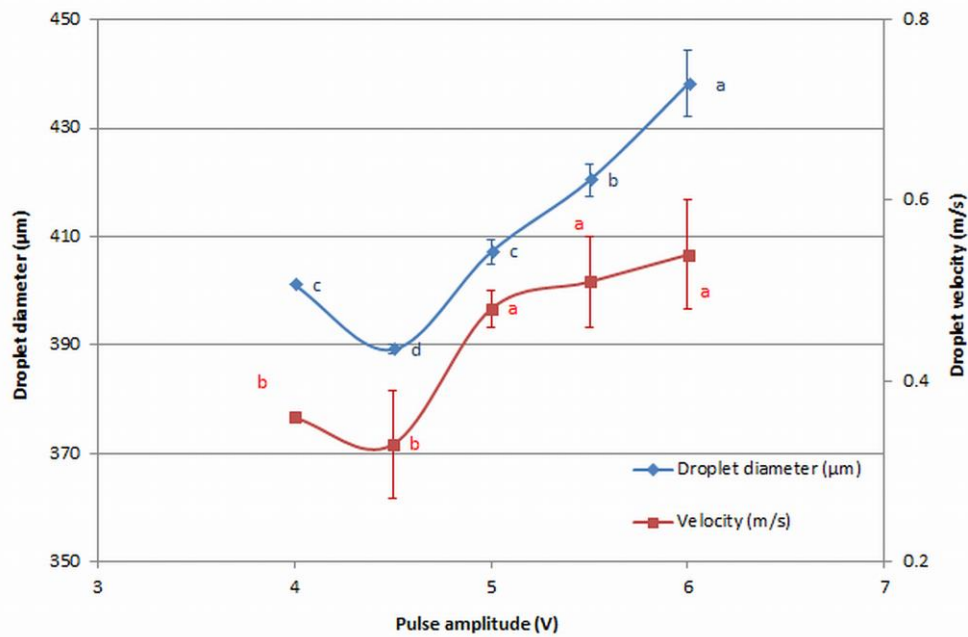
Figure 5.10. Droplet diameter ( \mu\text{m} , mean \pm std.) and velocity (m/s, mean \pm std.) for nozzle 1 at different pulse amplitudes and t_a = 5 ms and t_p = 0.01 ms. Different letters indicate statistical differences between data points within the same curve ( P < 0.05 )
