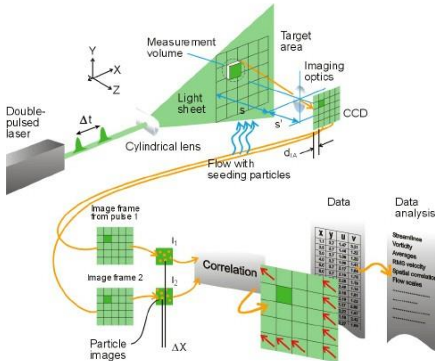
Figure 2.19. Measurement principals of PIV (Dantec Dynamics Inc.)
