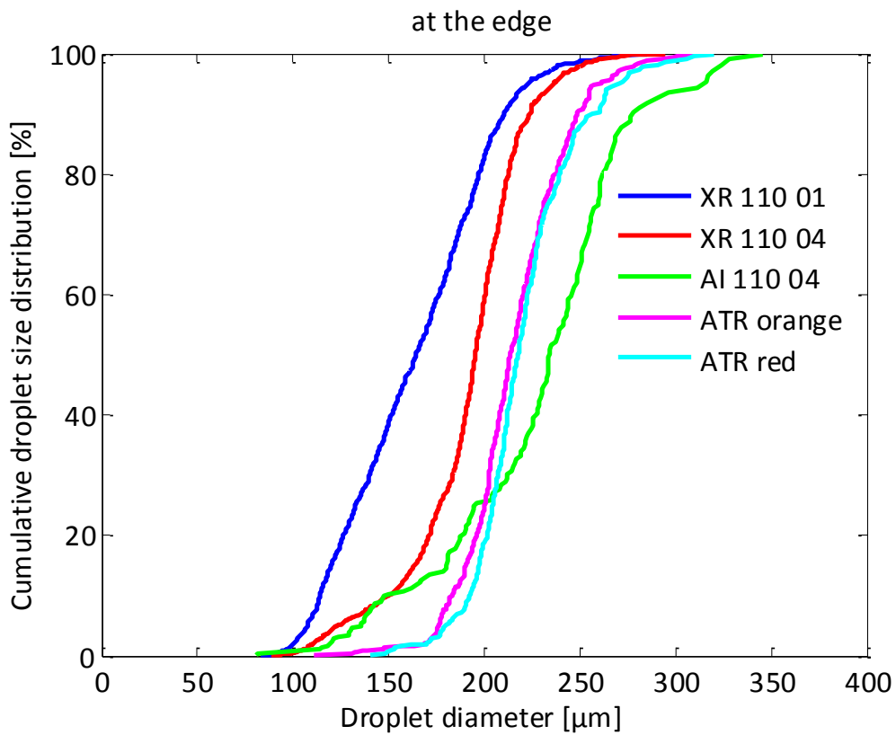
Figure 6.23. Effect of the nozzle type and size on the cumulative droplet size distribution at each measurement point
