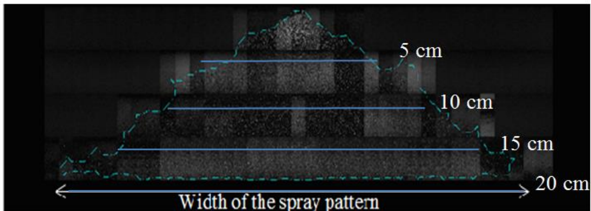
Figure 7.9. Spray shape analysis of the Tee Jet XR110 04 up to 20 cm below the nozzle
