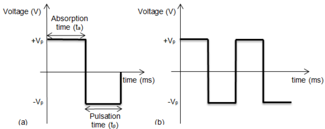
Figure 5.2. (a) Block diagram of the double pressure pulse for DOD mode and (b) continuous square signal for continuous mode
