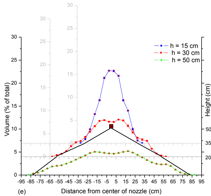
Figure 7.12. Spray angle and spray shape estimation based on spray distribution measurements at 3 different heights of the (a) Albuz ATR orange nozzle at 600 kPa, (b) Albuz ATR red at 800 kPa, (c) TeeJet XR 110 01 at 400 kPa, (d) TeeJet XR 110 04 at 400 kPa and (e) TeeJet AI 110 04 at 400 kPa
