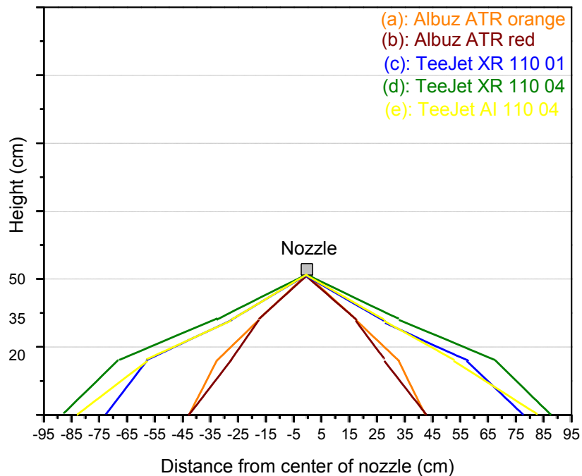
Figure 7.13. Spray angle as well as spray shape of the (a) Albuz ATR orange nozzle at 600 kPa; (b) Albuz ATR red at 800 kPa; (c) TeeJet XR 110 01 at 400 kPa; (d) TeeJet XR 110 04 at 400 kPa at 400 kPa and (e) TeeJet AI 110 04 at 400 kPa
