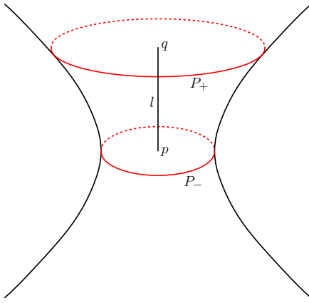
Figure 8.3: The setting of the proof of Proposition 8.B.
