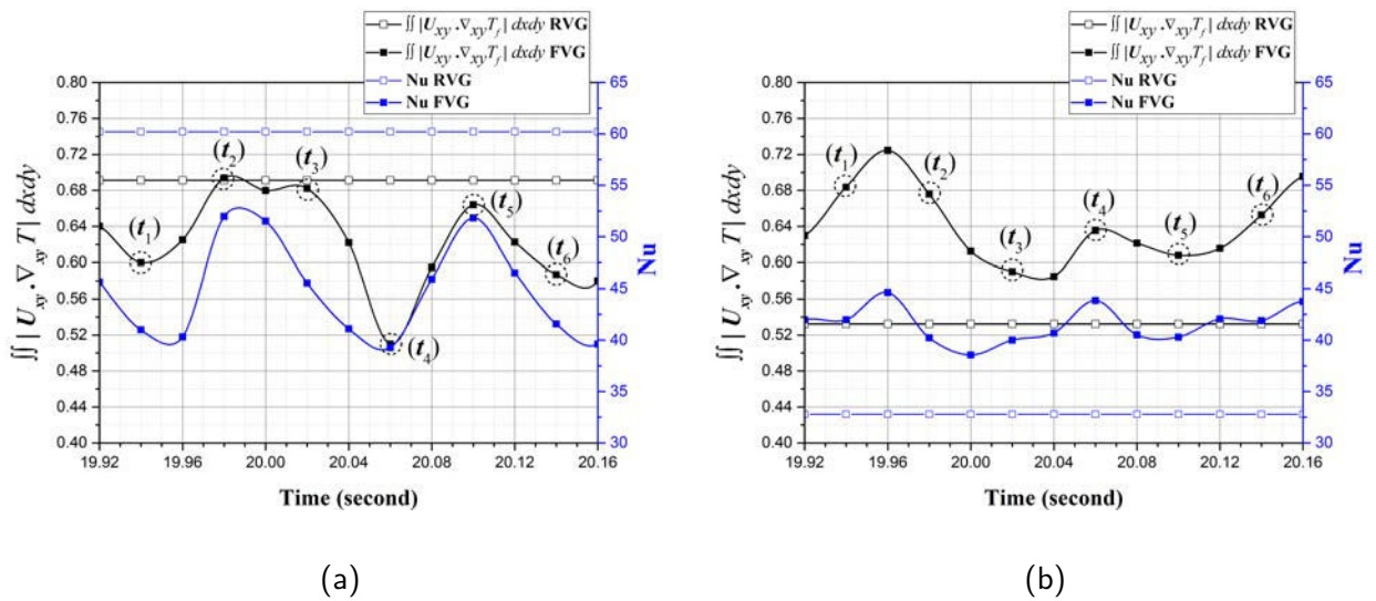
Figure 6.18: Time variation of local Nusselt number Nu_z and \iint |U_{xy} \cdot \nabla_{xy} T| dx dy during one period of oscillation for the FVG case at two different positions: (a) z/d = 1.96 (row C) and (b) z/d = 2.52 (row D). The RVG case is represented using constant lines with open symbols
