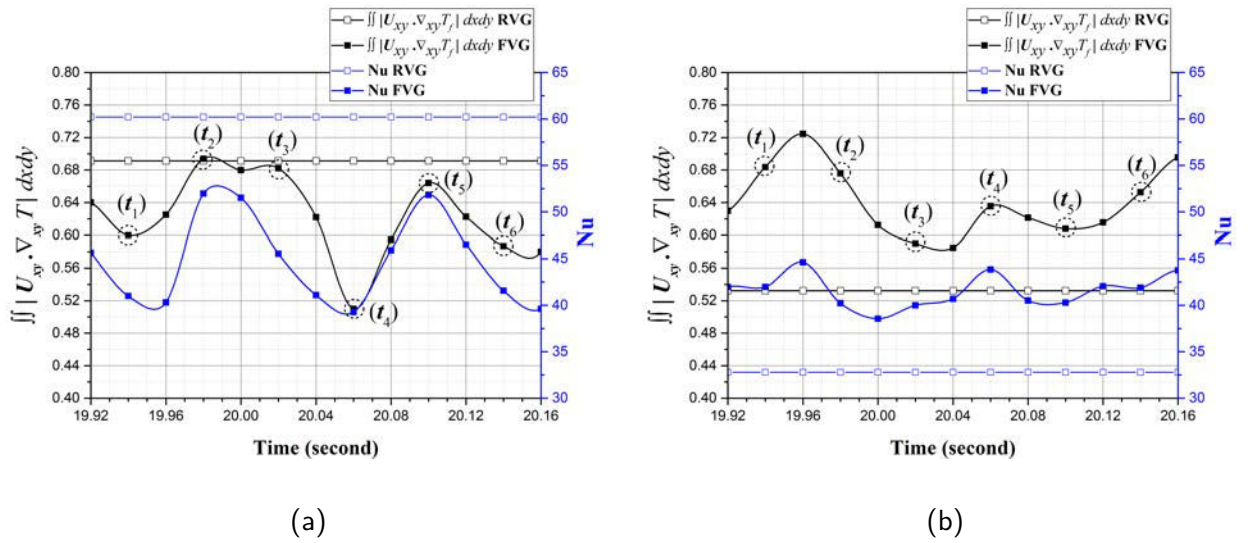
Figure 6.18: Time variation of local Nusselt number Nu_z and \oint |U_{xy} \cdot \nabla_{xy} T| dx dy during one period of oscillation for the FVG case at two different positions: (a) z/d = 1.96 (row C) and (b) z/d = 2.52 (row D). The RVG case is represented using constant lines with open symbols
