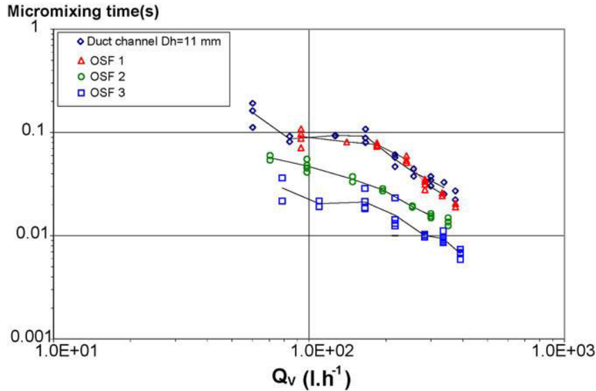
Figure 1.12: Micromixing time versus flow rate for three different offset strip fins (OSF) and a duct channel [Ferroillat et al., 2006]
