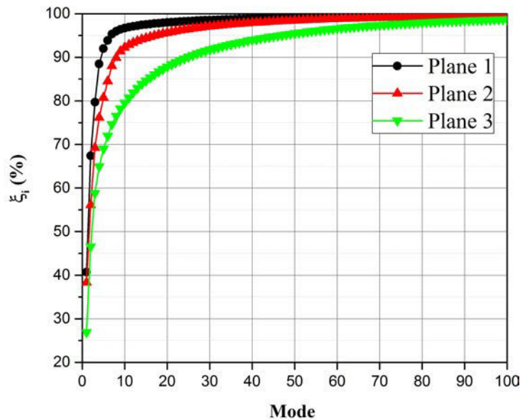
Figure 6.6: Cumulative energy content percentage \% \xi_i associated with POD modes 1-100 using all the 1500 available snapshots for each plane
