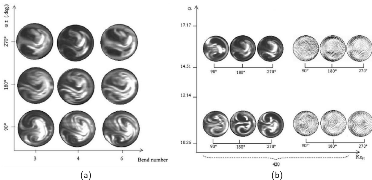
Figure 1.5: Experimental and numerical visualization of secondary flows for various: (a) bend number; (b) dimensionless frequency parameter \alpha [Timité et al. , 2011]
