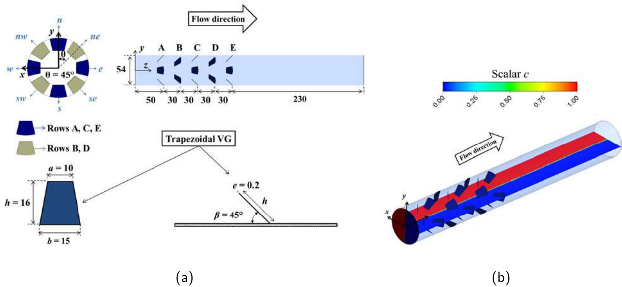
Figure 6.1: HEV geometry: (a) tab dimensions (in mm) and (b) Initial scalar field distribution in the fluid domain
