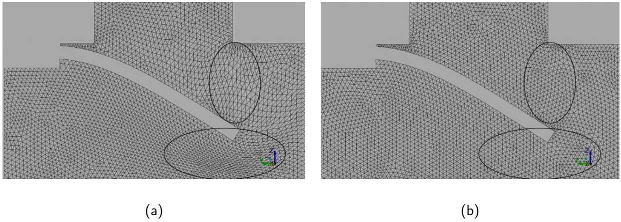
Figure 2.7: (a) zone before remeshing; (b) zone after remeshing [ANSYS, 2015]
