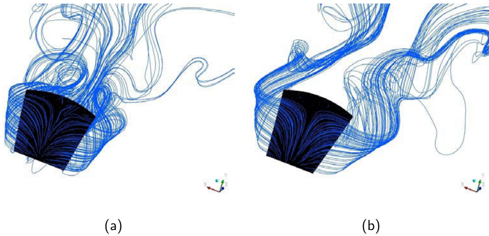
Figure 6.25: Streamlines around a tab En during two time instants: (a) t_1 and (b) t_3
