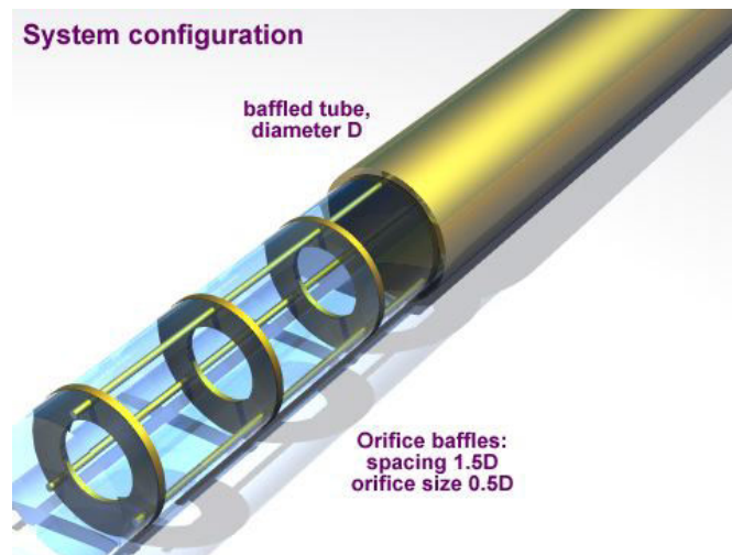
Figure 1.4: A 3-D schematic diagram of an oscillatory flow baffled tube [OFM Research Group, 2015]
