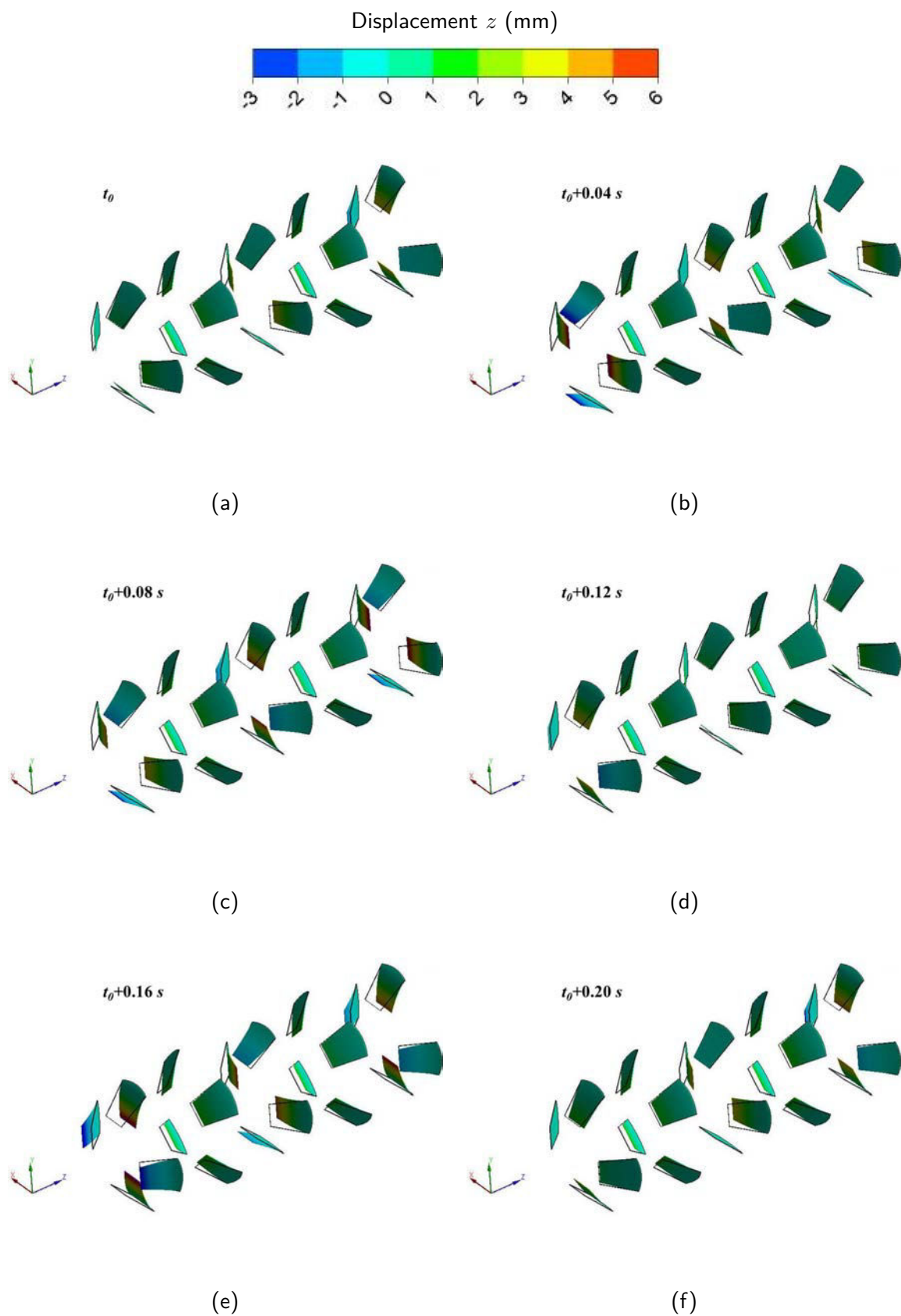
Figure 6.3: 3D perspective view of tabs deformations during one period of oscillation; the fixed wireframe represents the initial position of every tab
