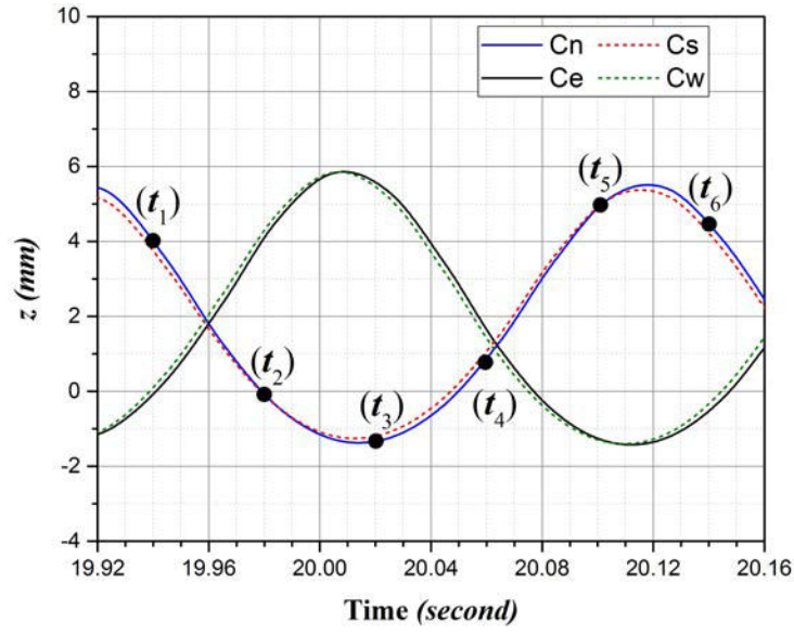
Figure 6.19: Displacement of tabs at row C in the z direction during one period of oscillation
