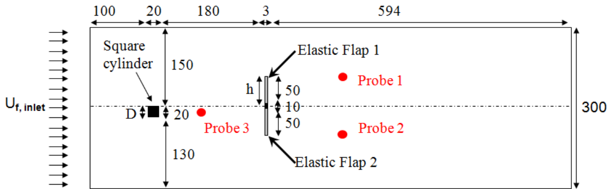
FIG. 1 - Schematic view of computational domain with mm as unit of length
