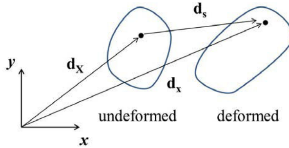
Figure 2.1: Motion of a deforming body
