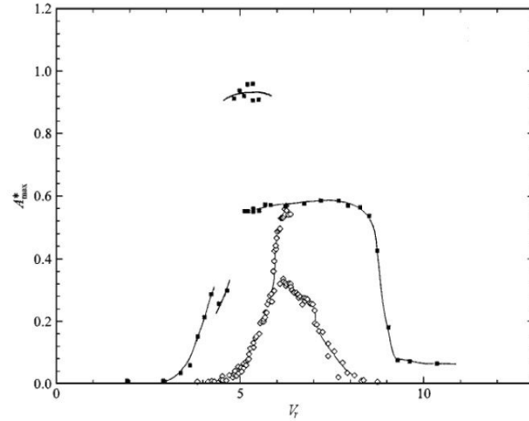
Figure 1.32: Amplitude of vibration in terms of cylinder diameter A_{max}^* as a function of reduced velocity V_r in VIV of cylinder with mass ratio m^* = 10.1 , ( \blacksquare Khalak and Williamson [Khalak and Williamson, 1999]), and m^* = 248 , ( \diamond Feng [Feng, 1968])
