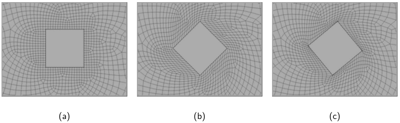
Figure 2.3: Comparison between spring-based and diffusion-based smoothing: (a) initial cube position; (b) cube rotated 45^\circ using diffusion-based smoothing and (c) using spring-based smoothing [ANSYS, 2015]
