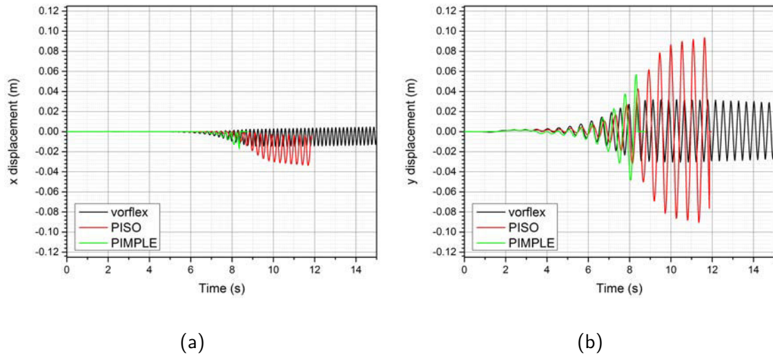
Figure A.1: Oscillation amplitudes as function of time. (a) x-displacement; (b) y-displacement
