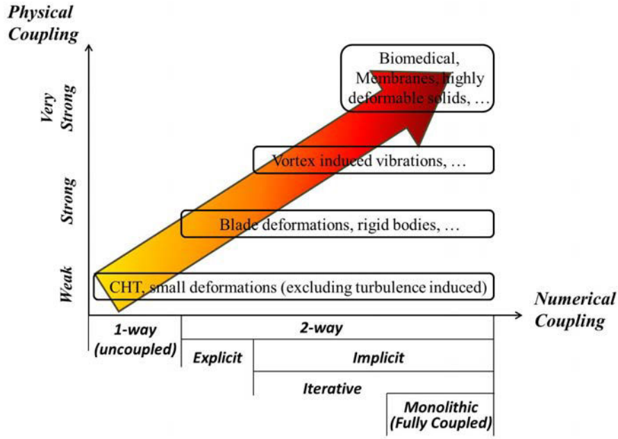
Figure 2.8: Modeling approaches for fluid-structure interaction problems
