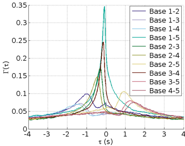
Fig. 15. Cross-correlation function \Gamma_{\alpha|\beta}(B_{i,j}, \tau) as a function of time \tau for each basis B_{i,j} using the five lasers beams of INTENSE .
