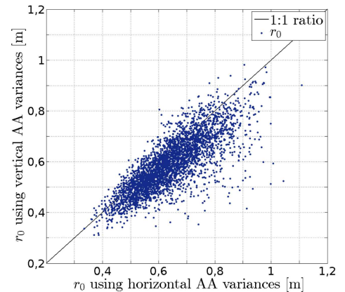
Fig. 3. r_0 distribution using horizontal and vertical AA differential variances in the weak turbulence case.
