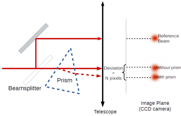
Fig. 7. Method for determining the angular resolution of the INTENSE instrument.
