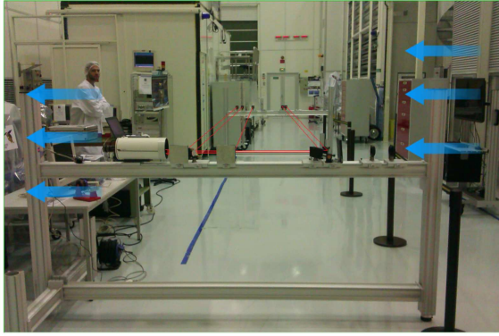
Fig. 4. The INTENSE instrument installed inside a Class 100000 clean room with strong laminar airflow.
