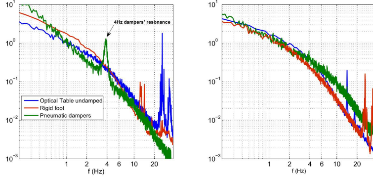
Figure 2. Examples of Power Density Spectra of A.A fluctuations. Top figure represents the PDS of a single spot A.A fluctuations when the benches are mounted on a undamped optical table (blue line), on rigid foot (red line) and on pneumatic dampers (green line).
