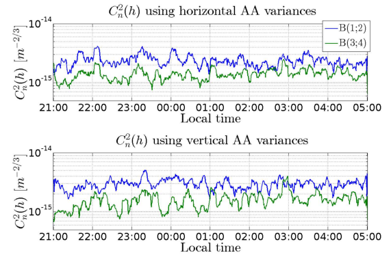
Fig. 14. Evolution of the C_n^2(h) in the closed vacuum chamber situation for two bases which are situated at each side of the INTENSE instrument.
