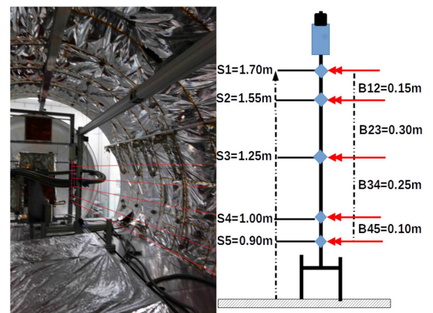
Fig. 15. The INTENSE instrument installed in the same Classe 100 room previously studied. The beams height and neighbouring bases size are shown on the right.
