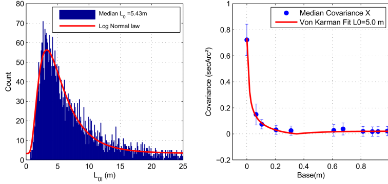
Figure 4. Outer scale of the turbulence L_0 under a strong turbulence condition. The left figure shows the histogram of the L_0 . The right figure shows the median longitudinal covariances of the A.A measured as a function of the bases.
