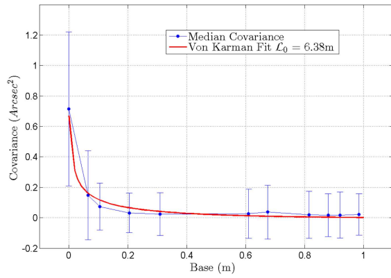
Fig. 14. Extraction of the outer scale \mathcal{L}_0 using median covariances under a strong turbulence. Each error bar is computed using the difference between the percentil at 75% and 25%.
