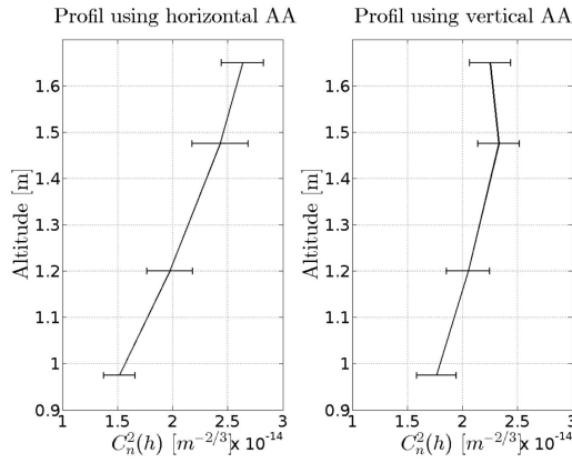
Fig. 19. C_n^2(h) profile in open room situation using mean and standard deviation for multiple bases.
