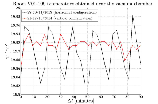
Fig. 17. Temperature measurements made in a room adjacent to the vacuum chamber during two acquisition periods using respectively the INTENSE instrument horizontal and vertical configuration.
