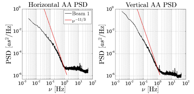
Fig. 25. PSD of AA fluctuations in the vacuum chamber with closed doors.
