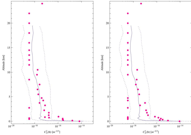
Fig. 7. Example of C_N^2 profile (dots) from PML at Dome C in Antarctica on January 25, 2011 at 16h45UT ( left panel ) and 17h17 ( right panel ). For comparison, the median profile (solid line) of radio-sounding balloons obtained during the 2005 winter campaign is plotted in solid line. Dotted lines indicate the 10% and 90% percentiles of the balloon data.
