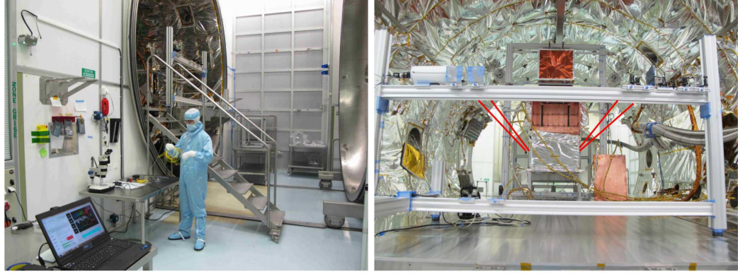
Figure 6. Left: View of the entrance of the testing chamber in the class 100 rated clean room. At the background, the fence of the particle regulation system where air blows out. Right: The INTENSE instrument installed testing chamber.
