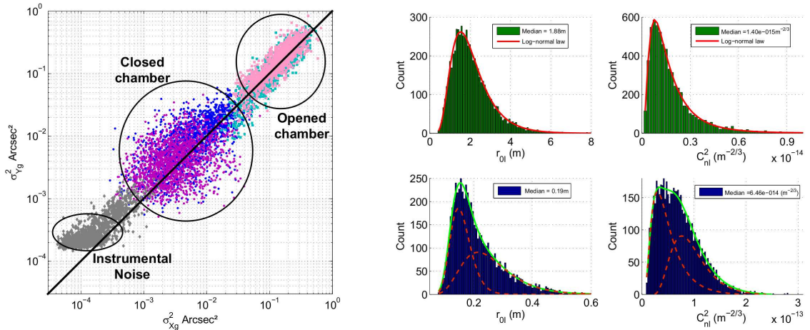
Figure 7. Left: Isotropy of the A.A inside the closed and opened chamber. For comparison, the instrumental noise was recorded with only few centimeter of laser propagation. Left: Histograms of the quantities of interest: r_{0l} and C_n^2 (from left to right) inside the closed (top) and opened (bottom) vacuum chamber .
