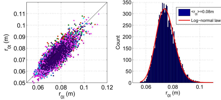
Figure 3. Statistics of the Fried's parameter r_0 under a strong turbulence condition. The left figure shows the isotropy of the r_0 measured along the longitudinal and transverse directions. The right figure shows the histogram of the longitudinal r_0 measured. The data fits well a log-normal law with a mean value \langle r_0 \rangle = 0.08\text{m} .
