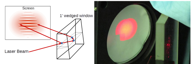
Fig. 6. Interference pattern obtained with the shearing interferometer.
