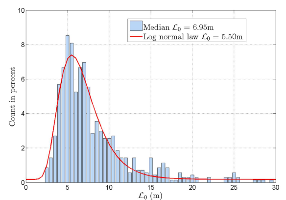
Fig. 13. Statistical analysis of the outer scale \mathcal{L}_0 along the longitudinal dimension under a strong turbulence condition using differential measurement of the r_0 (Fig. 12) and equation 12.
