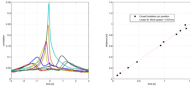
Figure 5. Left. Time cross-correlation of the A.A of the two spots separated by a base B . Right: Space ( B ) versus time position of maximum of the cross-correlation function. The fitted data gives an average wind speed of v_x = 0.67\text{m/s} .
