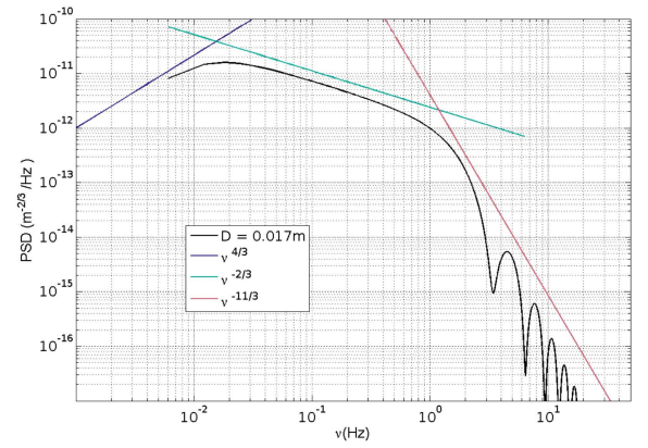
Fig. 2. Example of Temporal Power Spectrum Density of A.A. fluctuations using INTENSE laser beam diameter ( D = 0.017\text{m} ), an outer scale \mathcal{L}_0 = 5\text{m} , r_0 = 0.4\text{m} and a wind velocity \nu = 0.05\text{m/s} along the A.A. fluctuation direction.
