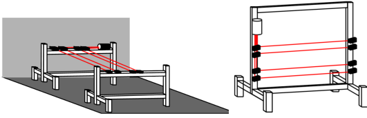
Fig. 3. Left: An horizontal version of the INTENSE instrument where emission and the reception of the laser beams can be separated by several meters on two different benches. Right: A vertical version of the INTENSE instrument on single bench.
