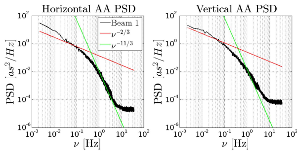
Fig. 13. PSD of AA fluctuations in the vacuum chamber in closed doors situation.
