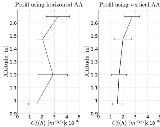
Fig. 24. C_n^2(h) profile in closed room situation using mean and standard deviation for multiple bases.
