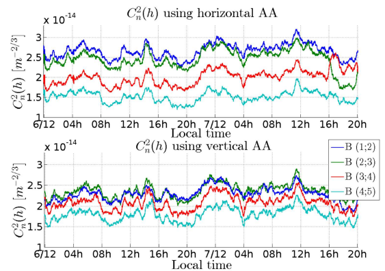
Fig. 18. Evolution of the C_n^2(h) with multiple base with different height.
