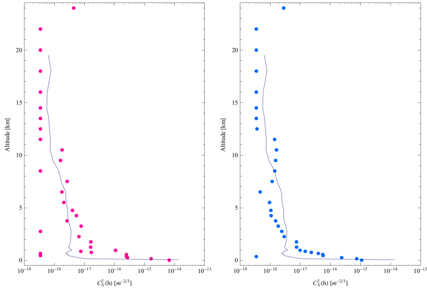
Fig. 4. Example of C_N^2 profile (dots) from PML at Dome C in Antarctica on January 25 and 26, 2011 at 16h45UT from Moon limb (left panel) and January 24, 2011 at 12h12UT from Sun limb (right panel). For comparison, the median profile of radio-sounding balloons obtained during the 2005 winter campaign is plotted in solid line.
