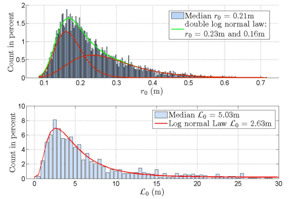
Fig. 17. Histograms of r_0 and \mathcal{L}_0 for the opened vacuum chamber.
