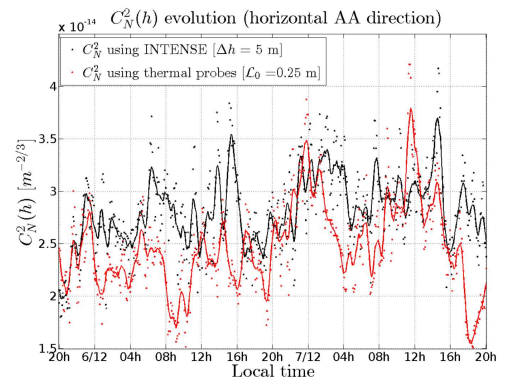
Fig. 21. C_N^2(h) comparison between AA measurements and temperature acquisitions in the same room. Marks represents raw-data of both estimations and smoothed curves are drawn for better visualization.
