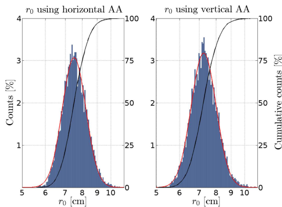
Fig. 5. r_0 histograms using AA differential variances obtained in the strong turbulence case.
