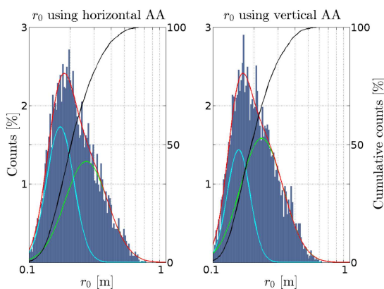
Fig. 9. r_0 histogram of the vacuum chamber in open situation with a two log-normal distribution fitting the results.
