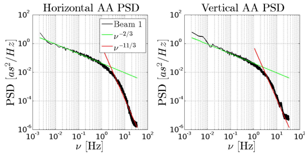
Fig. 12. PSD of AA fluctuations in the vacuum chamber in open doors situation.
