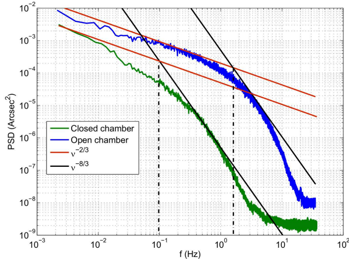
Figure 8. A.A fluctuations spectrum for closed (green) and opened chamber (blue). The two regimes in \nu^{-2/3} for intermediate frequencies and \nu^{-8/3} for high frequency are clearly visible.
