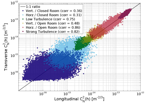
Fig. 9. Isotropy of all the C_n^2 measurements made at Thales Alenia Space Cannes.
