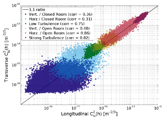
Fig. 27. Repartition of the C_N^2(h)h for each situation inside Thales Alenia Space clean rooms. C_N^2(h) named under Low Turbulence and Strong Turbulence are respectively from the Class 100000 SAS and the laminar ventilation systems room. Both Class 100 measurements with horizontal and vertical configuration were added.
