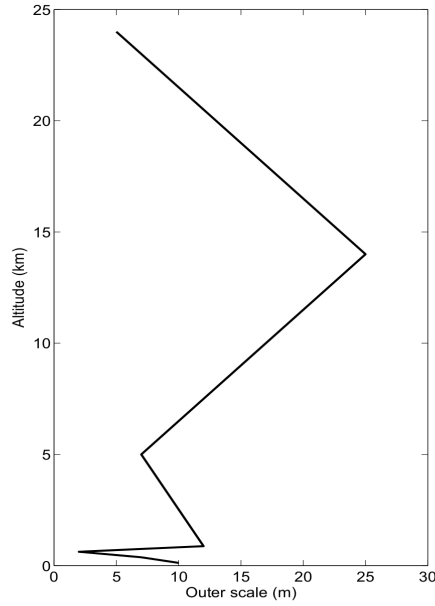
Fig. 5. Example of outer scale profile obtained with PML/PBL at Dome C in Antarctica on January 25, 2011 at 16h45UT from Moon limb.
