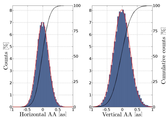
Fig. 2. AA histograms obtained in the SAS room using both horizontal and vertical directions.
