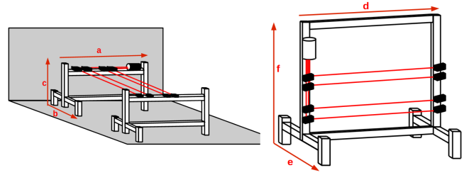
Fig. 1. The instrument in horizontal and vertical configuration respectively on the left and right.
