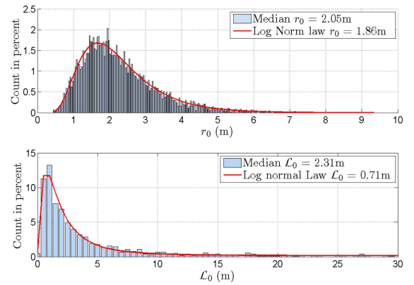
Fig. 18. Histograms of r_0 and \mathcal{L}_0 for the closed vacuum chamber.
