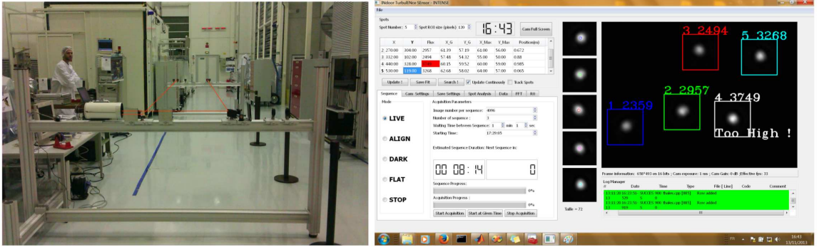
Figure 1. Left: Four or five laser beam are propagating through the local turbulence from an emitting bench at the background. Each beam is then reflected on the reception bench (at the foreground) toward a small telescope equipped with CCD camera. Right: User interface of the INTENSE instrument software.
