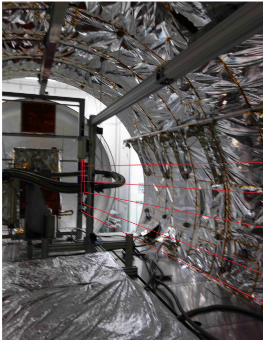
Fig. 10. The Intense instrument inside the cylindrical vacuum chamber at Thales Alenia Space Cannes.
