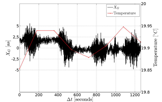
Fig. 11. Horizontal AA measured inside the vacuum chamber in open door situation and temperature measurements made in adjacent rooms (red line).
