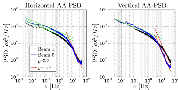
Fig. 20. PDS of AA fluctuations in the open room situation with two beams at the instrument minimal and maximal altitude ( S_5 = 0.90\text{m} and S_1 = 1.70\text{m} ).
