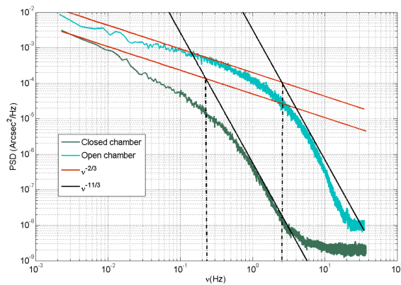
Fig. 19. A.A fluctuations spectrum for closed (green) and opened chamber (blue). The two regimes in \nu^{-2/3} for intermediate frequencies and \nu^{-11/3} for high frequency are clearly visible.
