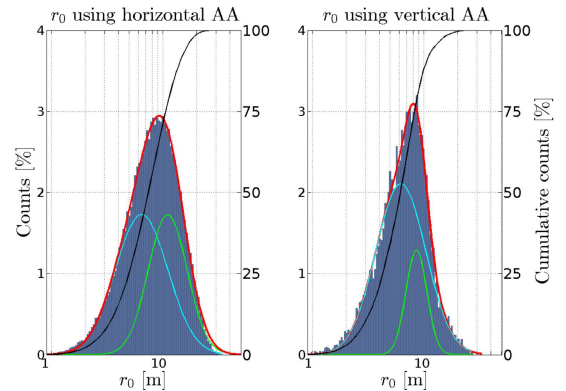
Fig. 22. r_0 histograms in the class 100 closed room using INTENSE vertical configuration.
