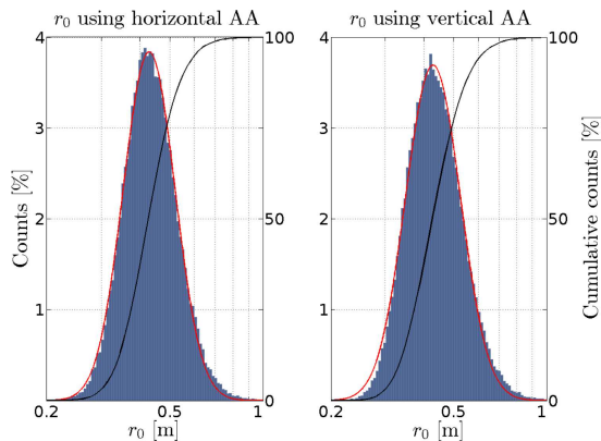
Fig. 16. r_0 histograms in the class 100 clean rooms using vertical configuration.
