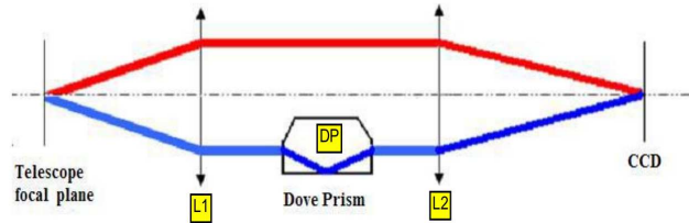
Fig. 2. The optical device in the focal plane of the PML/PBL instrument.
