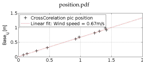
Fig. 16. Space-time position of the maximum of each cross-correlation function \Gamma_{\alpha|\beta}(B_{i,j}, \tau) .
