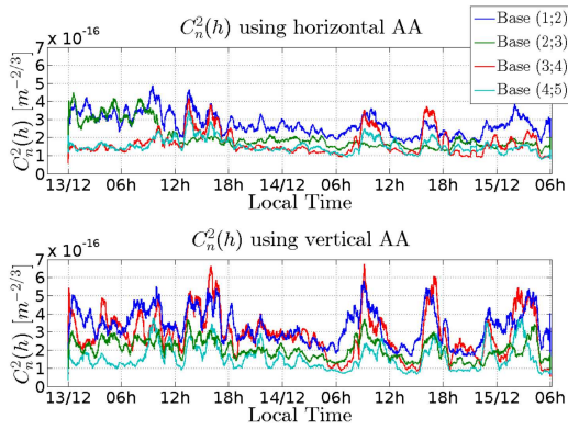
Fig. 23. Evolution of the C_N^2(h) during the acquisition. A transition period can be seen during the first 24 hour after the door were closed.
