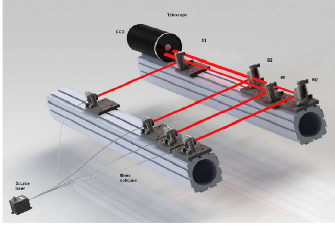
Fig. 1. Four or five laser beam are propagating through the local turbulence from an emitting bench at the foreground. Each beam is then reflected on the reception bench (at the background) toward a small telescope equipped with CCD camera.
