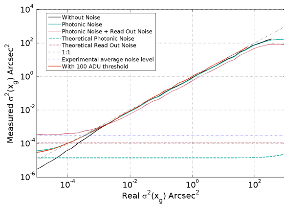
Fig. 4. Simulation of the barycentric measurement of the INTENSE instruments. For each point, N = 2048 realizations of a pure Airy Point Spread Function with a variance \sigma_{in}^2
