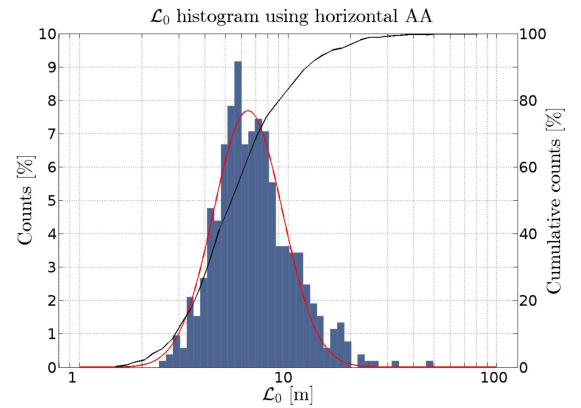
Fig. 6. \mathcal{L}_0 histogram using horizontal AA fluctuations in the strong turbulence case.
