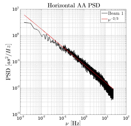
Fig. 7. PSD of AA fluctuations in horizontal direction for a strong turbulence case.
