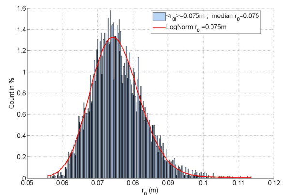
Fig. 12. Statistics of the Fried's parameter r_0 under a strong turbulence condition.
