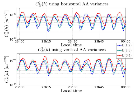
Fig. 10. Evolution of the C_N^2(h) in both horizontal and vertical direction during the open vacuum chamber case.
