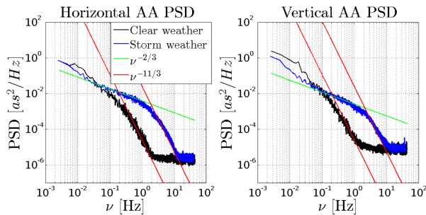
Fig. 26. AA PSD during two measurement periods. Both -2/3 and -11/3 are shown in order to fit the PSD.
