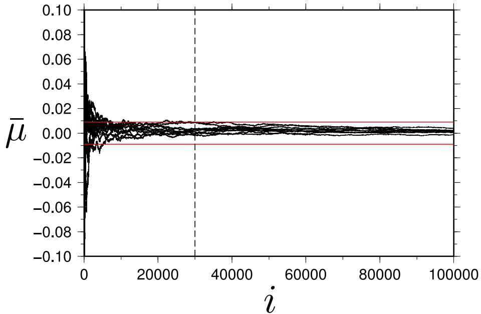
FIGURE 3.9 : Convergence test for \bar{\mu} in the case of a uniform distribution of instantaneous phases differences. The value of \bar{\mu} (équation 3.10) is plotted as a function of the number of instantaneous phase differences involved in the computation, given by i . The red lines indicate that the overall mean coherence \bar{\mu} reaches a value of 0 \pm 0.009 from 30 000 comparisons ( \simeq 245 instantaneous phases).
