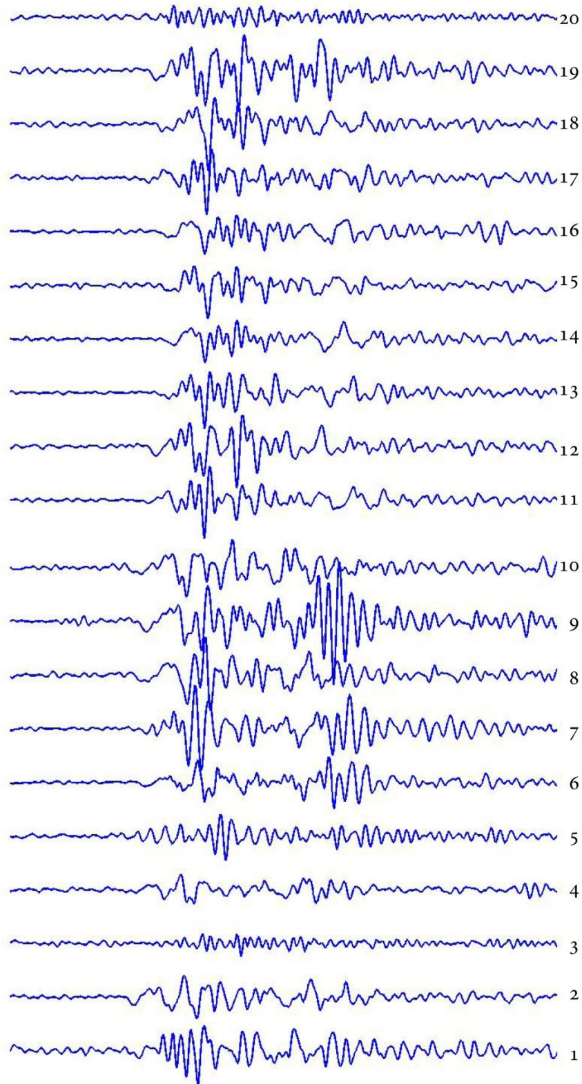
Figure 56 – Stack of velocity filtered (between 0.2 and 4 Hz) seismograms for ecpn station vertical component. The high frequencies make difficult to identify very similar events even if a certain degree of similarity between certain events is still recognizable. The event number is reported on the right.
