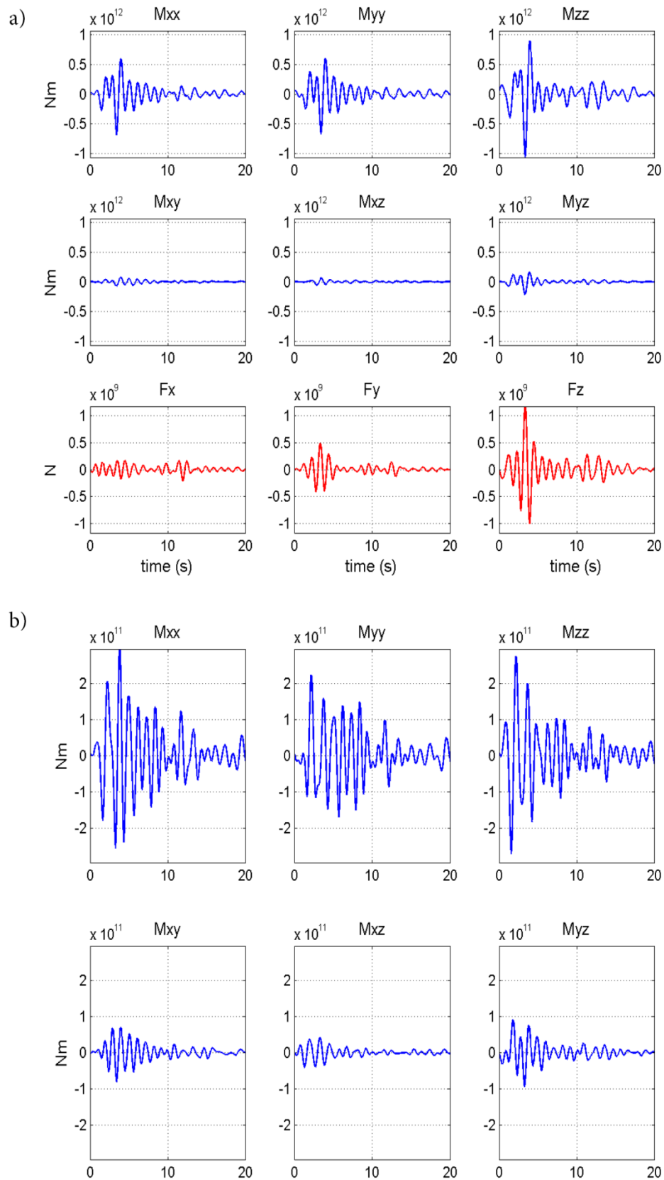
Figure 50 – a) MT inversion solution including forces for event 5 of the monochromatic set of events for the INGV source location and 14 stations of the INGV permanent network. b) MT inversion solution excluding forces for the same event.
