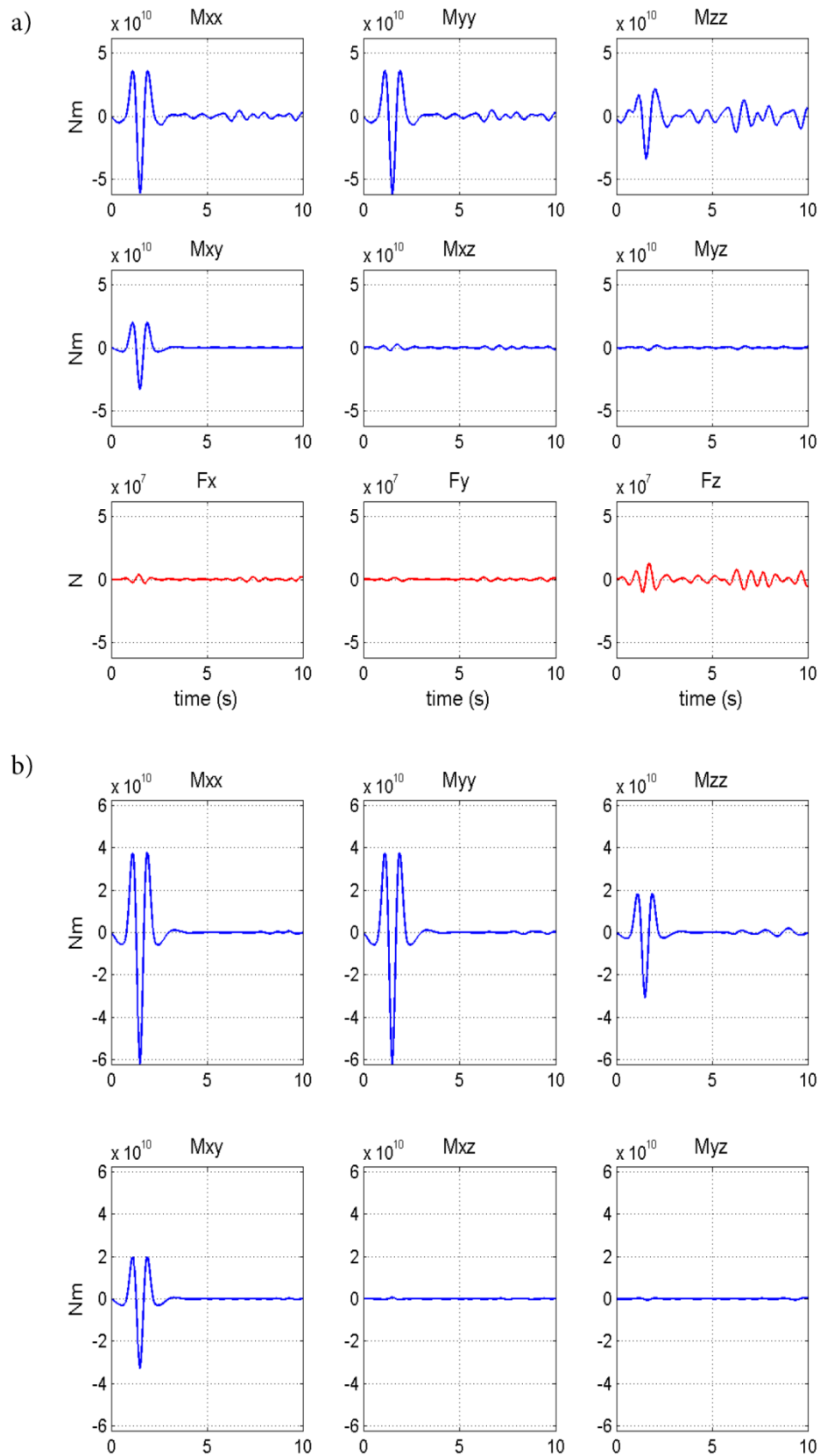
Figure 34 – a) MT inversion solution including forces for a shallow vertical crack and 14 stations of the INGV permanent network. b) MT inversion solution excluding forces for the same synthetic case as (a).
