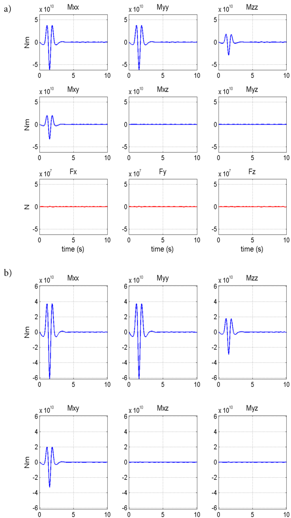
Figure 36 – a) MT inversion solution including forces for a deep vertical crack and 14 stations of the INGV permanent network. b) MT inversion solution excluding forces for the same synthetic case as (a).
