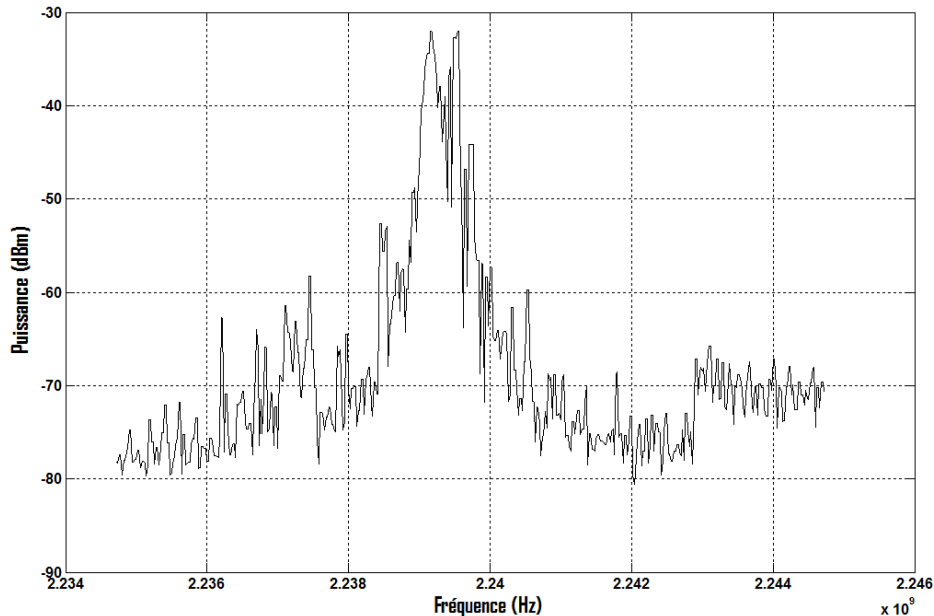
Figure 4.59. Spectre RF du MLLD perturbé
