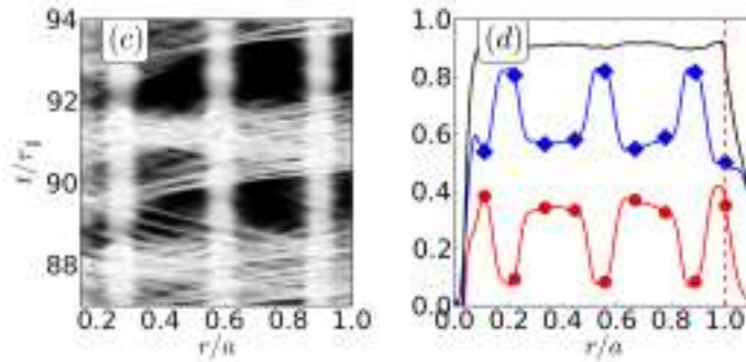
Figure 7.3: (c) parameter R_b used as figure of merit for the transport barriers (white corresponds to R_b = 1 , no barrier, black to R_b = 0 , barrier), (d) Radial flux profiles of total flux (black plain line), turbulent flux (blue line & diamonds) and diffusive flux (red line & circles)
