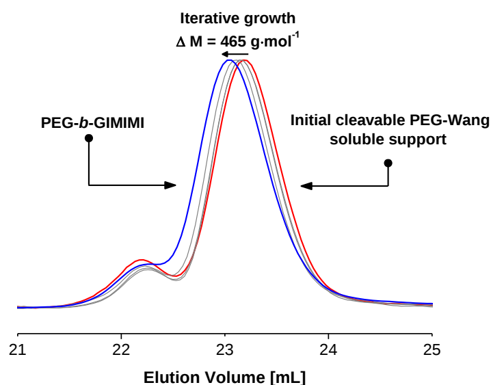
Figure 81. SEC chromatograms recorded in THF for a step-by-step growth of the poly(ethylene glycol)- b -pentamer conjugate performed on a cleavable soluble support (P9). The PEG Fmoc-protected support P9 is represented by a red line and the resulting (alkoxyamine amide)-polymer conjugate by a blue line. The grey traces show intermediate situations recorded after each bromoanhydride coupling.
