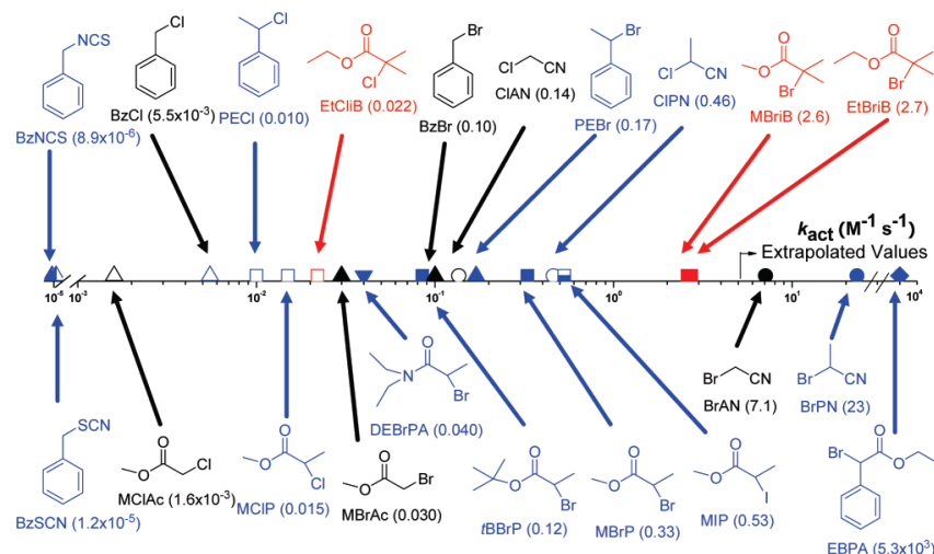
Figure 46. ATRP activation rate constants for various initiators with \text{Cu}^{\text{I}}\text{X}/\text{PMDETA} ( \text{X} = \text{Br} or \text{Cl} ) in MeCN at 35 °C: 3°, red; 2°, blue; 1°, black; isothiocyanate/thiocyanate, left half-filled; chloride, open; bromide, filled; iodide, bottom half-filled; amide, ▼; benzyl, ▲; ester, □; nitrile, ○; phenyl ester, ◇. Reprinted with permission from [193]. Copyright 2007 ACS.
