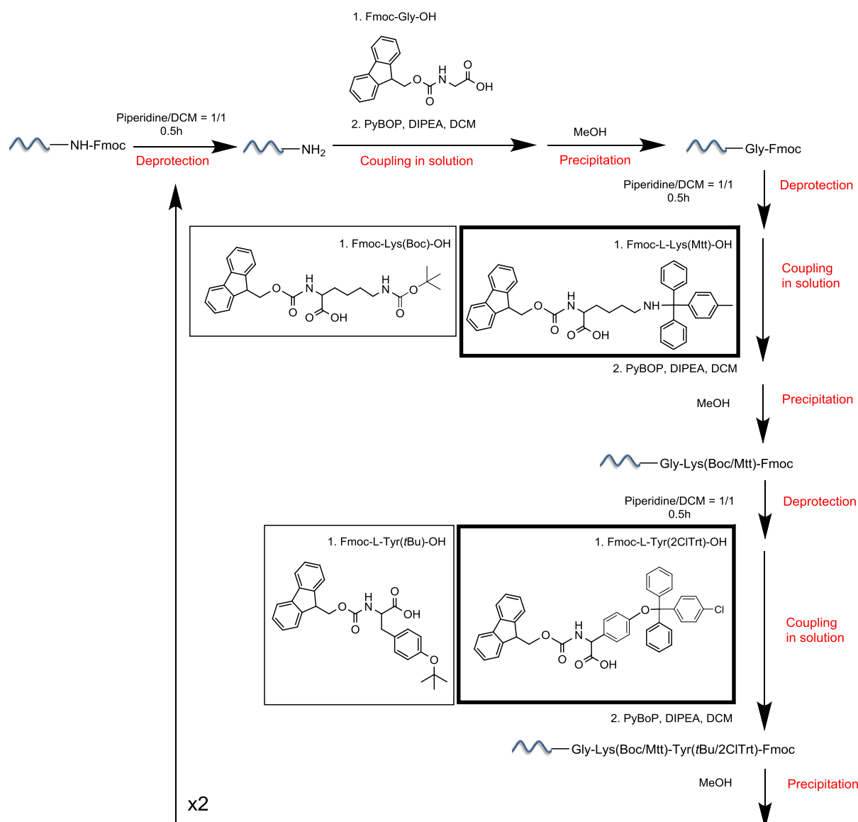
Scheme 16. Synthesis of -(\text{Gly-Lys-Tyr})_2 oligomer sequence on polystyrene soluble supports. Amino acid structures placed in bolded frames were bonded with the support containing a cleavable linker, as opposite to the oligopeptide containing Lys(Boc) and Tyr( t Bu) units that was synthesized on a non-cleavable support.
