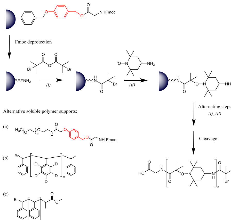
Scheme 17. Iterative approach to (alkoxyamine amide)s using a cleavable Wang solid support via alternating coupling of the monomers of AB and CD type (steps (i) and (ii), respectively). Alternative soluble polymer supports are displayed on the left. The iterative syntheses using supports (b) and (c) were performed via invers order of the alternating steps (i) and (ii).
