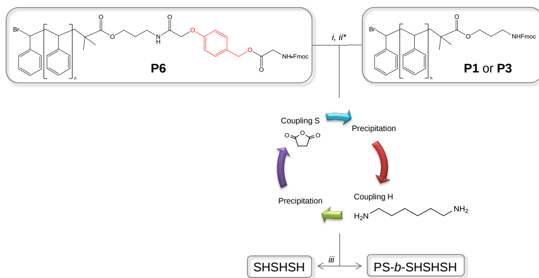
Scheme 21. Strategies examined for the synthesis of PS- b -PA conjugates. Terminal amine groups of polymers P1, P3 and P6 were deprotected prior to the assembly of the polyamide ( i ). Support P3 was additionally modified by treatment with TBAF to eliminate the bromide moiety at the end of the polymer chain ( ii ). After sequential coupling with succinic anhydride (S) and hexamethylenediamine (H) building blocks, the oligoamide was cleaved from the support under strong acidic conditions ( iii ).
