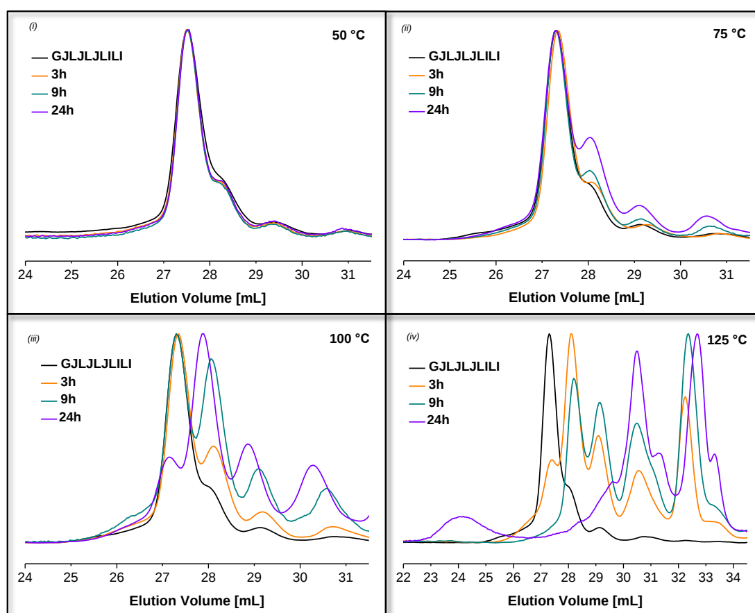
Figure 84. SEC chromatograms recorded in THF for the thermal degradation of the oligo(alkoxyamine amide) (GJLJLJLILI) in anisole (0.02 M) conducted at the following temperatures: (i) 50 °C, (ii) 75 °C, (iii) 100 °C and (iv) 125 °C. The black curve represents the initial dynamic polymer and the remaining curves correspond to the reorganized polymer after 3h, 9h and 24h (the orange, green and violet lines, respectively).
