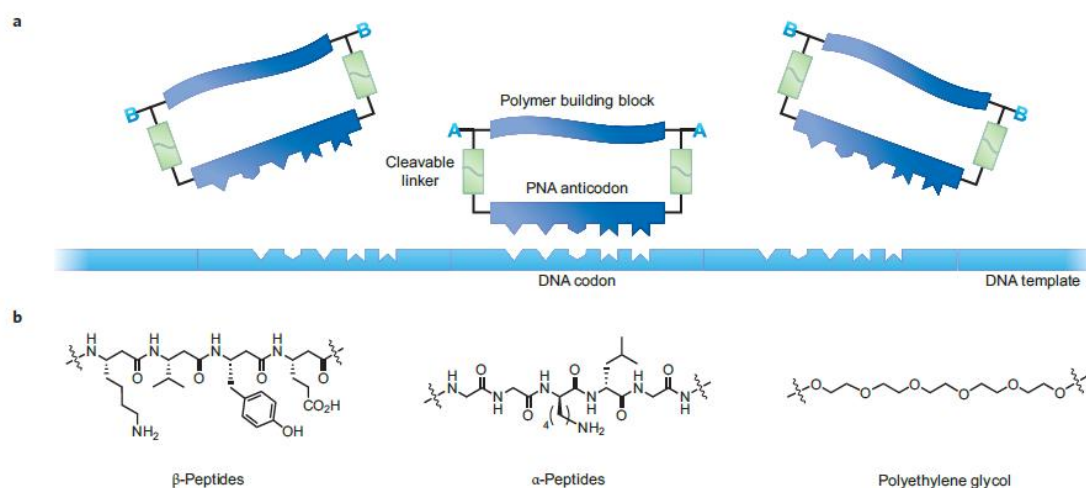
Figure 20. Sequence-controlled polymers prepared via macrocyclic building blocks with five-base-long PNA anticodons assembled on a DNA template and coupled through the reactive groups A and B ( a ). The bottom panel presents examples of polymer building blocks that can be stitched together to form sequence-defined materials using this approach. Reprinted by permission from Macmillan Publishers Ltd: Nature Chemistry,[53] copyright 2013.
