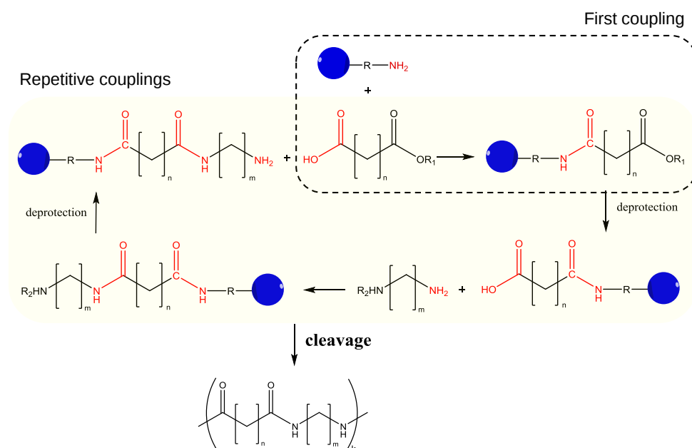
Scheme 20. Schematic representation of conventional solid-phase approach to polyamides formation using protecting groups. R 1 and R 2 are respectively protecting groups of the carboxyl and amine functions, while R represents a resin-bond chemical linker. Final polyamide structure is obtained after cleavage from the support with simultaneous removal of the protecting groups.
