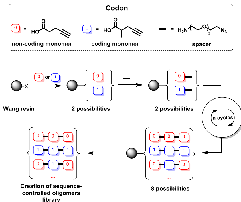
Figure 6. General strategy for synthesizing sequence-defined oligomers via an “AB + CD” iterative approach. Reprinted by permission from [23], © 2013 WILEY-VCH Verlag GmbH & Co. KGaA, Weinheim.
