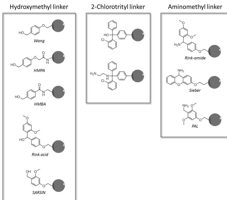
Figure 41. Variety of resin-bound linkers commonly used in solid phase synthesis.
