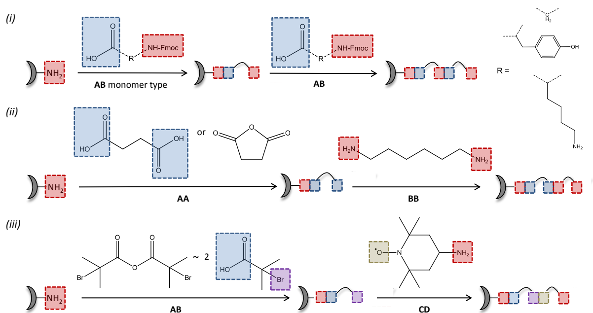
Figure 2. Sequence-controlled polymers prepared by iterative growth on a soluble/solid support via 3 different approaches of monomer coupling: (i) AB + AB, (ii) AA + BB and, (iii) AB + CD.
