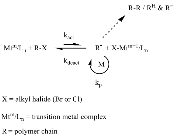
Scheme 7. Schematic representation of the ATRP mechanism.
