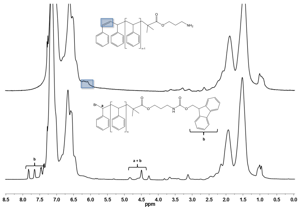
Figure 56. ^1\text{H} NMR spectra recorded in \text{CDCl}_3 for the polystyrene support prepared by ARGET ATRP technique from initiator 1 (bottom) and treated with TBAF (top).
