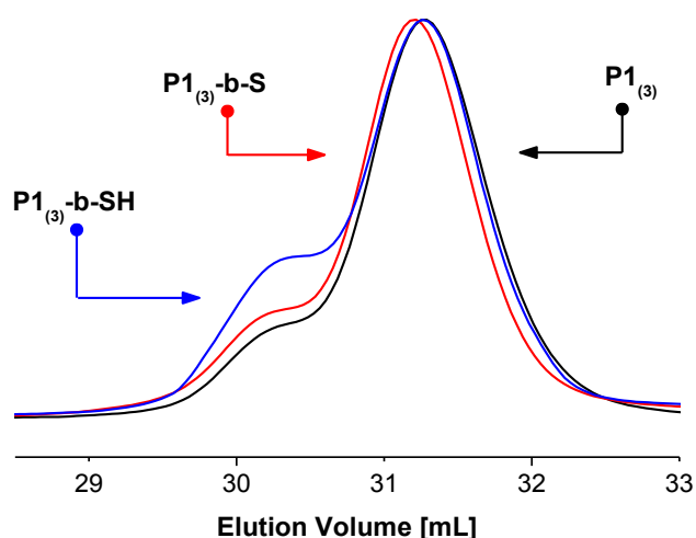
Figure 86. SEC chromatograms recorded in THF for the polystyrene permanent support P1 (3) (black curve) and two consecutive steps of the oligoamide iterative growth: (i) addition of succinic anhydride represented by a red curve, and (ii) addition of hexamethylenediamine represented by a blue curve.
