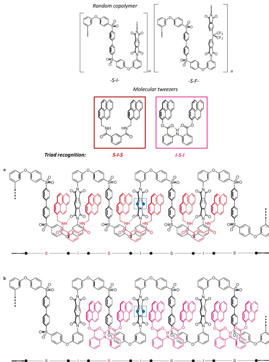
Figure 7. Visualisation of multiple binding to different polyimide triplet sequences by tweezer molecules ( a and b ). Constitution of a random copolymer prepared from S, I and F units is presented in the top panel and the structures of complementary molecular tweezers responsible for recognition of the triads S-I-S and I-S-I is displayed below. Preference for the S-I-S pattern has been revealed by the tweezers containing the 3-aminophenoxy residue (red), while the I-S-I sequence was binded to the intramolecularly hydrogen-bonded diester tweezers (magenta). Reprinted by permission from Macmillan Publishers Ltd: Nature Chemistry,[25] copyright 2010.
