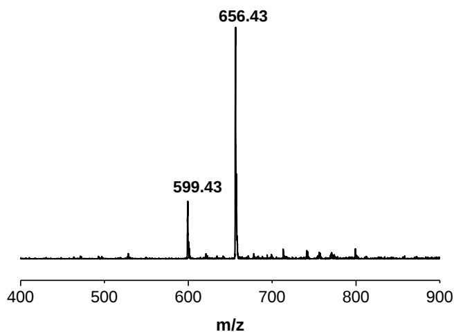
Figure 67. Negative mode ESI-MS of Gly-Lys-Tyr-Lys-Tyr molecule cleaved from P5 (2) -b-Gly-Lys(Boc)-Tyr( t Bu)-Lys(Boc)-Tyr( t Bu) polymer conjugate (protection groups removed simultaneously).
