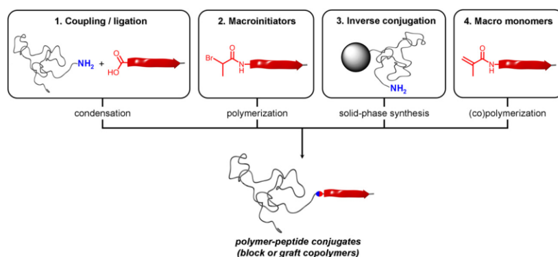
Scheme 10. Graphic illustration of the principal approaches towards polymer bioconjugates: (1) coupling of peptide segments to preformed polymer blocks using one or multiple reactive sites, (2) “grafting from” approach: growth of polymer block from the peptide segment, (3) sequential assembling of the peptide on a preformed synthetic polymer, (4) polymerization of short peptide segments that possess a polymerizable functionality. Reprinted with permission from [228]. Copyright 2013 ACS.
