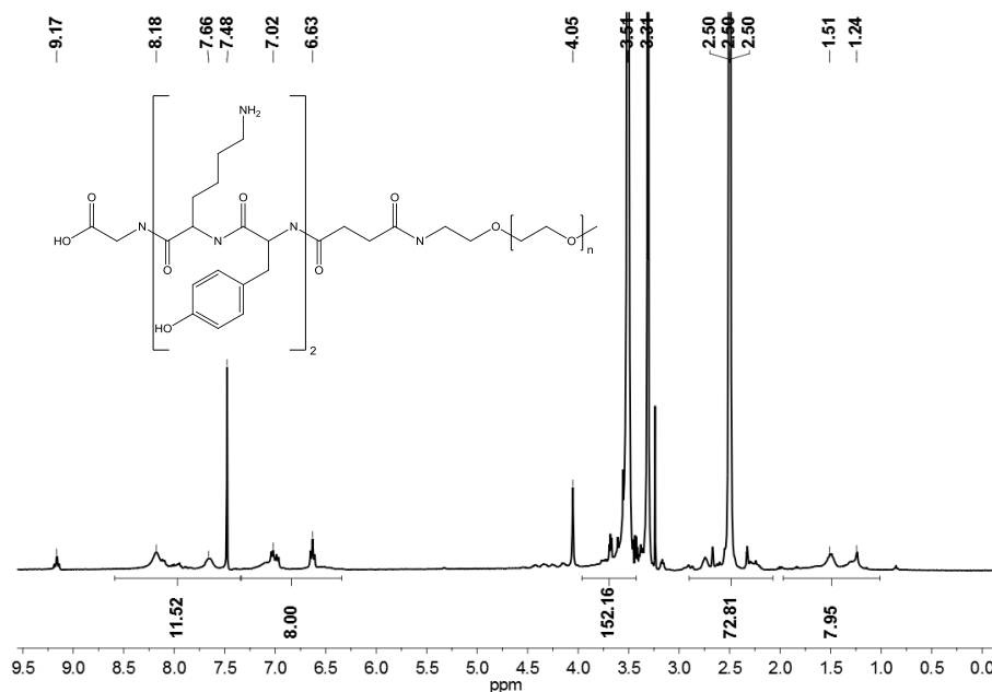
Figure 70. 1 H NMR spectrum recorded in CDCl 3 for MeO-PEG5k-Tyr-Lys-Tyr-Lys-Gly-COOH synthesized on PS soluble support P5 (2) .
