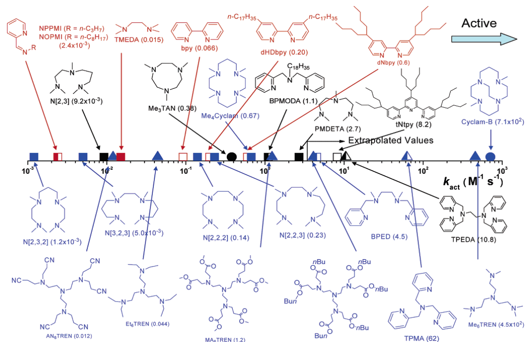
Figure 48. ATRP activation rate constants for various ligands with ethyl 2-bromoisobutyrate in the presence of Cu 1 X (X = Br or Cl) in MeCN at 35 °C: N2, red; N3, black; N4, blue; amine/imine, solid; pyridine, open; mixed, left-half solid; linear, □; branched, ▲; cyclic, ○. Reprinted with permission from [201]. Copyright 2006 ACS.
