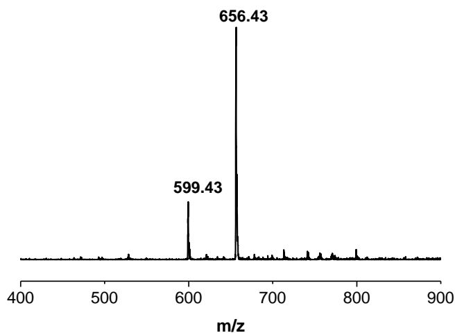
Figure 67. Negative mode ESI-MS of Gly-Lys-Tyr-Lys-Tyr molecule cleaved from P5_{(2)}\text{-}b\text{-Gly-Lys(Boc)-Tyr}(t\text{Bu})\text{-Lys(Boc)-Tyr}(t\text{Bu}) polymer conjugate (protection groups removed simultaneously).
