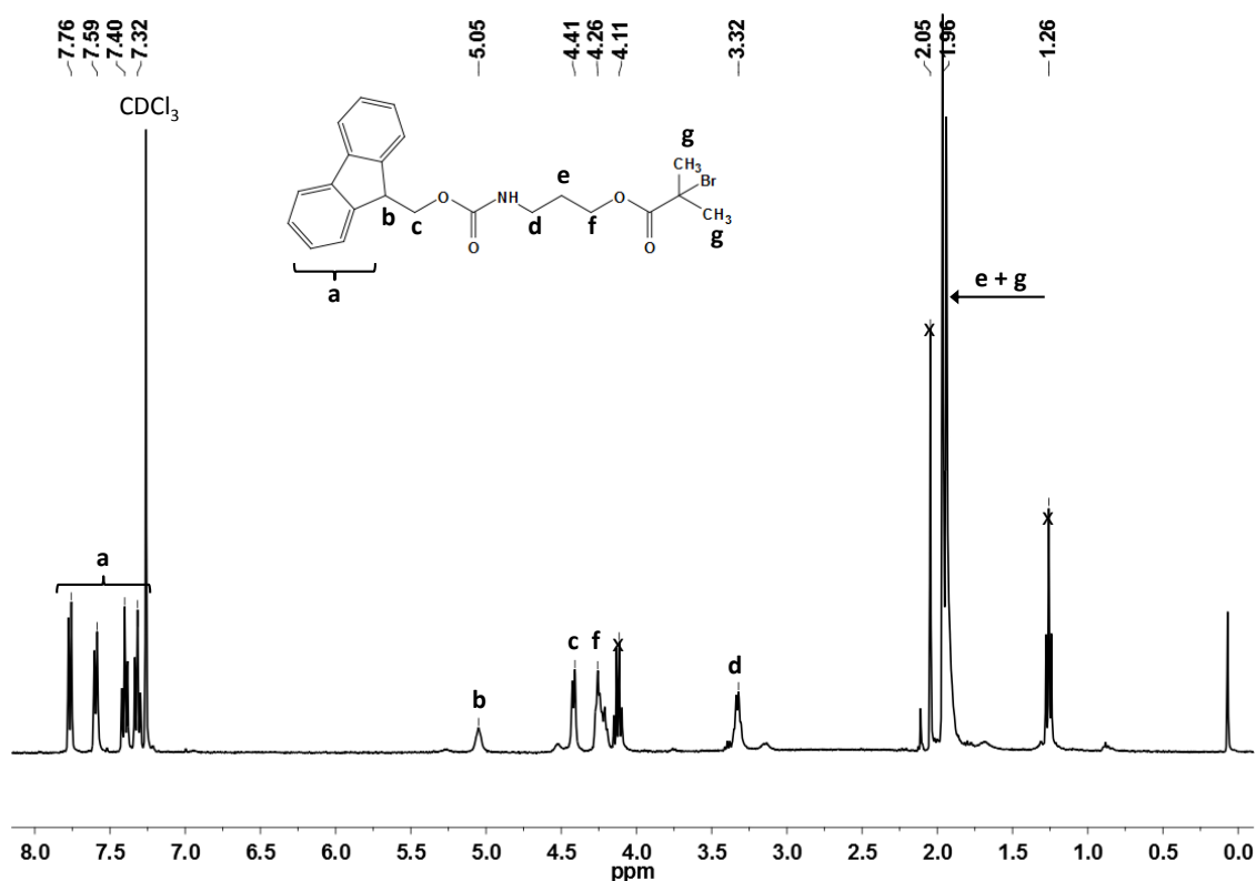
Figure 49. ^1\text{H} NMR spectrum recorded in \text{CDCl}_3 for the ATRP initiator 1 .
