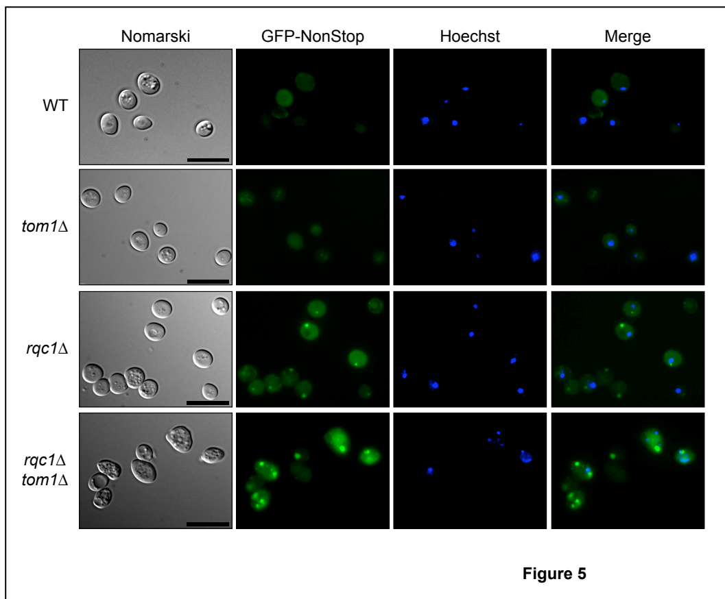
Fig. 5 The absence of Tom1 leads to increased aggregation of the GFP-NS when Rqc1 is defective WT, tom1Δ , rqc1Δ or rqc1Δtom1Δ strains expressing the GFP-NS reporter gene were analyzed by fluorescence microscopy. Yeast cells are displayed in left column (Nomarski) GFP and Hoechst fluorescent signals are displayed in middle columns and merged in the right column. Scale bar = 15μm.
