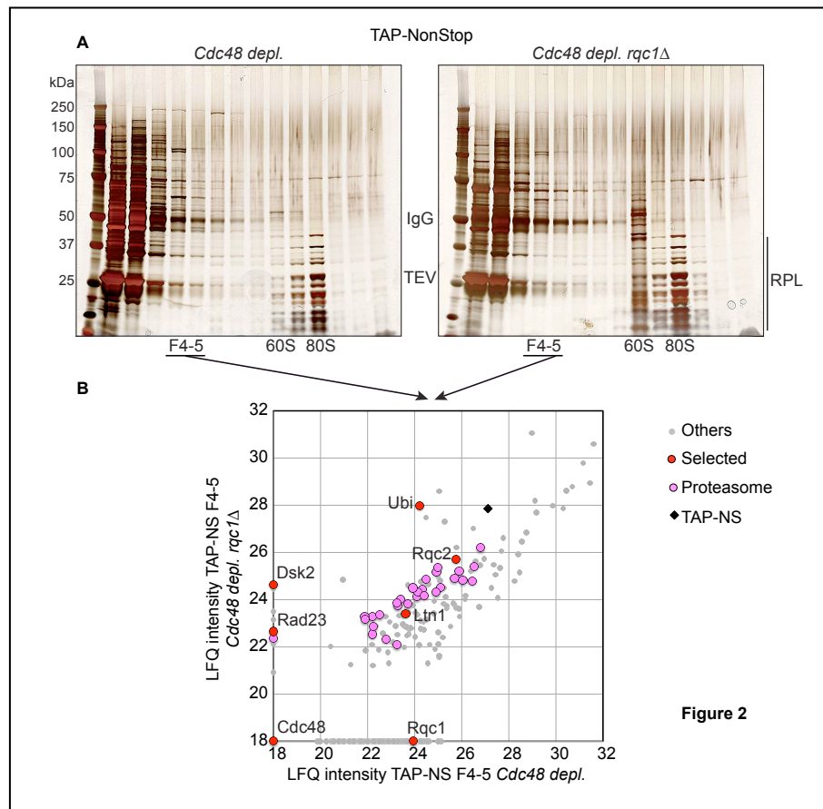
Fig. 2 The RQC complex remains associated to the aberrant nascent peptides during their escort to the proteasome
