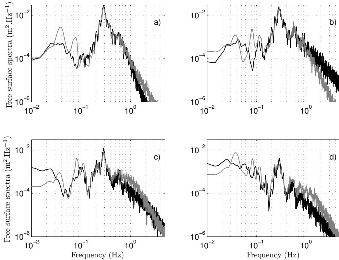
Figure 4.19 – Free surface wave spectra S_{\eta\eta} of experimental wave gauges for experiment 30 ( t=21:00-26:00 ) (grey line) and of the numerical model (black line) at distances (a) x = 5.01\text{m} , (b) x = 10.31\text{m} , (c) x = 15.31\text{m} , (d) x = 20.34\text{m} , from the wavemaker. The alongshore distance is y = 15\text{m} , at the center of the basin.
