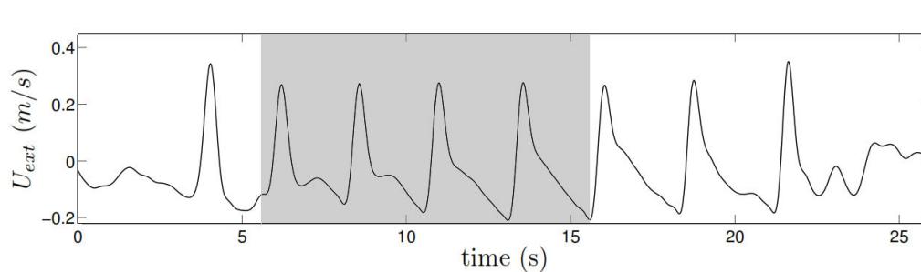
Figure 3: Free stream velocity. Phase averaged velocity records of the 2.5 s wave packet at the cross-shore position x = 13 m and at an elevation of z = 3.6 cm above the mean bed elevation. The grey-tinted box bounds the waves used in the analysis.
