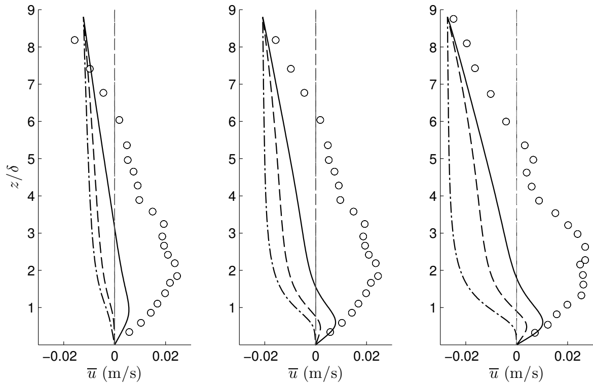
Figure 2.20 – Comparison of mean velocity profiles at gauges P4 (left panel), P8 (middle panel) and P10 (right panel). (o): Lin et Hwung [2002] experimental results; ( -\cdot- ): k-\omega model without the mean pressure gradient; ( --- ): k-\omega model with the mean pressure gradient; ( - ): k-\omega model with the mean pressure gradient and the advection terms.
