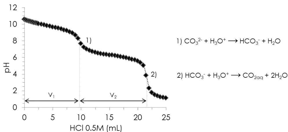
Figure 21. Titration curve of geopolymer pore solution extracted after 3 days cured at 20°C, 50% R.H. and 50% of CO 2 by a 0.5M HCl solution followed by pH.
