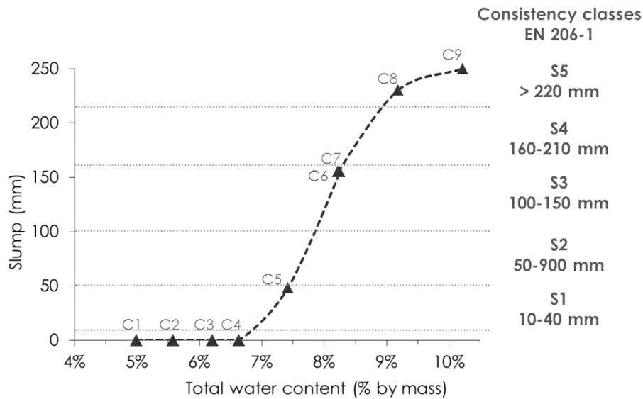
Figure 13. Slump versus total amount of water in geopolymer concretes C1 to C9, with consistency classes according to EN206-1.
