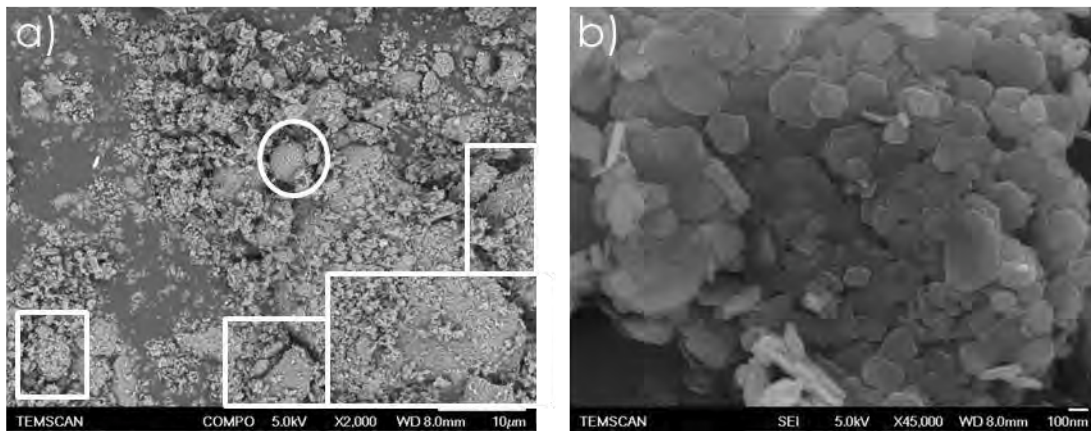
Figure 10. Photomicrograph of flash-metakaolin obtained at two different scales a) x 2,000 and b) x 45,000. □ corresponds to the quartz and ○ to the spherical particles.
