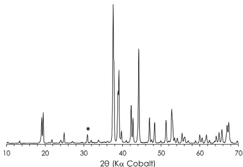
Figure 28. XRD pattern of efflorescence formed under natural \text{CO}_2 environment at 20^\circ\text{C} and 50% R.H. All the peaks were identified as \text{Na}_2\text{CO}_3 \cdot \text{H}_2\text{O} (PDF # 08-0448) except for a quartz peak noted (*).
