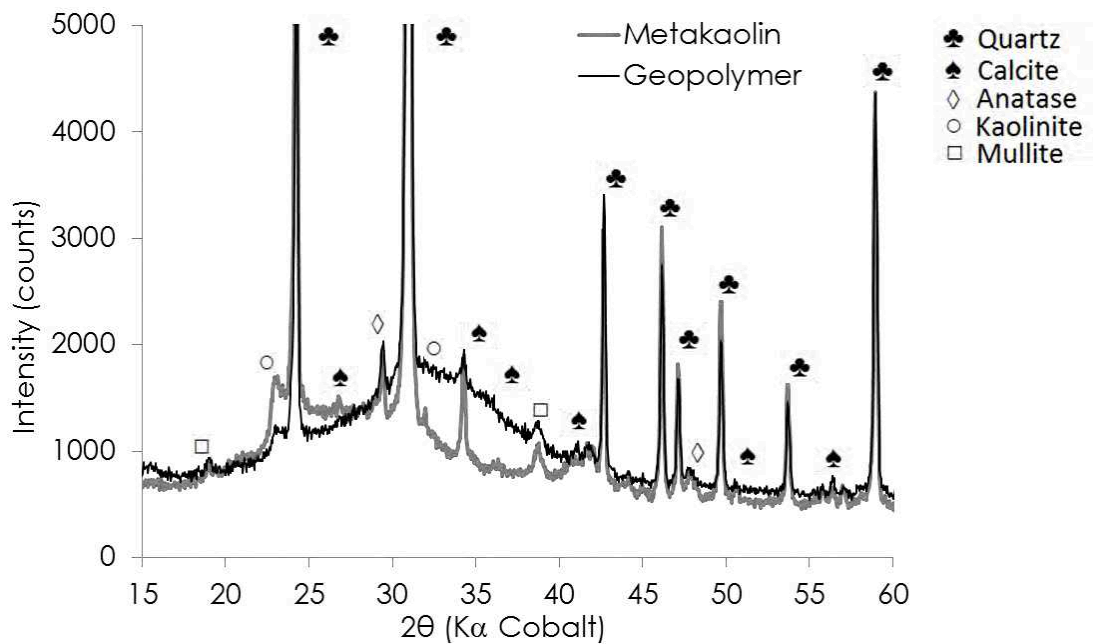
Figure 30. XRD pattern of flash-calcined metakaolin and pure geopolymer GP14.5.
