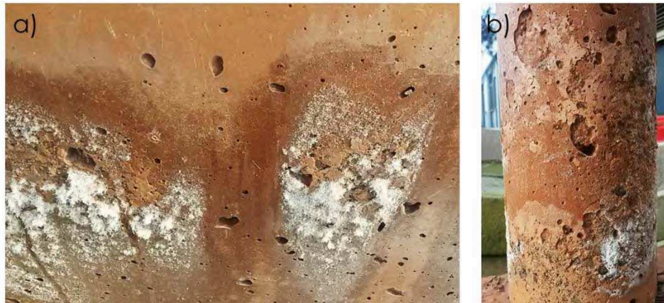
Figure 24. Visual observation of the sides of a) the beam and b) cylinder stored outside.
