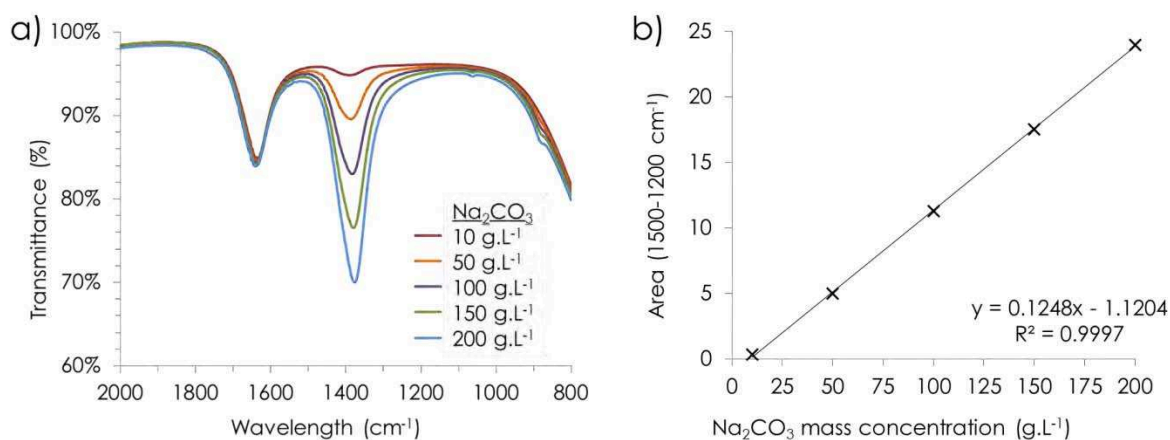
Figure 18. a) FTIR spectra of pure Na 2 CO 3 solutions having mass concentrations of 10, 50, 100, 150, and 200 g.L -1 between 2000 cm -1 and 800 cm -1 and b) Calibration curve of the area of the carbonate vibrations between 1500 and 1200 cm -1 , plotted versus the mass concentration of the references.
