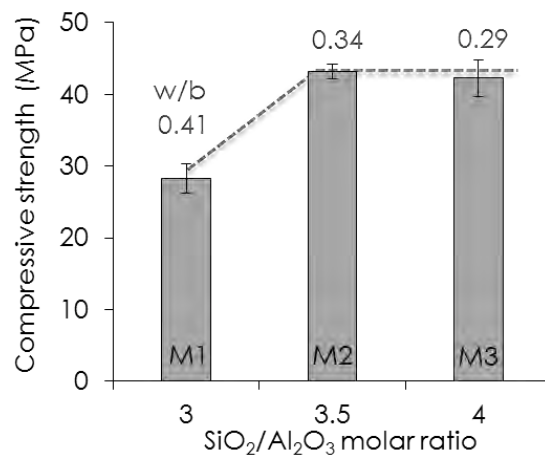
Figure 15. Compressive strength of geopolymer mortars with different SiO 2 /Al 2 O 3 molar ratios at 7 days, with the water/binder ratios.
