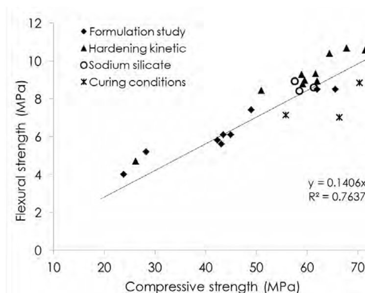
Figure 25. Flexural versus compressive strength of all the geopolymer mortars.
