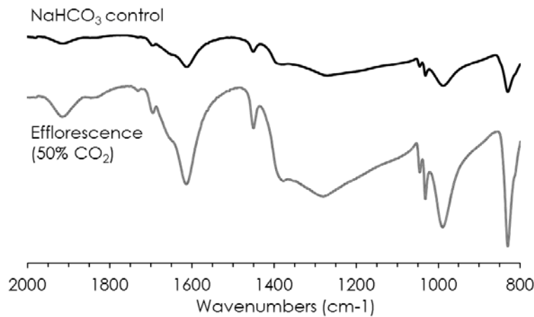
Figure 31. Infrared spectra of pure \text{NaHCO}_3 crystals and efflorescence residues collected on geopolymer paste cured at 50% of \text{CO}_2 (20°C and 50% R.H.).
