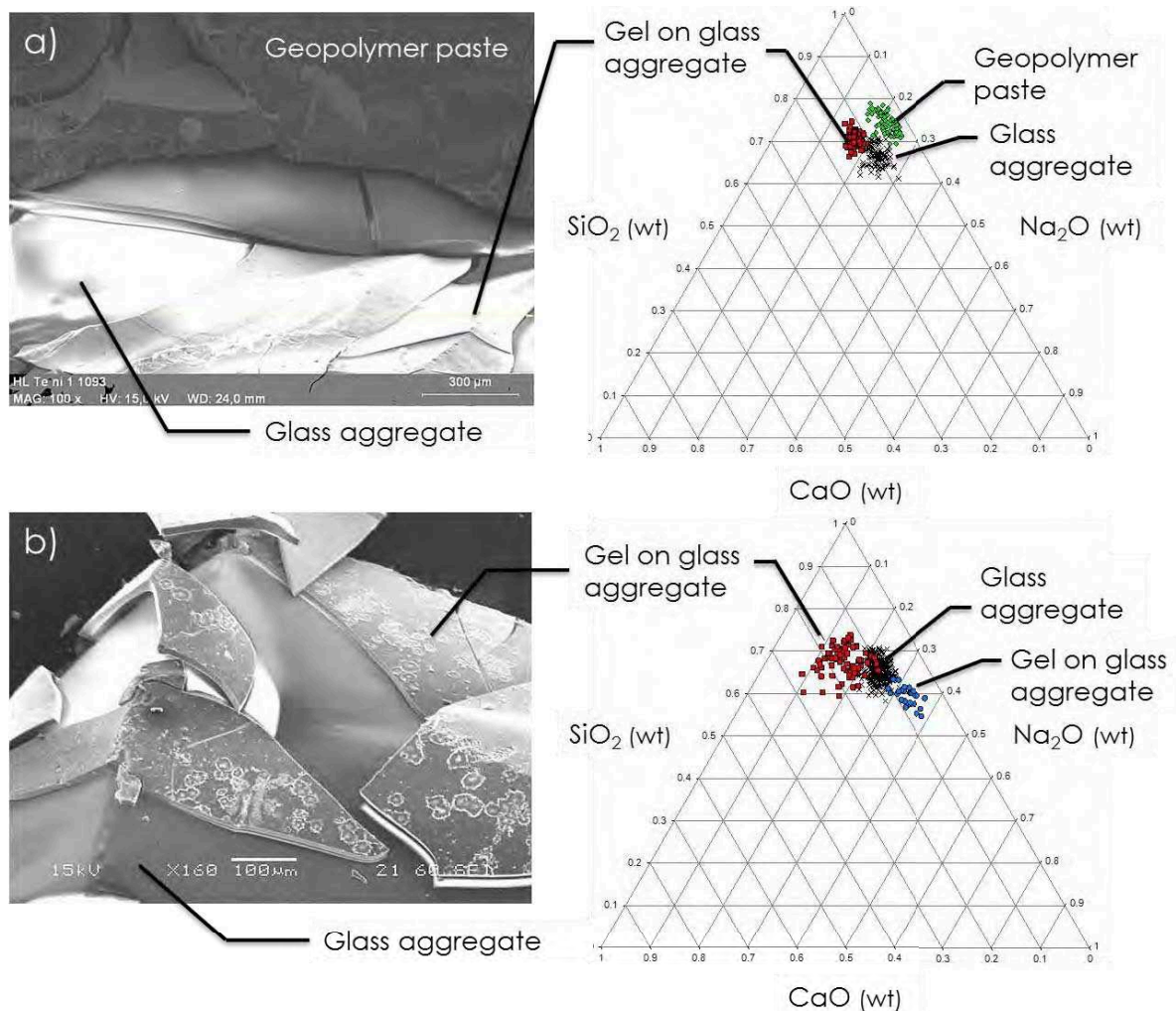
Figure 13. Photomicrograph and Energy Dispersive X-ray spectrometry (ternary diagram \text{SiO}_2\text{-CaO-Na}_2\text{O} in % weight) for (a) paste-aggregate interface of GP-f mortar and (b) glass aggregate detached from GP-f mortar.
