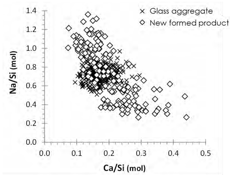
Figure 14. Composition of new-formed products around glass particles in geopolymer mortar.
