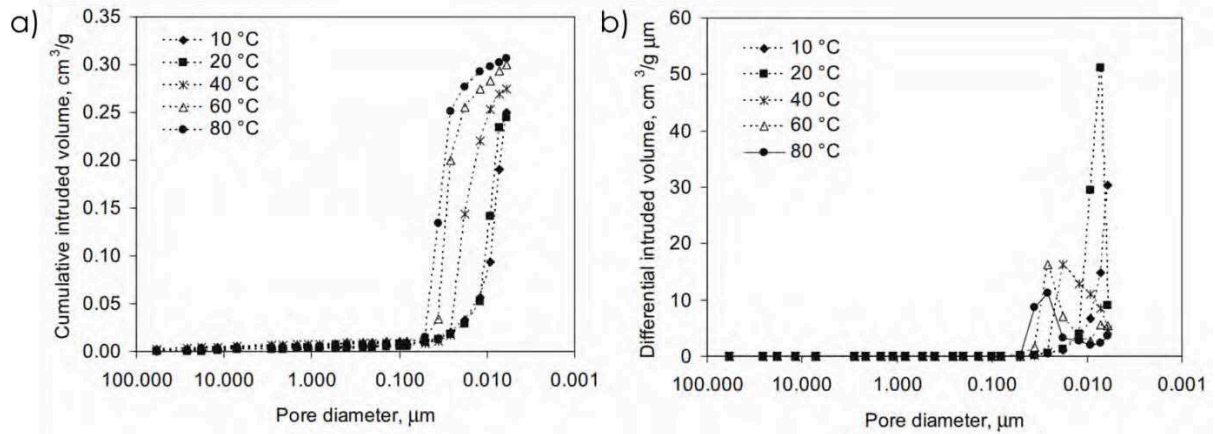
Figure 8. Comparison of pore distribution of geopolymers cured at 10, 20, 40, 60, and 80°C at the age of 28 days. Curing at 40, 60 and 80°C was carried out for an initial 4 h (Rovnaník, 2010).
