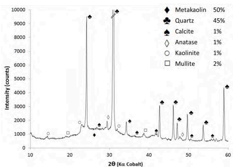
Figure 9. XRD pattern of flash-calcined metakaolin with Rietveld quantification of phases
