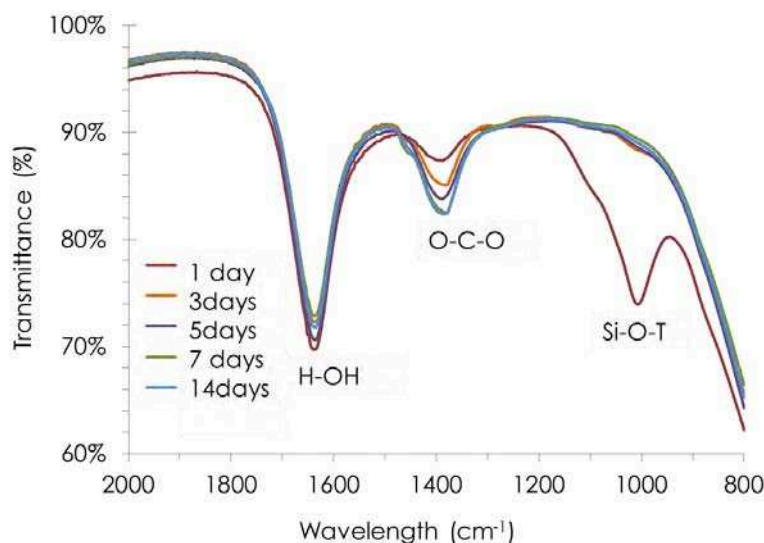
Figure 19. FTIR spectra of pore solutions of geopolymer paste cured at 20^\circ\text{C} , 95% R.H. and atmospheric \text{CO}_2\% , extracted after 1, 3, 5, 7 and 14 days between 2000\text{ cm}^{-1} and 800\text{ cm}^{-1} .
