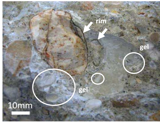
Figure 2. Visual observation of a dam-concrete affected by ASR. Circles show traces of gel in pores and aggregate-prints (Sellier et al., 2009).
