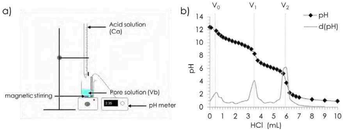
Figure 9. Diagram of a) a pH metric titration and b) theoretical titration curve.
