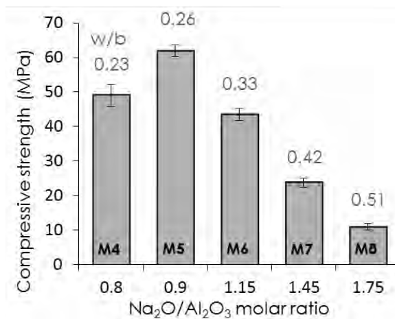
Figure 16. Compressive strength of geopolymer mortars at 7 days with different \text{Na}_2\text{O}/\text{Al}_2\text{O}_3 molar ratios ( \text{SiO}_2/\text{Al}_2\text{O}_3 = 3.6 and \text{Mk}/\text{sand} = 0.33 )
