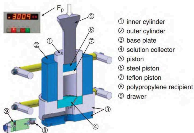
Figure 8. High-pressure device for extracting fluid from porous materials (From Cyr et al. , 2008).
