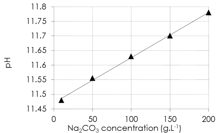
Figure 25. pH versus mass concentration of industrial Na 2 CO 3 solution measured at 20°C.
