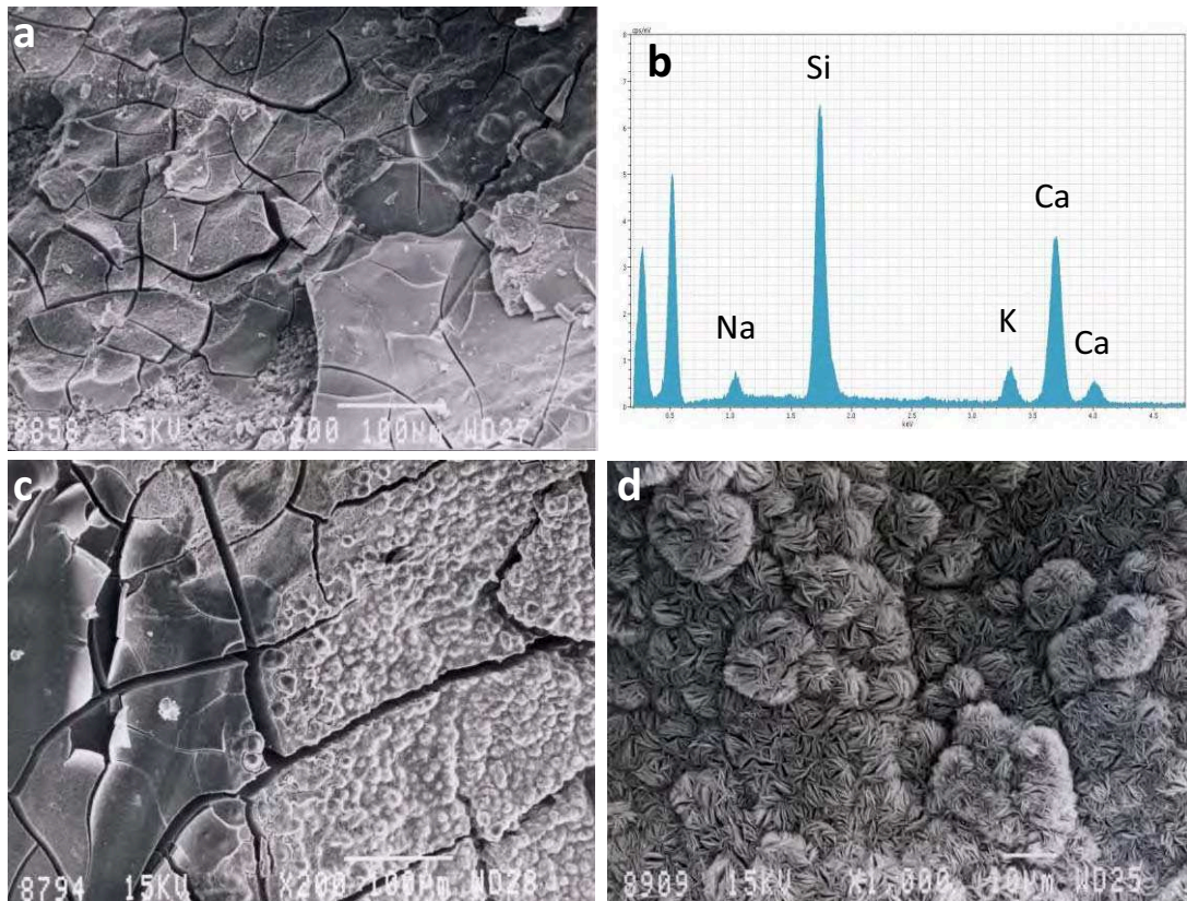
Figure 3. Typical morphologies and composition of ASR-reaction products obtained with scanning electron microscopy (SEM) and energy dispersive X-ray spectrometry (EDX). (a,b,c) SEM micrographs and EDX spectrum of ASR-gel (cracks were provoked by the drying in the microscope chamber), (d) Rosette-type morphology of crystallised gel.
