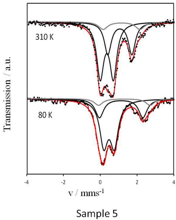
Figure 2.19: Selected ^{57}\text{Fe} Mössbauer spectra (dots) and fit (line) for samples 1-5
