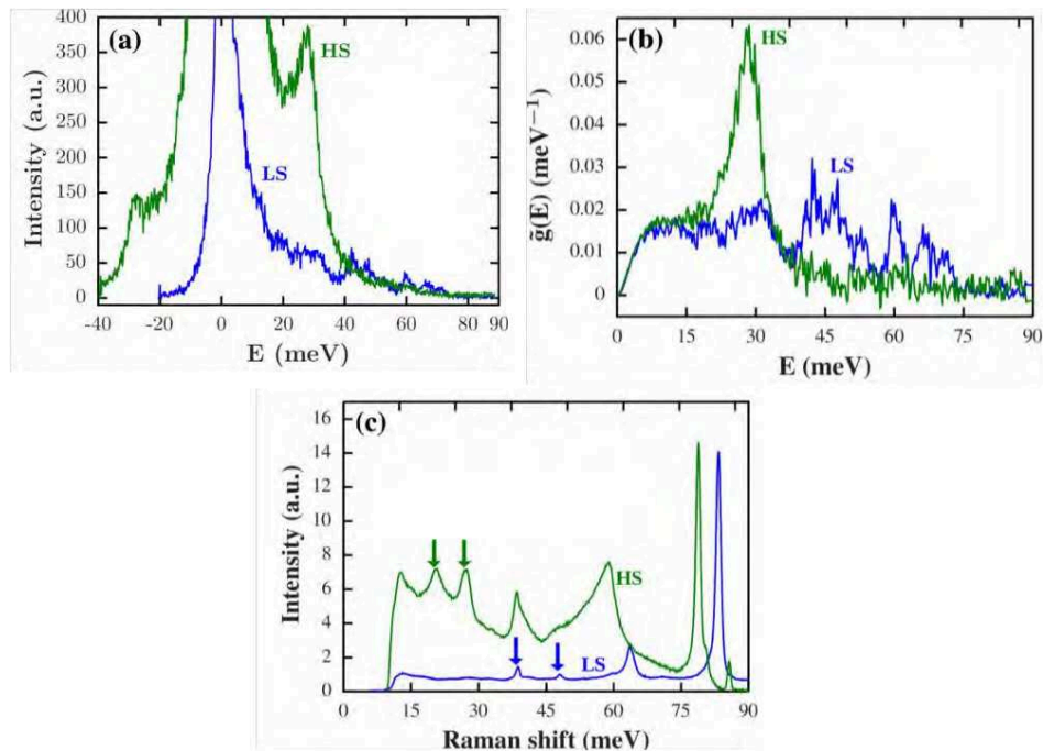
Figure 2.29: (Color online) NIS spectra (a), iron-DOS (b), and Raman spectra (c) of 50-nm [\text{Fe}(\text{pyrazine})\{\text{Ni}(\text{CN})_4\}] nanoparticles in the two spin states. The central peak of (a) is the elastic absorption, while the peaks on the right and on the left are the Stokes (phonon creation) and the anti-Stokes (phonon annihilation) peaks respectively. Their ratio depends on the temperature. Thereby, in the LS state, the anti-Stokes peaks have a very low intensity when compared to the Stokes peak. In (c), the arrows show, from the left to the right, the \nu(\text{FeN}_{\text{cycle}}) and the \nu(\text{FeN}_{\text{NC}}) modes in the two spin states.
