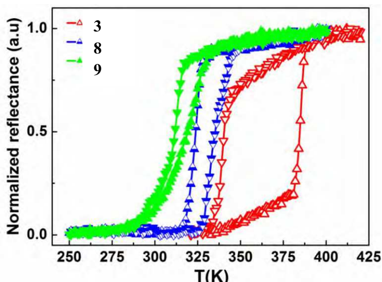
Figure 3.31: Optical reflectance spectra for samples 3, 8 and 9
