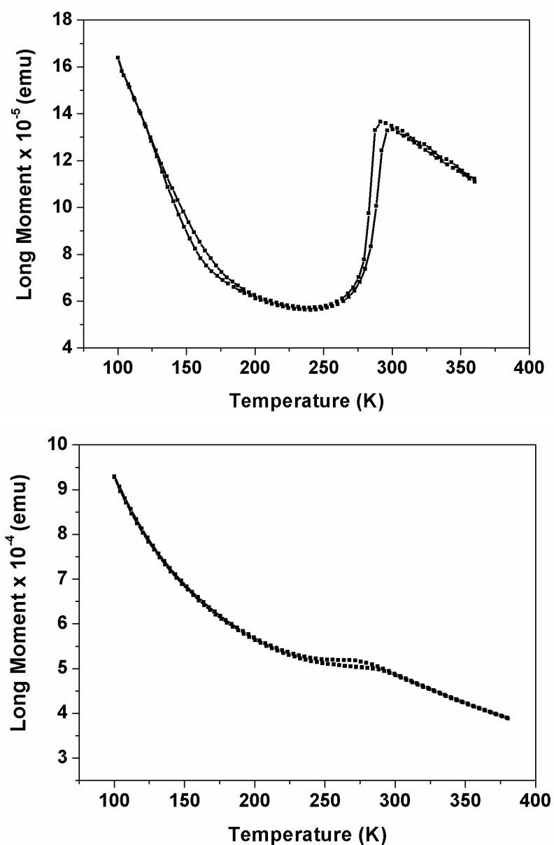
Figure 2.27: Magnetization as a function of the temperature in the heating and cooling modes for dehydrated 50 nm (up) and 2 nm (bottom) [\text{}^{57}\text{Fe}(\text{pyrazine})\{\text{Ni}(\text{CN})_4\}] particles.
