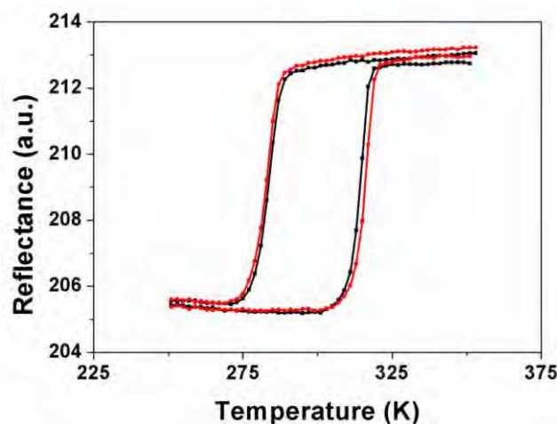
Figure 3.50: Optical reflectivity measurements for testing the hysteresis reproducibility of sample 12 (in black the first cycle and in red the tenth cycle)
