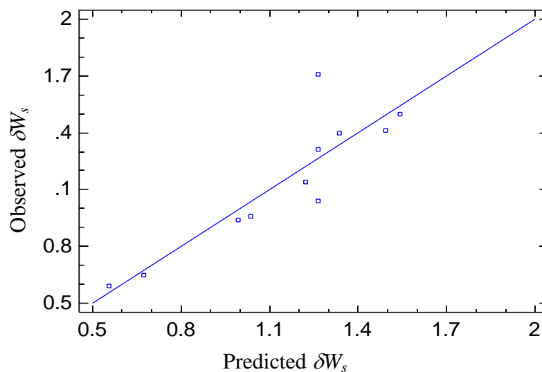
Figure III.19. Comparison between experimental starting accessibility and calculated from the empirical model
