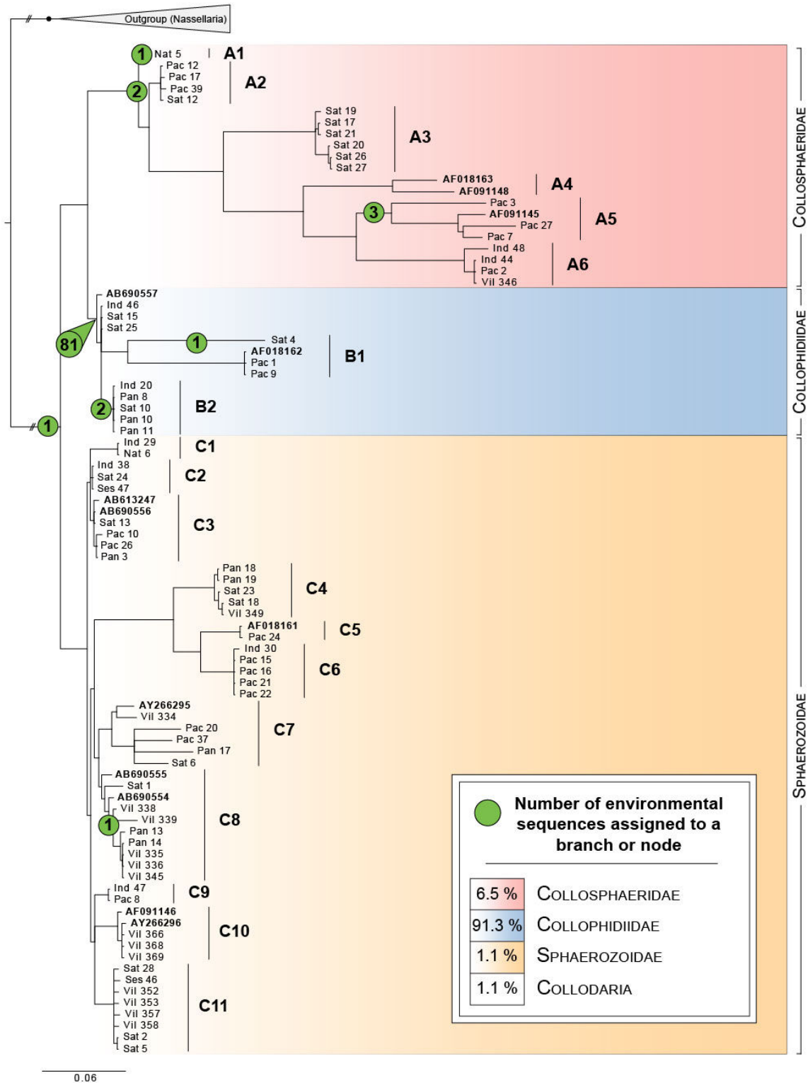
Figure 4. pplacer phylogenetic placement of 92 environmental sequences onto a concatenated phylogenetic tree of Collocladia (complete 18S + partial 28S rRNA genes). Number of sequences affiliated to a clade (node) or sub-clade (branch) is shown inside green circles.
