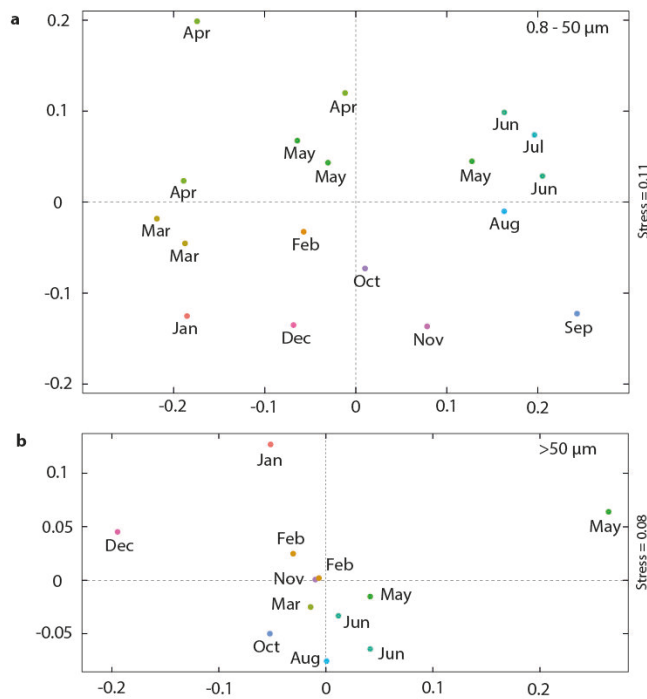
Figure 3 Seasonality of the plankton community. Non-metric multidimensional (NMDS) ordination of plankton community using presence-absence transformed Jaccard similarities between all sampling dates. (a) NMDS ordination of the 0.8 – 50 µm fraction. (b) NMDS ordination of the >50 µm fraction.
