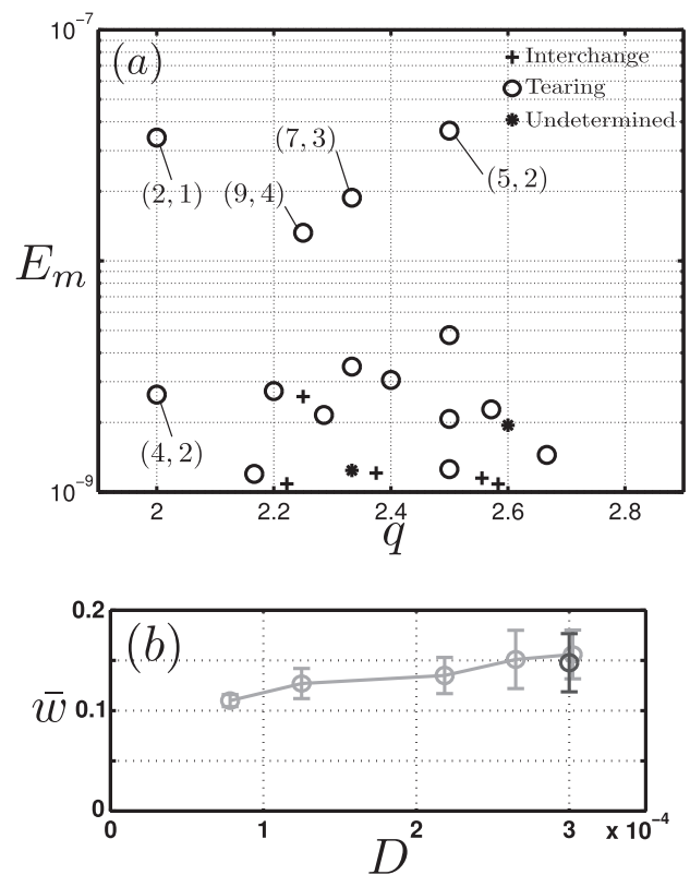
FIG. 4. (a) Magnetic energy spectrum of dominant modes during the asymptotic regime. (b) Impact of the quasi-linear coefficient D on the saturated island width. The error bars correspond to the standard deviation. The grey mark corresponds to a slightly different pressure profile where the right radial band where P_{eq} is constant has been reduced, compared to Fig. 1(a).
