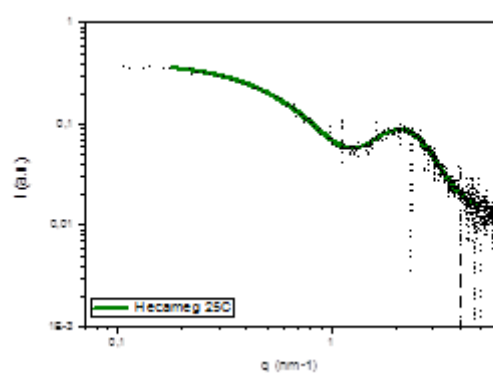
Superposition of experimental and calculated (GIFT) spectra.
