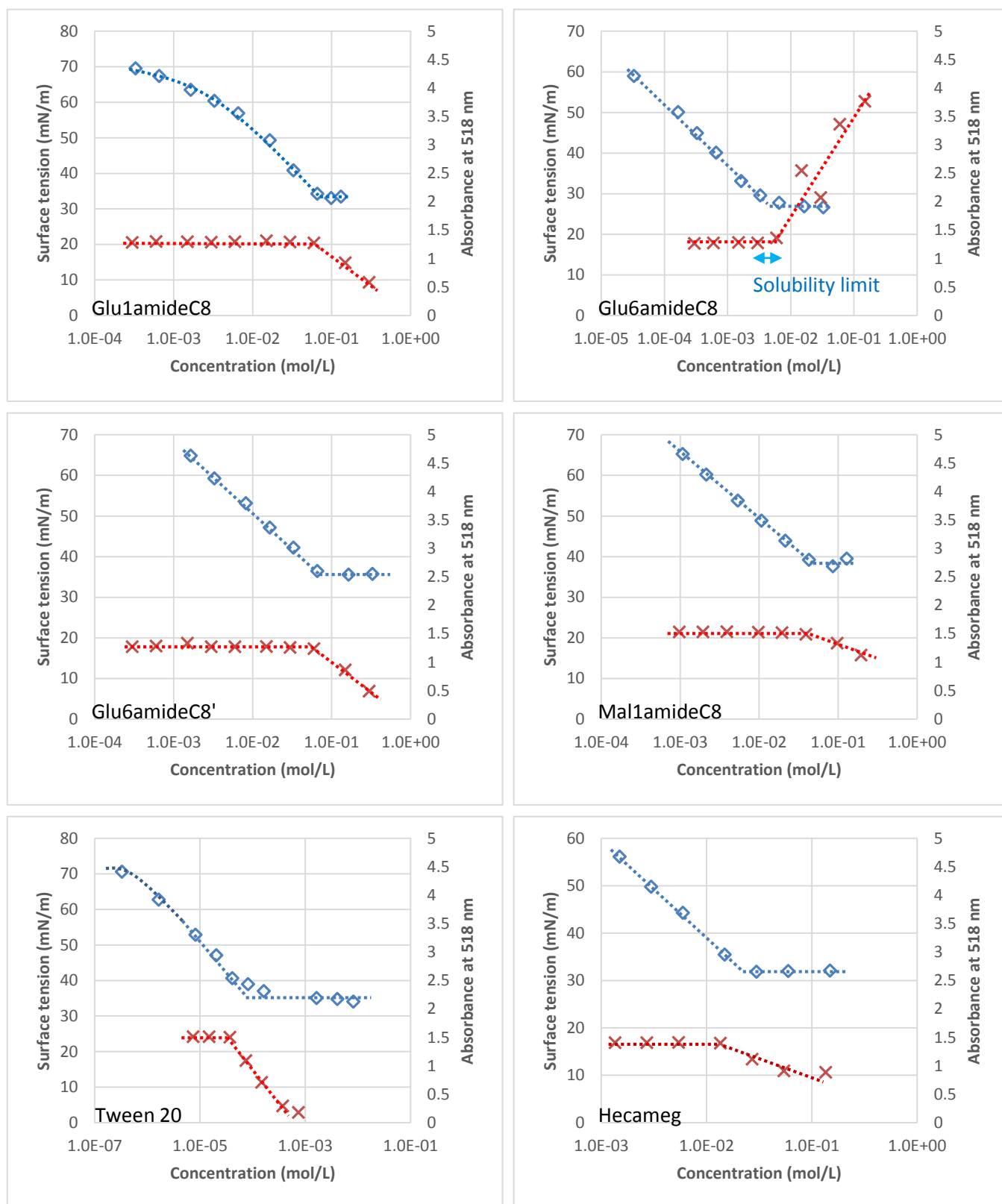
Figure 42: Surface tension ( \diamond ) of surfactant solutions and optical absorbance at 518 nm ( \times ) of Eosin Y-surfactant mixed solutions, concentration of Eosin Y is fixed at 0.17 mmol/L. Solubility limit is determined visually.
