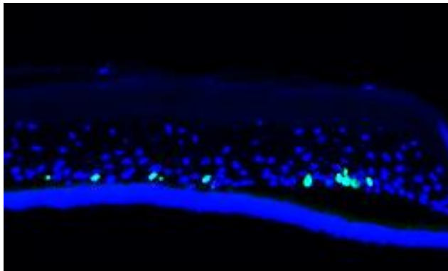
Glu6amideC8' (1000 μg/mL)
