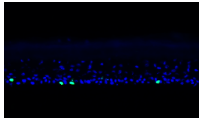
Mal1amideC8 (1000 μg/mL)
