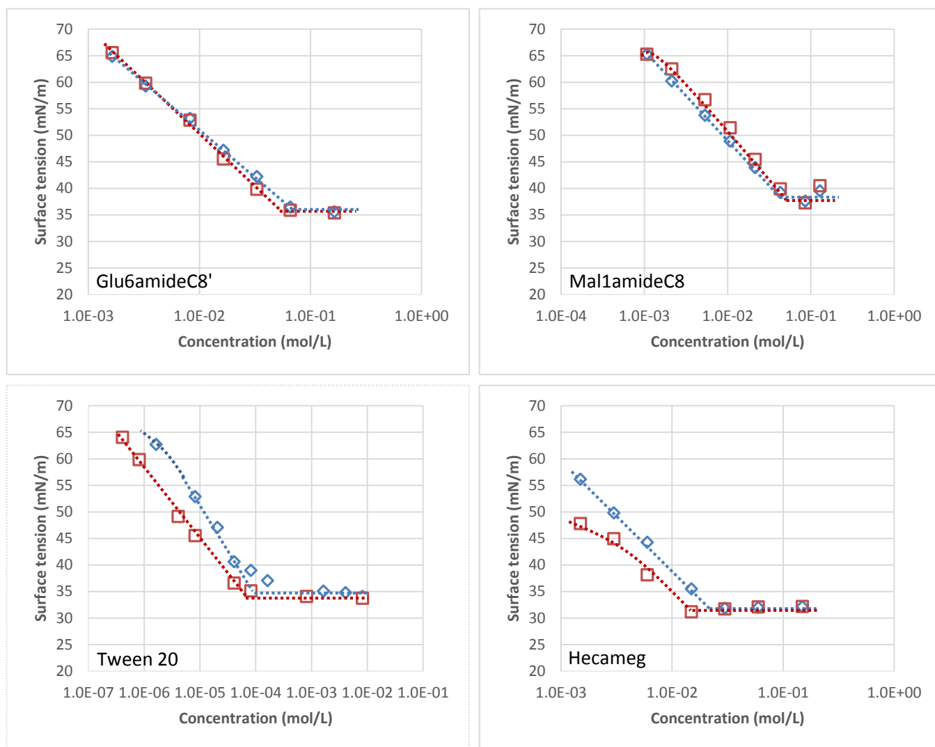
Figure 45: Surface tensions of surfactant in water ( \diamond ) and in complete DMEM (no FBS) ( \square ), T=37^{\circ}\text{C} (part 2).
