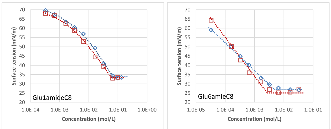
Figure 45: Surface tensions of surfactant in water (◇) and in complete DMEM (no FBS) (□), T=37^{\circ}\text{C} (part 1).
