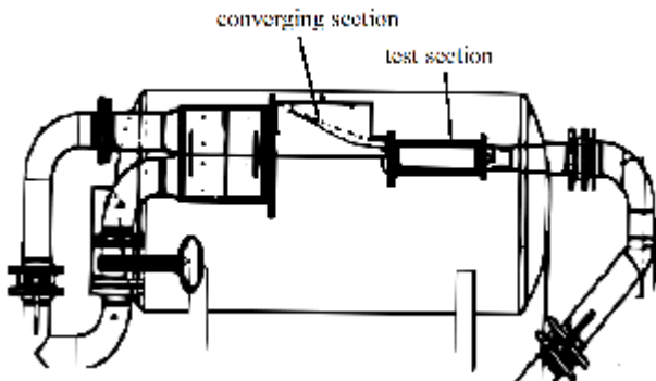
Figure 1: Schematic representation of the tunnel
