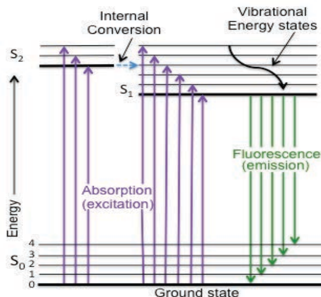
Figure.4. Jablonski diagram typically, S_0 , S_1 , and S_2 are singlet group, first and second electronic states of fluorophores respectively. 0, 1, 2, etc. indicates number of vibrational energy levels shown the principles of the absorption and fluorescence (from Lakowicz, 2006).
