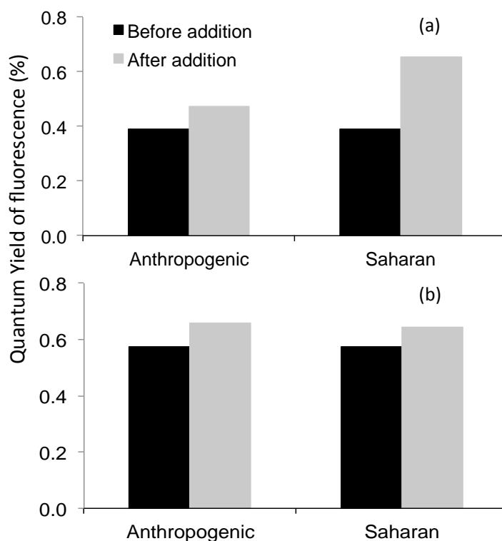
Figure 6. Fluorescence quantum yield at 340 nm [ \Phi(340) ] before-after anthropogenic and Saharan dust addition. (a) BLSp experiment and (b) BCNSp experiment. The [ \Phi(340) ] is expressed in percentage (%).
