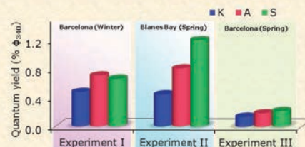
Fig 4. Fluorescence quantum yield at 340 nm after Anthropogenic (A) and Sahara (S) dust addition respectively. Expressed as a percentage (%). K was kept without addition.
