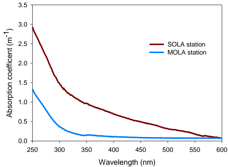
Figure 5. Typical absorption coefficient of surface Mediterranean Sea water. Brown line represents a coastal station (SOLA) and blue line an offshore station (MOLA). Measures for this figure were determined in February 2013.
