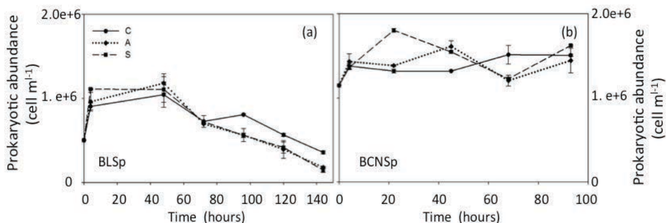
Figure 2. Prokaryotic abundance over time for the three treatments of BLSp (a) and BCNSp (b) experiments. The dust was added at t=4\text{h} in both experiments.
