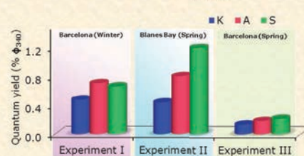
Fig 4. Fluorescence quantum yield at 340 nm after Anthropogenic (A) and Sahara (S) dust addition respectively. Expressed as a percentage (%). K was kept without addition.
