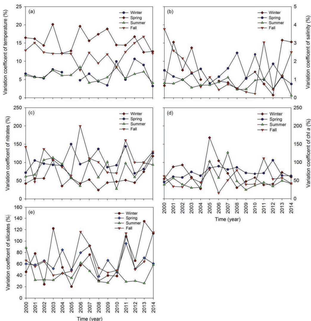
Figure 6. Seasonal coefficient of variation (CV) from 2000 to 2014 in the Bay of Banyuls-sur-mer (SOLA station). (a) Temperature, (b) salinity, (c) nitrates (d) chl a, and e) silicates. The CV is expressed in percentage (%).
