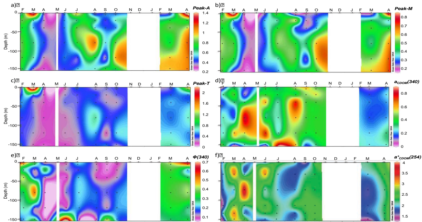
Figure 7. Temporal variability from February 2013 to April 2014. a) Peak-A, b) Peak-M, c) Peak-T. All peaks are expressed in quinine sulfate units (QSU), d) a_{\text{CDOM}(340)} in \text{m}^{-1} , e) \Phi(340) in percentage (%), and f) a^*_{\text{CDOM}(254)} in \text{m}^2 \text{g}^{-1} \text{C}^{-1} . The dots represent the sampling points.
