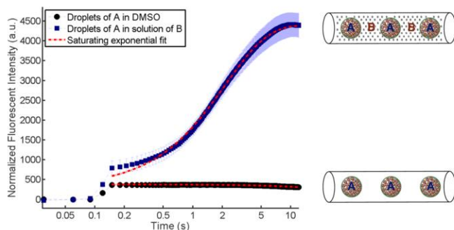
Figure 5. Fluorescence increase after the ultrasound release at t = 100 ms. Comparison between control experiment (droplets of 3-azido-7-hydroxycoumarin A in DMSO, black curve) and reaction (droplets of 3-azido-7-hydroxycoumarin A in a solution of TMDIBO B in DMSO, 0.3% w/v, blue curve). The reaction rate is well described by a saturating exponential fit with a time constant of 2.2 s ( R^2 = 0.99 ).
