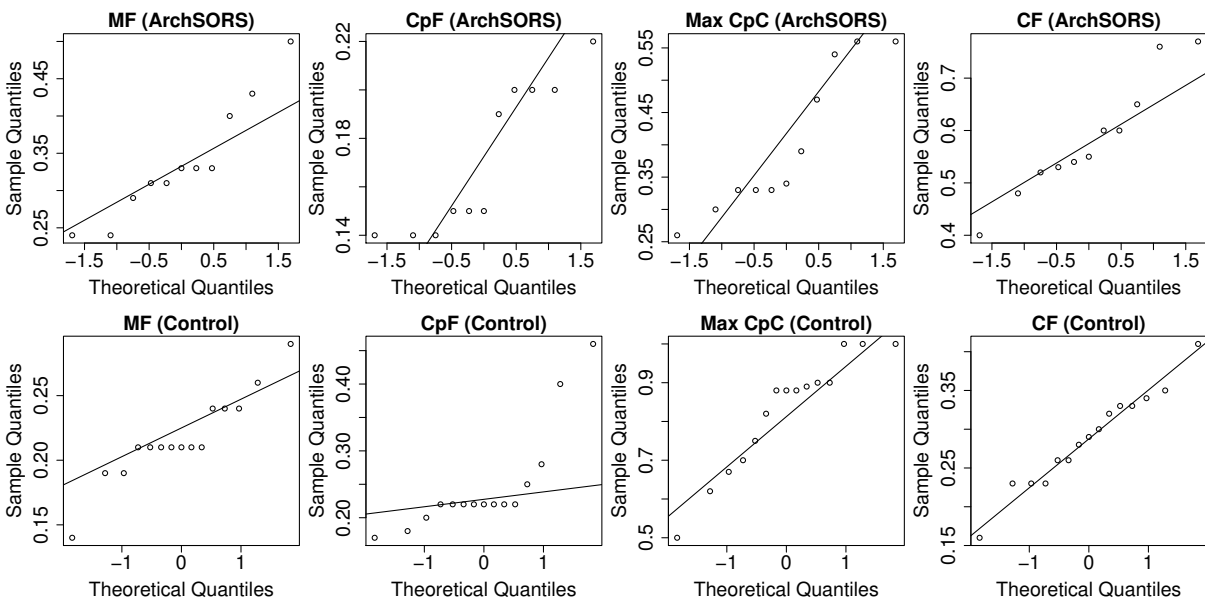
Figure 4.16: Normal probability plot of the results
