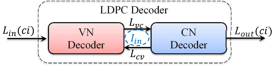
Figure 1.10: Block diagram of LDPC decoder.
