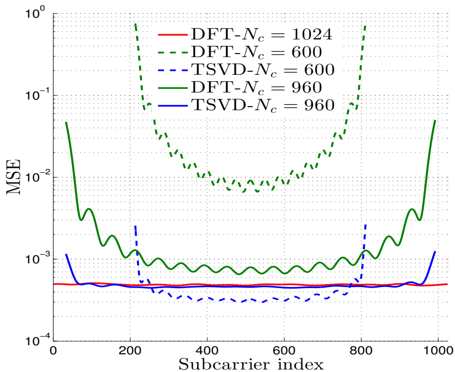
Figure 5.8: MSE in function of sub-carriers index for classical DFT and TSVD based channel estimation with N = 1024 , N_c = 1024, 960, 600 at SNR = 20 dB, 4-QAM.
