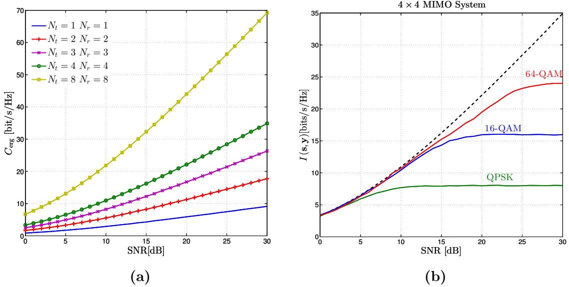
Figure 1.14: Ergodic channel capacity of MIMO system with different number of transmit and receive antennas (a) and average Mutual information according to the SNR for 4 \times 4 (b) MIMO system using 3 constellations.
