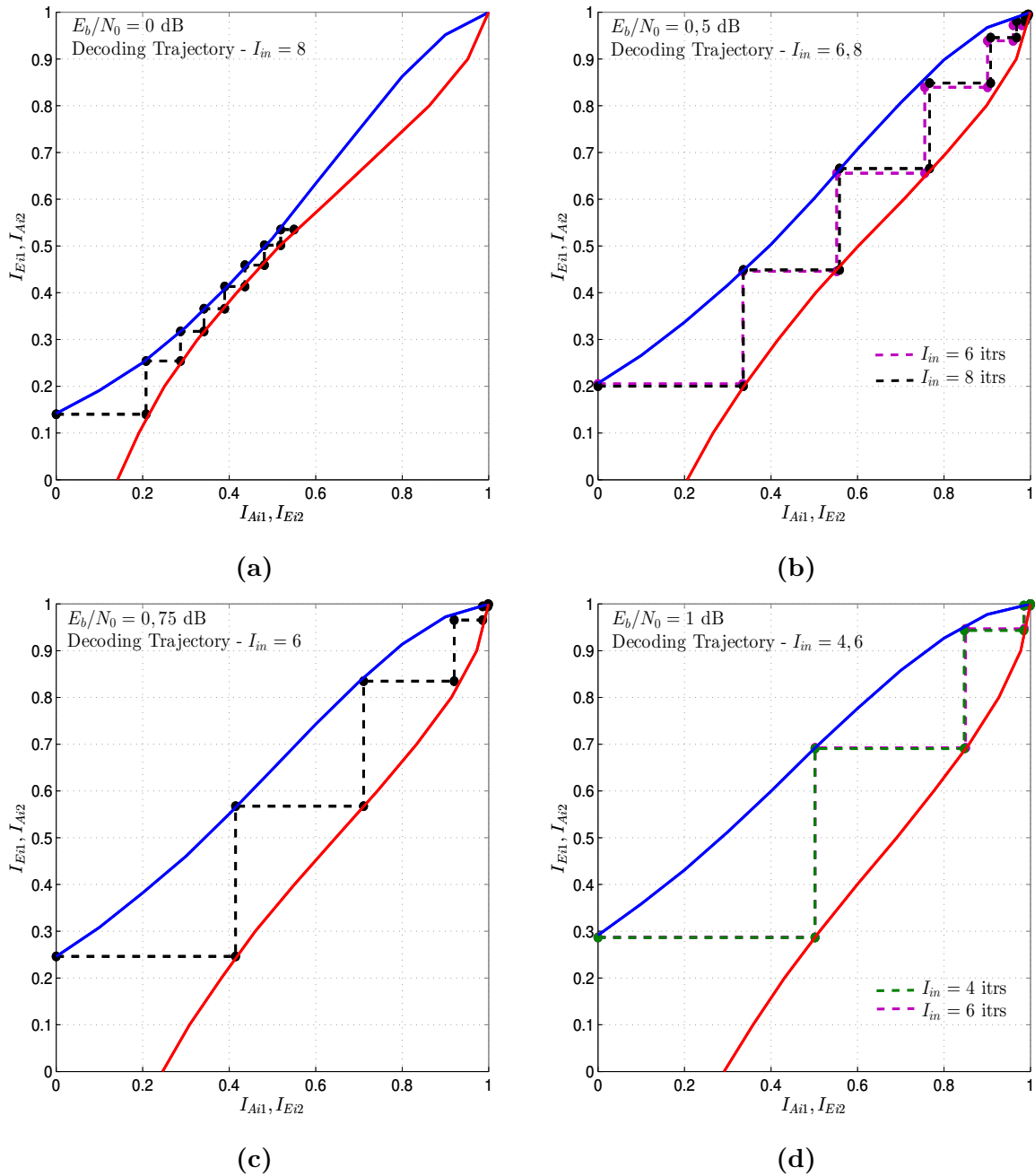
Figure 3.11: Iterative decoding trajectory of LTE turbo decoder, R_c = 1/2 , K_b = 2,048 in AWGN channel with BPSK modulation for different E_b/N_0 values.
