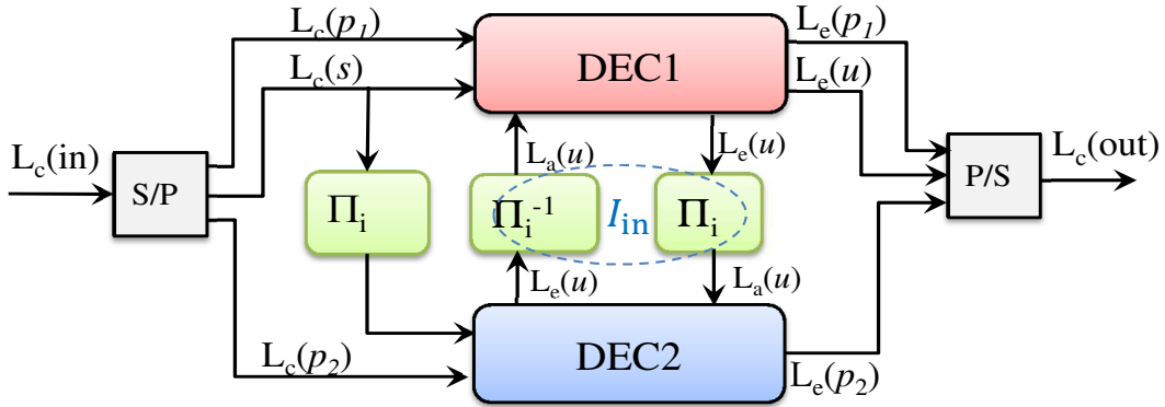
Figure 1.6: Turbo decoder.
