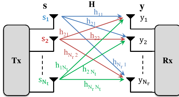
Figure 1.16: MIMO channel.
