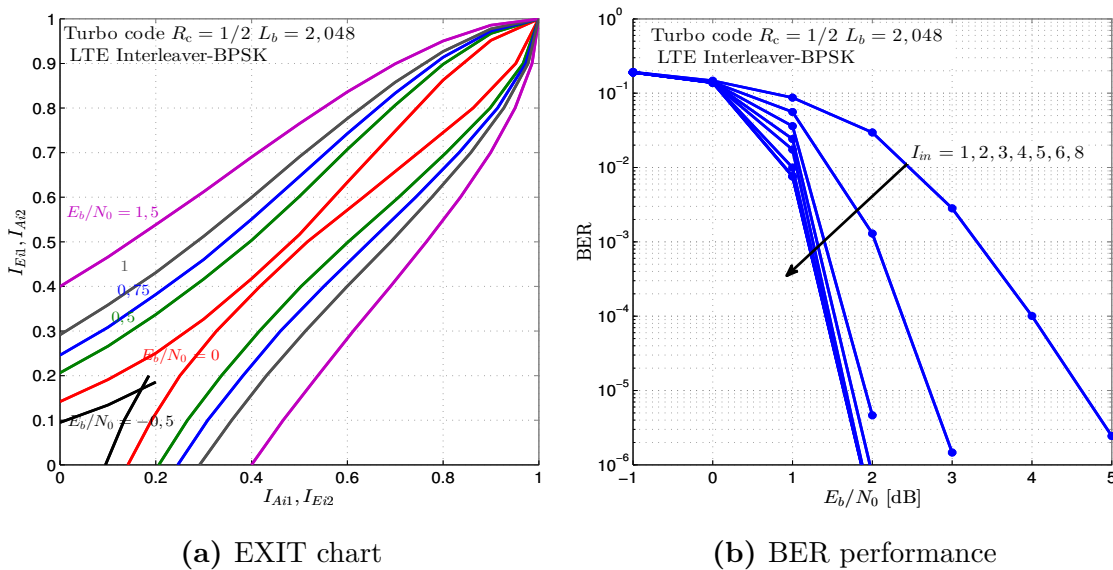
Figure 3.10: EXIT chart of the two component decoders of LTE turbo decoder (a), and BER performance (b), R_c = 1/2 , K_b = 2,048 in AWGN channel with BPSK modulation for different E_b/N_0 values.
