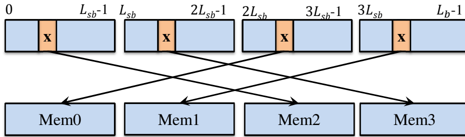
Figure 1.7: QPP interleaver propriety.
