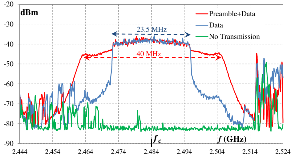
Figure 5.23: Frequency spectrum.
