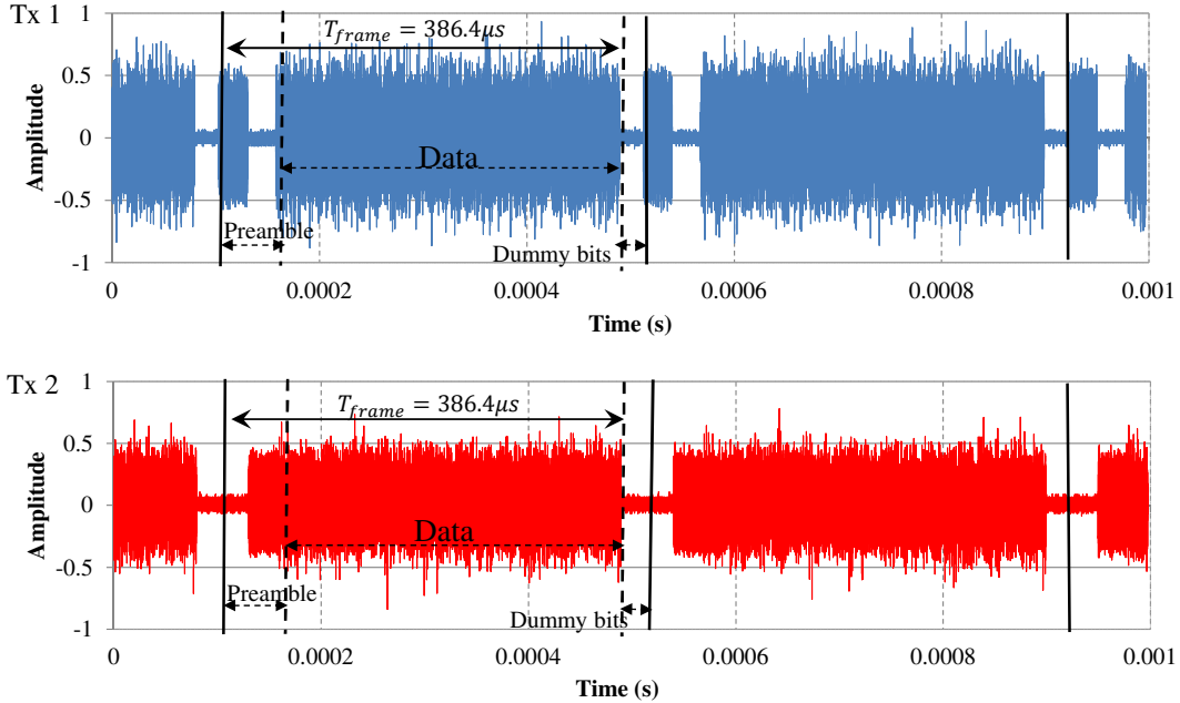
Figure 5.22: Transmitted signals.
