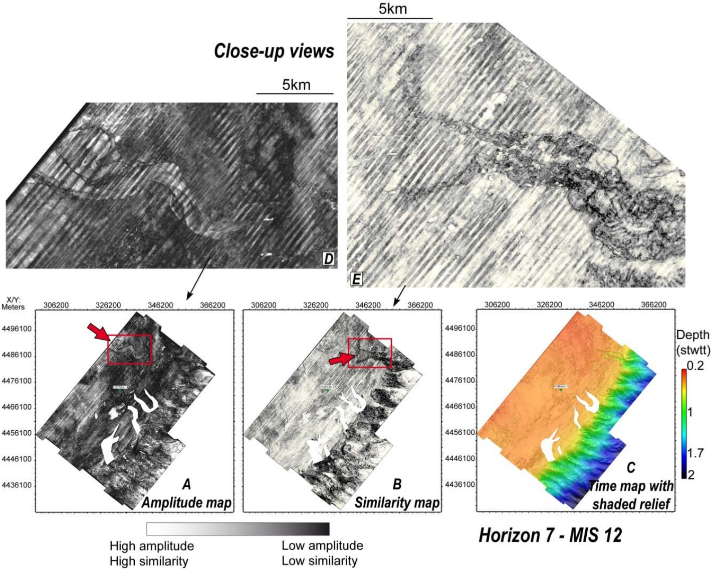
Figure 10: Maps for Horizon 7. A and B (shades of gray) display the amplitude and similarity attributes, whereas C shows the structure time map with shaded relief. D is a close-up view extracted from the amplitude
