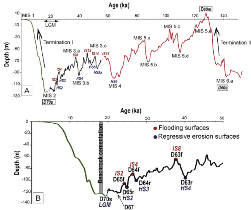
Fig. 8. Correspondence between seismic surfaces described in this study, sea-level and climatic events during the last 150 kyr. The composite sea-level curve is based on Khripounoff et al., 2012 (red; from 150 to \approx 60 kyr), Arz et al., 2007 (black; from \approx 60 to \approx 20 kyr) and Lambeck et al., 2014 (green; for the last \approx 20 kyr) in order to better represent the variability of high-frequency sea-level changes and their link with seismic surfaces. A: Composite sea-level curve with climatic event terminologies according to Railsback et al., 2015 (for MIS and Terminations) and to Sierro et al., 2009 (for Heinrich stadials (HS) and Interstadials (IS)). In addition, sequence boundaries (D60s and D70s) and the maximum flooding surface (D60m) are presented. B: Focus on the last 50 kyr with the regressive erosion surfaces corresponding to Heinrich stadials (low sea-level) and the flooding surfaces in phase with the following Interstadial (higher sea-level). The gray rectangle highlights the period of beachrock cementation.
