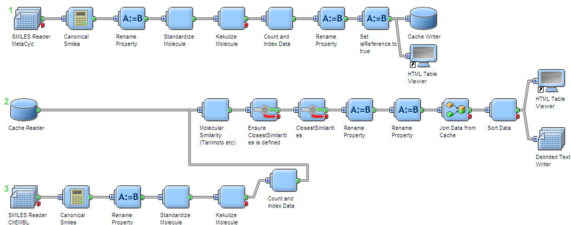
Figure 10. Pipeline pilot protocol for natural products known target search.
