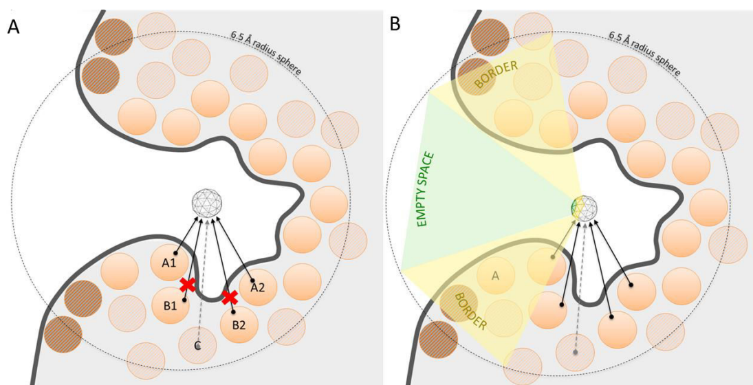
Figure 8. Identification of binding site mouth.
