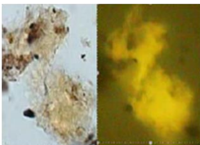
Figure 25: Photographs of palynofacies fractions used for OM characterization along the core. From Graz et al., 2010 and Boussafir et al., 2012.
