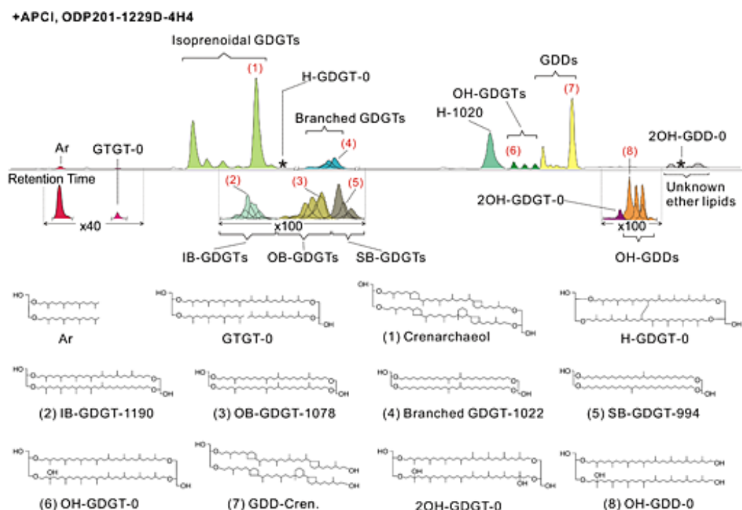
Figure 12: LC/APCI/MS chromatogram showing the distribution of glycerol ether lipids in sample ODP201-1229D-4H4, Peru Margin (Liu et al. 2012c) and their corresponding structures. From Liu et al. (2012c).
