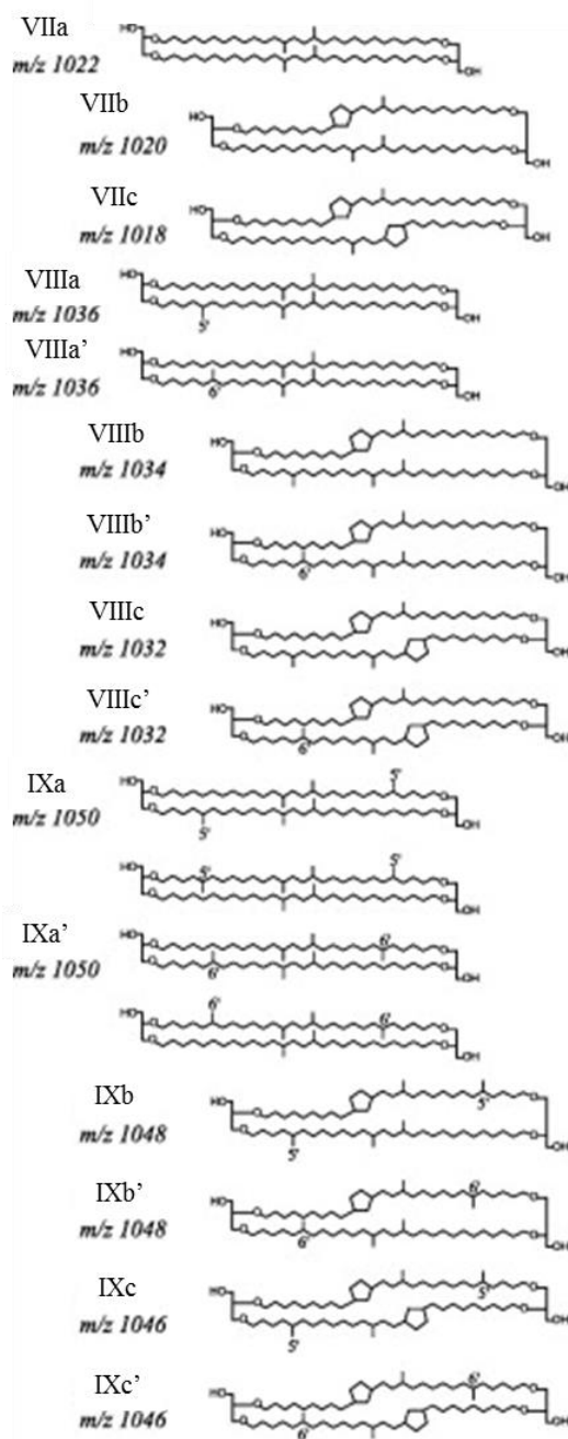
Figure 13: Chemical structures of br GDGTs including those containing one or two methyl groups at the \alpha and/or \omega -6 position (indicated with a prime symbol). Note that the numerotation is different from the rest of the thesis (GDGTs I are GDGTs IX series, II are the series VIII and III correspond to GDGTs VII). From (De Jonge et al., 2014).
