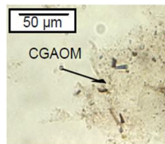
Figure 25: Photographs of palynofacies fractions used for OM characterization along the core. From Graz et al., 2010 and Boussafir et al., 2012.
