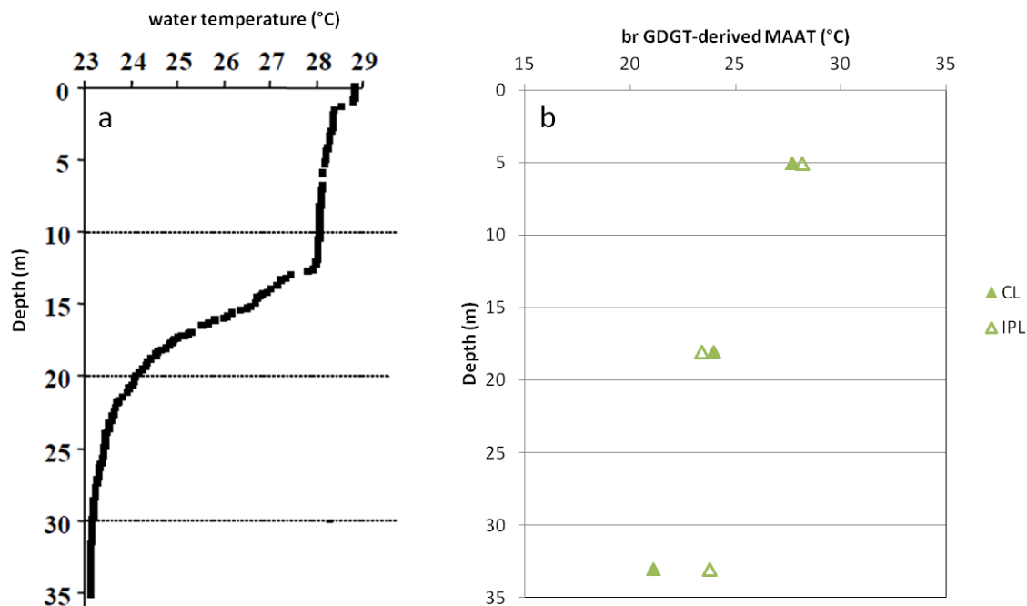
Figure 49: Comparison between (a) Lake Masoko thermocline and (b) br GDGT-derived MAAT (based on East African lacustrine calibration; Loomis et al., 2012) for the POM samples collected at 5, 18 and 33 m depth. MAAT was estimated from CL (solid symbols) and IPL (open symbols) br GDGTs
