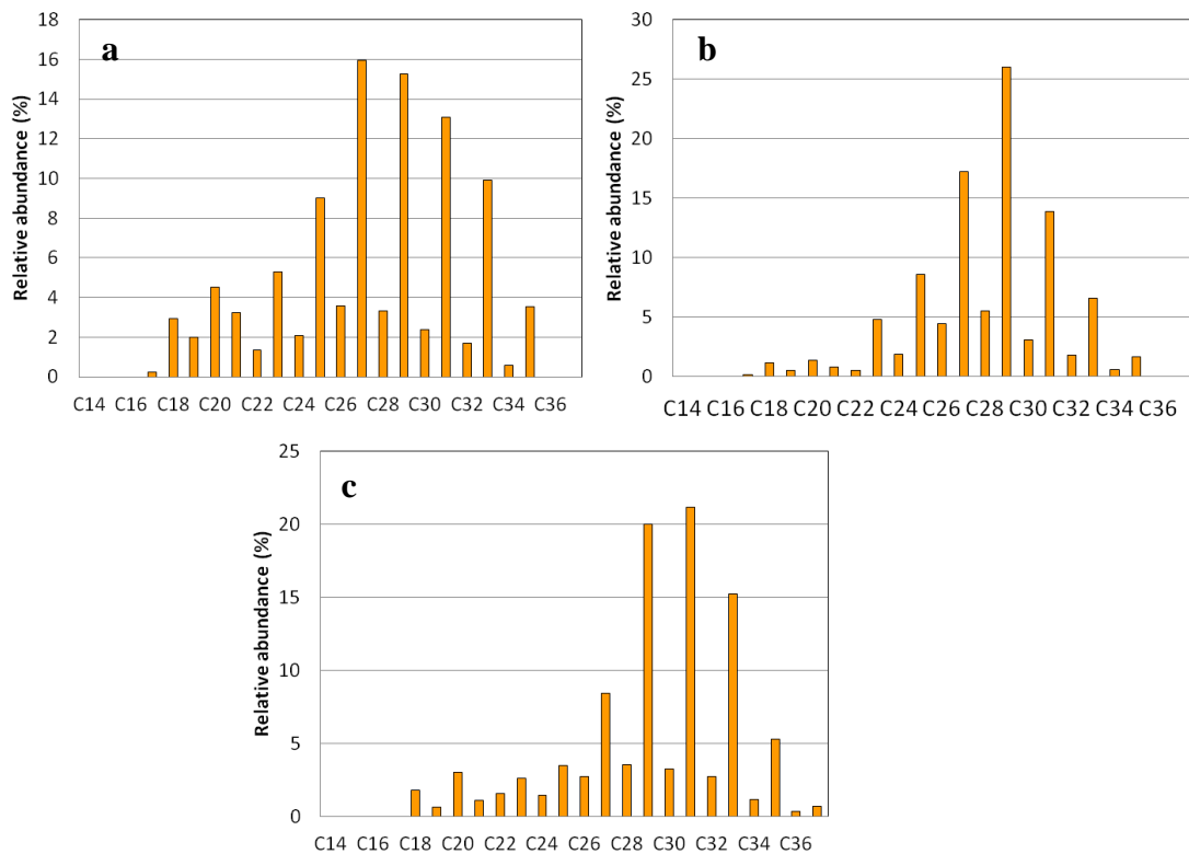
Figure 53: typical distributions of n -alkanes along the core: (a) at 6.5 cm depth, (b) at 176 cm depth and (c) at 256 cm depth.
