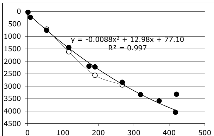
Figure 38: model age based on 14 ^{14}\text{C} AMS dates of bulk OM (black points). ^{14}\text{C} AMS dates of wood remains (white dots) are also represented.
