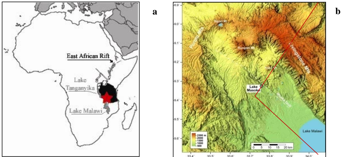
Figure 16: (a) Location map of the Rungwe Volcanic Province (RVP), at the extremity of the western branch of the East African Rift System (after Delalande, 2008). (b) Digital elevation model of the RVP, (after Garcin, 2006).
