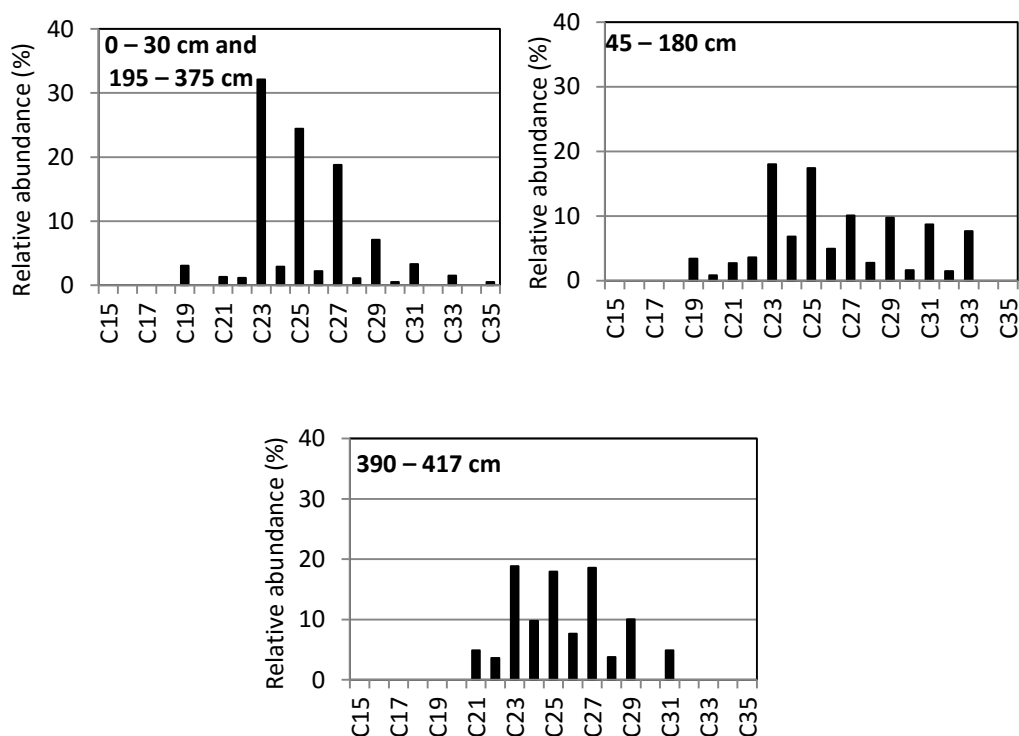
Figure 43: Typical n -alkane distributions observed along the core. The 3 profiles correspond to those described in the text.
