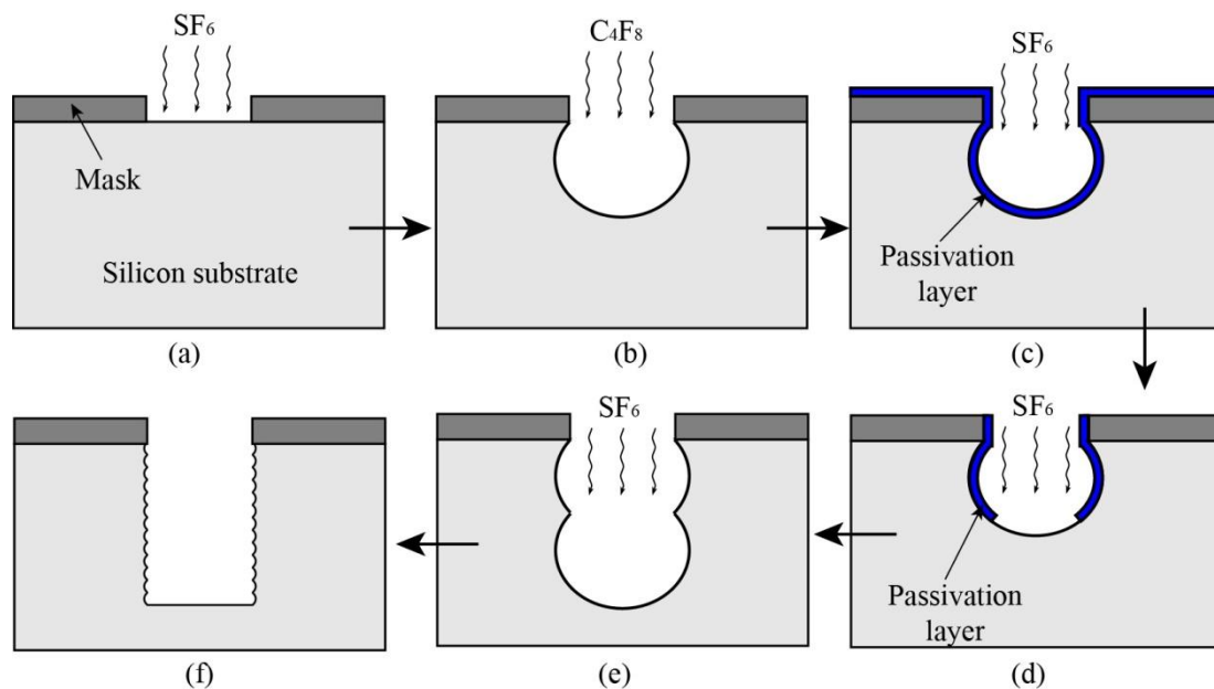
Figure 2 - 17. Bosch etch process: (a) First etch cycle with SF 6 ; (b) First passivation with C 4 F 8 ; (c) (d) and (e) Second etch cycle; (f) Vertical side wall with multiple etch-passivation cycles.
