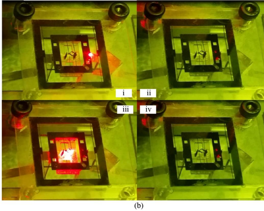
Figure 3 - 22. (a) Two cycles of the actuation of silicon quadristable micro-actuator; (b) Photos of the quadristable micro-actuator in one actuation cycle: i - ii actuation of outer row; iii - iv actuation of inner row.
