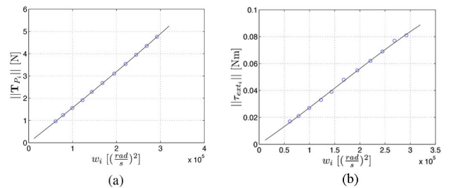
Fig. 9. (a) and (b) Dots: measured values of the thrust \|\mathbf{T}_{P_i}\| and torque \|\boldsymbol{\tau}_{ext_i}\| versus the signed squared spinning velocity w_i . Black lines: identified polynomial model (25) and (26).
