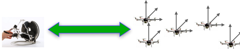
FIGURE V.4: A single human operator acting on a device with 3–6 free DOFs must control a slave side made of N robots with \sim 6N DOFs. This large redundancy must be resolved autonomously by the slave side for not overloading the human operator.
