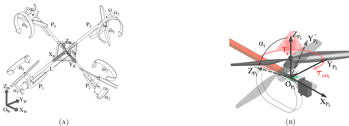
FIGURE VII.2: Left: schematic view of the quadrotor considered in this paper. The overall center of mass is assumed to be in the body frame center. The symbol L represents the length of all propeller arms, \omega_i , i = 1 \dots 4 , the propeller rotation speed and \alpha_i , i = 1 \dots 4 , the orientation of the propeller group. Right: i -th tilting arm visualizing the body frame \mathcal{F}_{P_i} , the associated propeller thrust T_i , torque \tau_{ext_i} and the propeller tilt angle \alpha_i
