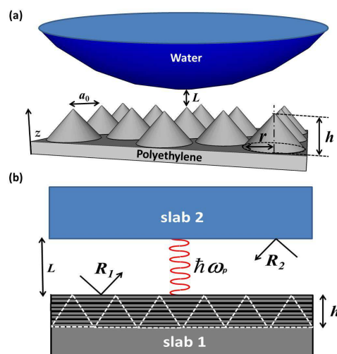
FIG. 1. (Color online). (a) Corrugated surface separated by a distance L from a water droplet. The surface of the droplet can be considered as flat at the scale of corrugation. (b) Approximation of the two-body system. R_1 and R_2 are the reflection coefficients of the effective multilayer (slab 1) and of the water droplet (slab 2), respectively. Virtual photons \hbar\omega_p exchanged between the two slabs are pictured in red.
