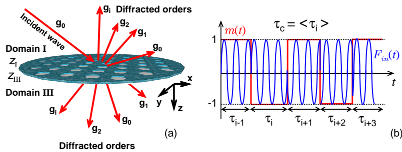
FIG. 1: (a) Sketch of a light trapping diffracting structure ( Z_I < z < Z_{III} ) with many diffraction orders. Domains I and III are respectively the incident and emergence media. (b) Model of field amplitude F_{in}(t) for the incoherent monochromatic incident light. m(t) is the corresponding modulation which characterizes the random phase switching at different times \tau_i . \tau_c is the coherence time, equal to the average value \langle \tau_i \rangle .
