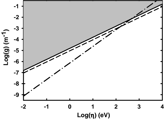
Figure 2: Solid line: Experimental limits for the coupling constant g against the confinement energy \eta h . Dashed-dotted line: expected limits for a yearly experiment. Dashed line: expected limits for a resonant experiment (laser-induced). Grey domain is excluded.
