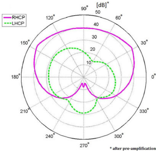
Fig. 13. Leica AR10 antenna gain pattern for RHCP and LHCP polarization.
