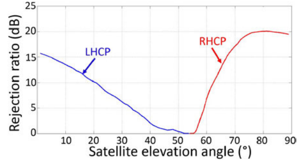
Fig. 14. RHCP and LHCP rejection ratio of the Leica AR10 antenna used in this study.
