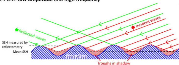
Fig. 13. Sea State Bias (SSB) induced by waves trough shadowing when measuring off-nadir at low elevation angles with high amplitude and frequency of waves (a) or low amplitude but high frequency of waves (c). Signal convergence in troughs with low amplitude and frequency of waves (b). SSH: Sea Surface Height.
