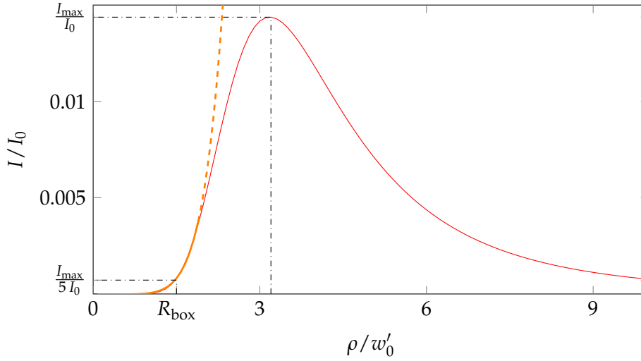
Figure 6.2.: In red solid line, intensity distribution for a phase plate with a 12\pi phase winding in paraxial approximation. This beam profile is extracted from exact integration of Eq. 6.5 for a Gaussian beam. I_0 is the intensity in the center of a Gaussian beam with the same total power P . In orange is presented the power law fit of the trap edges using Eq. 6.4. The fit gives \beta = 6.55 \pm 0.07 .
