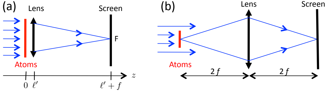
Figure D.1.: Two possible setups for measuring the absorption of an incident probe beam by a slab of atoms using a lens of focal f . a) Global probe. b) Local probe.
