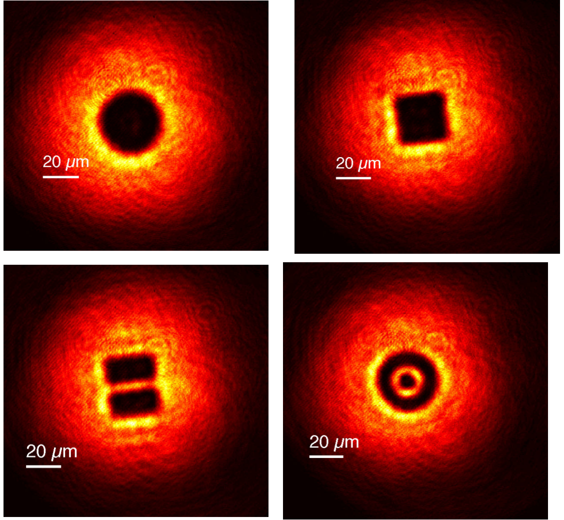
Figure 6.8.: Example of the possible changes in shape or in size of the box-trap. We show the intensity profile for: a disk (upper left) of larger radius than previously ( R_{\text{box}} = 15 \mu\text{m} instead of R_{\text{box}} = 12 \mu\text{m} ), a square (upper right), two rectangles (we can also produce a unique rectangle of the same size – lower left), a target that is made of a central disk circled by an annulus (lower right).
