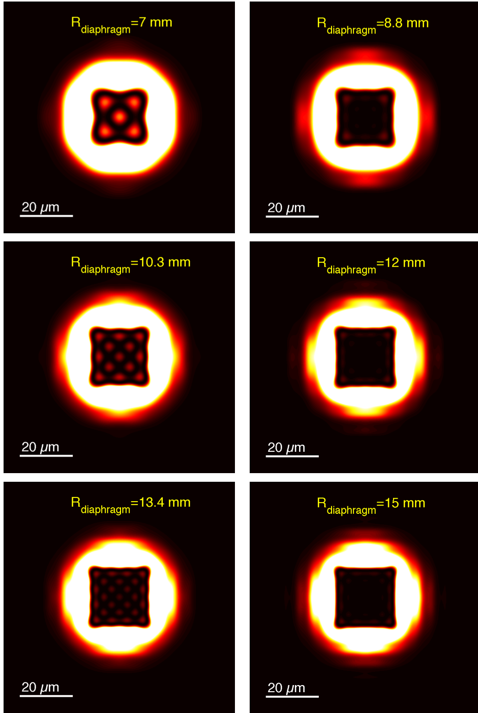
Figure G.5.: Examples of simulated intensity profiles for a square-shaped mask when varying R_{\text{diaphr}} . We simulate the intensity profile using the procedure described in G.1.1 . We use R_{\text{diaphr}} = 7, 8.8, 10.3, 12, 13.4 and 15 mm which correspond to the detected extrema (alternatively maxima and minima) of \delta I_{\text{std}} . We rescale the intensity to 15% of the barrier to enhance the trap bottom defects.
