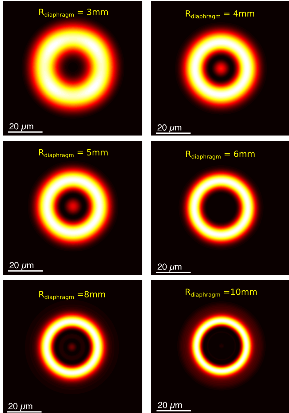
Figure G.2.: Examples of simulated intensity profiles with various diaphragm apertures R_{\text{diaphr}} = 3, 4, 5, 6, 8 and 10\text{ mm} . We use a initially disk shaped mask of radius R_{\text{mask}} = 40\ \mu\text{m} . It is imaged via a 1 to 1 telescope made up with two lenses of focal f = 500\text{ mm} .
