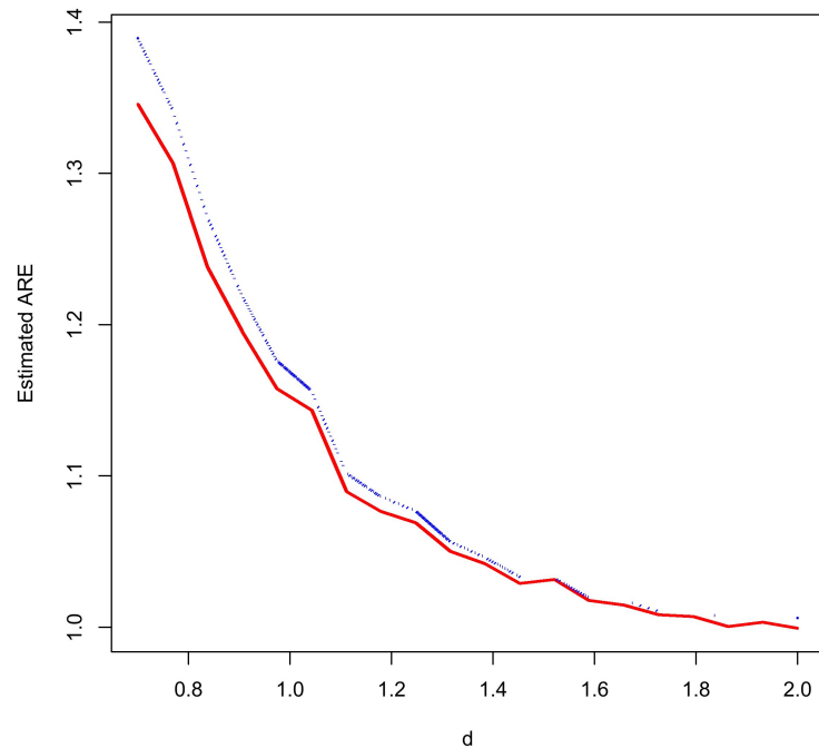
Figure 2.3 – As figure 2.2, but the ARE's are estimated from the residuals of a GARCH(1,1) with innovations \eta_t \sim \Gamma(1, 2, d) .
