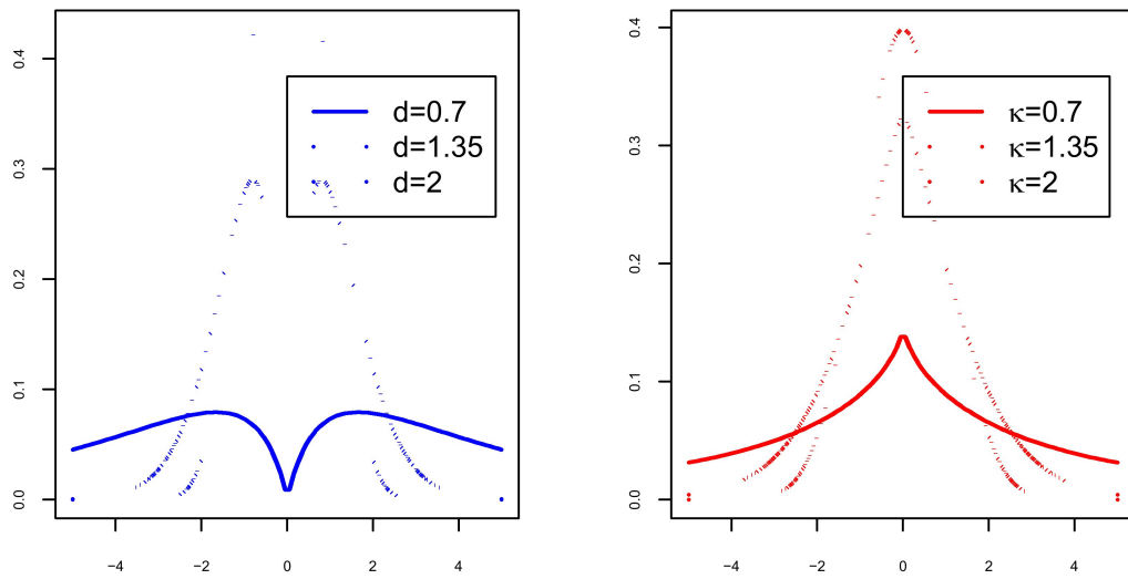
Figure 2.1 – Density \Gamma(1, 2, d) for d = 0.7 , d = 1.35 and d = 2 (left panel) and density GED(\kappa) for \kappa = 0.7 , \kappa = 1.35 and \kappa = 2 (right panel). The asymptotic distribution of the generalized QMLE based on \Gamma(b, p, d) is the same as that based on GED(\kappa) when \kappa = d .
